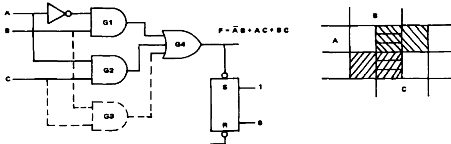
Figure 4.3.1-3. Redundant design can prevent a glitch.
