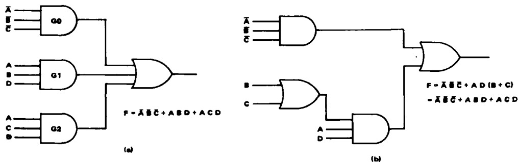
Figure 4.3.1-2. Provide test access by redesign to avoid fault redundancy.
