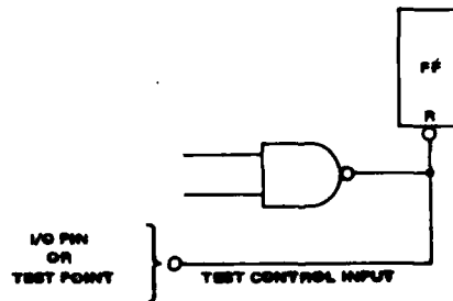
Figure 4.3.1-6. Wired OR for test control input.
