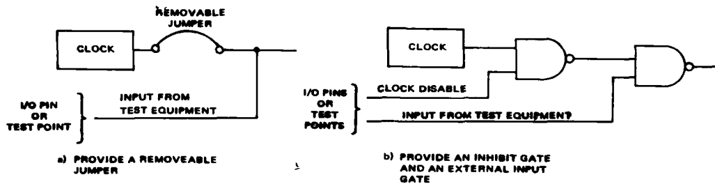
Figure 4.3.1-7. Techniques for disabling on-board clocks to allow off-board clocking.
