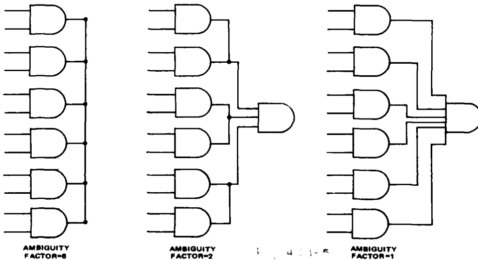
Figure 4.3.1-5. Redesign gate networks to reduce fault ambiguity factor.
