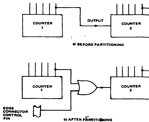
Figure 5.3-1. Provide gates to partition counter chains.
