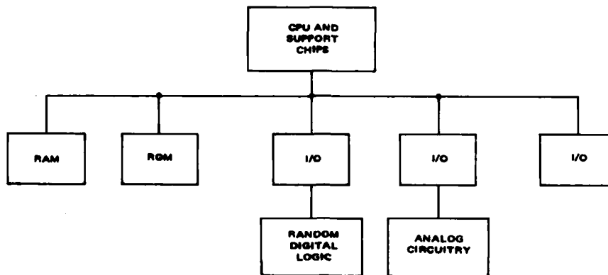
Figure 4.3.2-1. Structure Diagram of Microprocessor Based System
