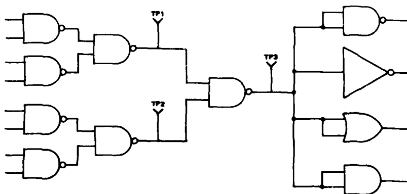
Figure 4.3.3-1. High Fan-Out/High Fan-In Test Point Placement
