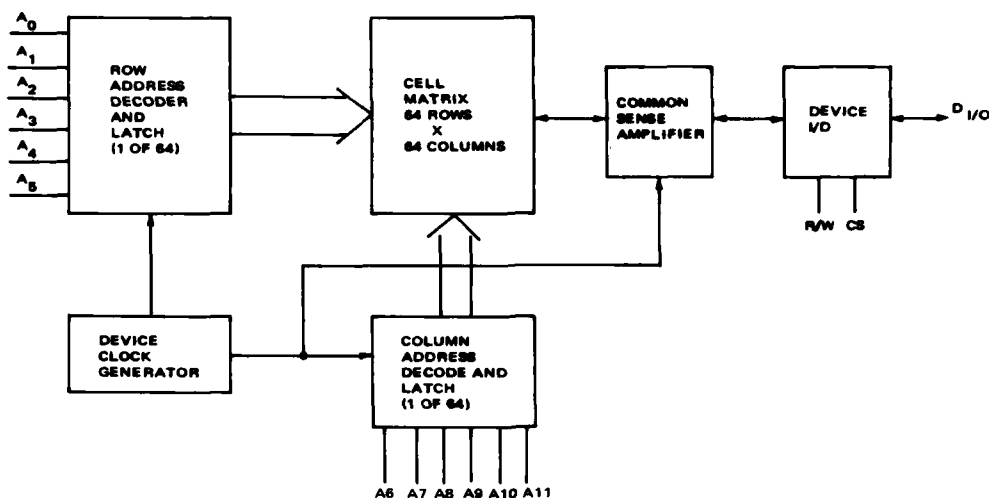
Figure 4.3.5-2. Block Diagram of 4Kx1 MOX Dynamic RAM
