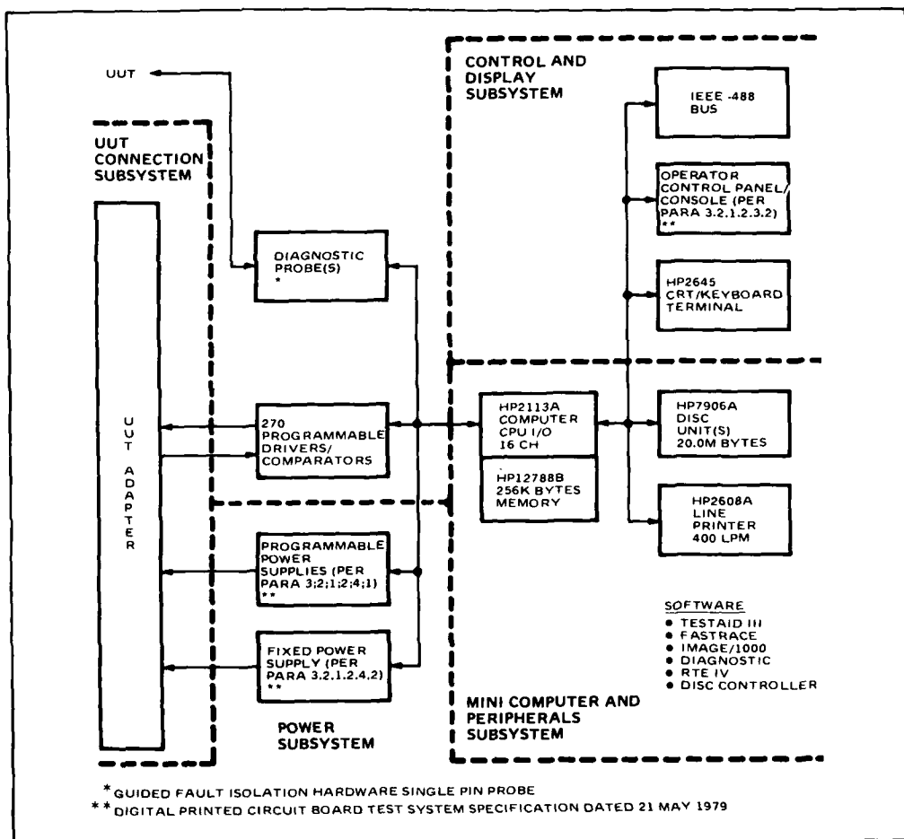
DTS-70 Test System Hardware Block Diagram and Software Packages. The system is capable of expansion to support 6 time sharing terminals.
