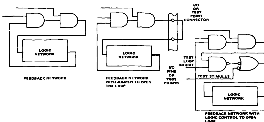
Figure 4.3.1-13. Break feedback paths.
