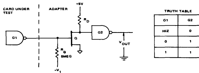
Figure 4.3.3-2. Tri-State High Impedance State Detector
