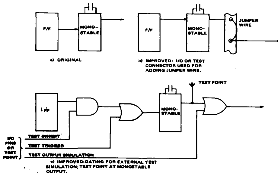
Figure 4.3.1-12. Electrical disconnection of monostables with external simulation path provided.
