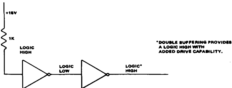
Figure 4.3.1-1. Isolate logic highs and lows from power buses.
