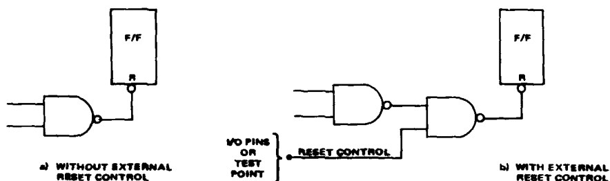
Figure 4.3.1-9. Flip-flop modified for external reset control.
