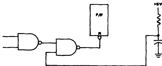
Figure 4.3.1-10. Power-up reset.
