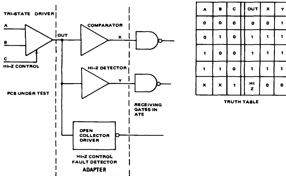
Figure 4.3.3-3. Tri-State Detection Circuit with Hi-Z Control Fault Protection
