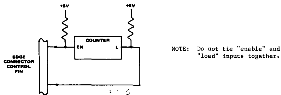
Figure 5.3-2. Provide WIRE-AND at enable and load inputs.
