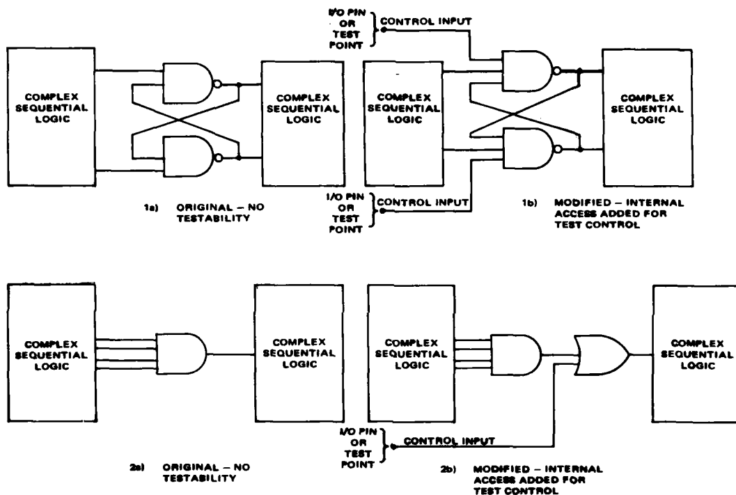
Figure 4.3.1-11. Provide access to internal nodes for test control.
