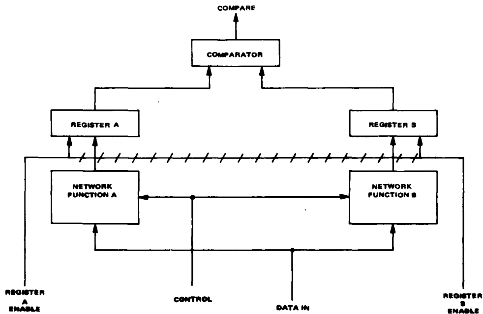
Figure 4.3.1-4. Separate enables allow separate testing of redundant voting networks.
