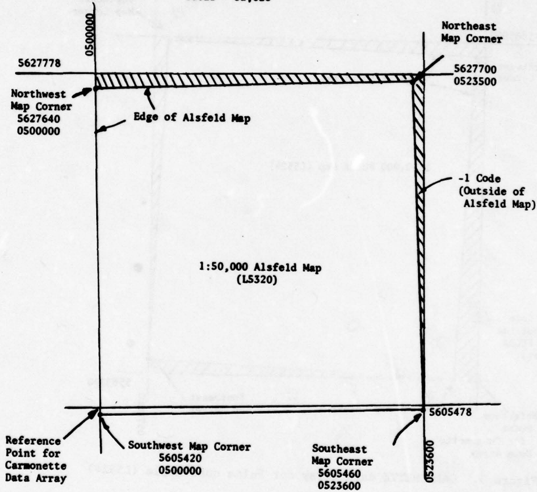
Figure 4. CARMONETTE data array for Alsfield quadrangle (LS320)
