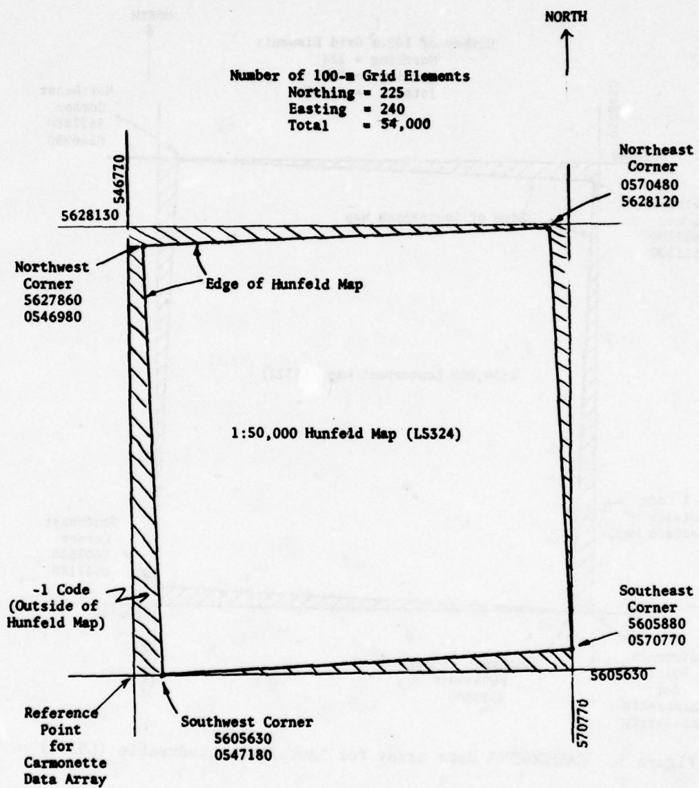
Figure 6. CARMONETTE data array for Hunfeld quadrangle (L5324)
