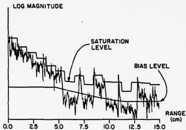
Figure 4.12 Stationary Targets, Raw Echo Signal
