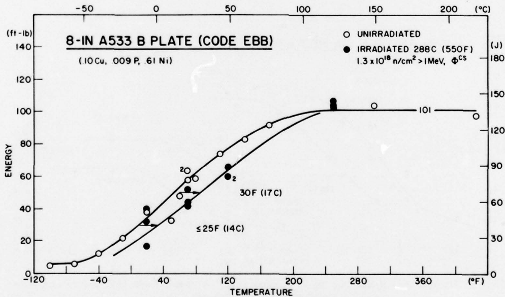
Fig. 3 — Charpy-V notch ductility of the A533-B plate, Code EBB, after low fluence irradiation
