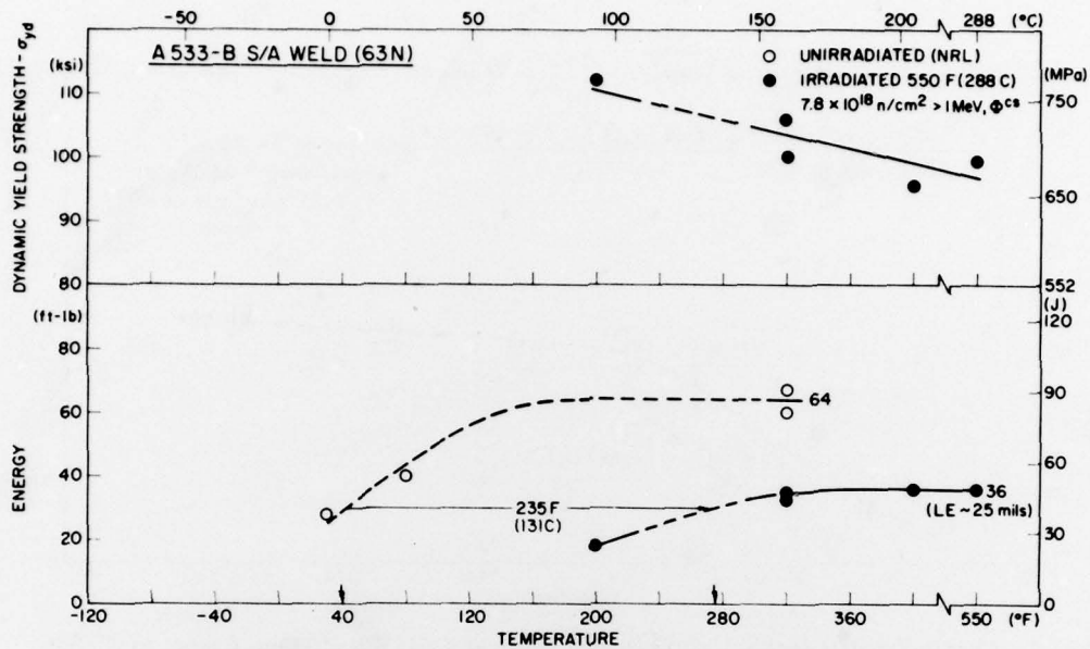
Fig. 8 — Charpy-V notch ductility of submerged arc weld, Code 63N, after intermediate fluence irradiation
