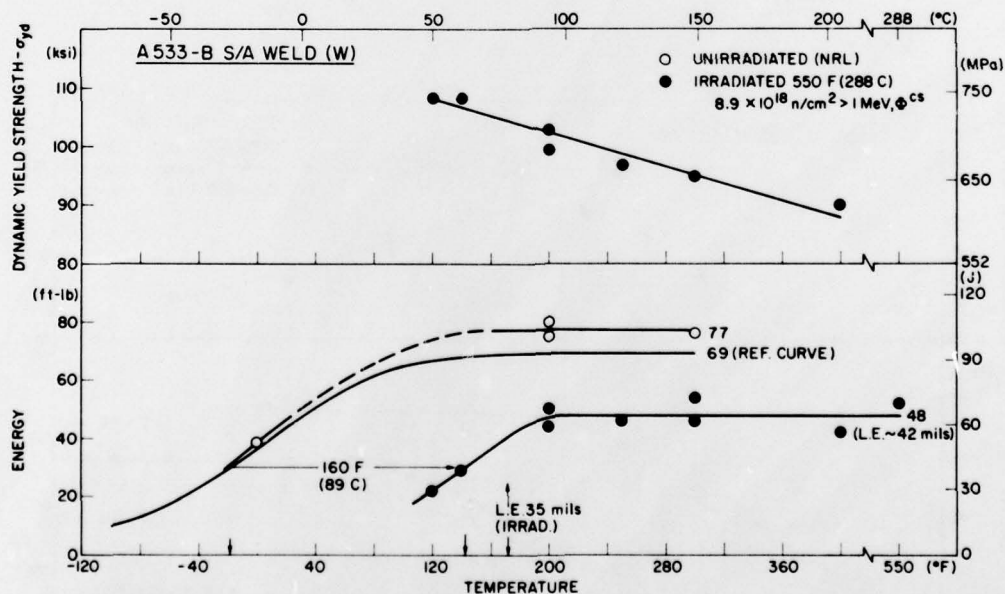
Fig. 7 — Charpy-V notch ductility of submerged arc weld, Code W, after intermediate fluence irradiation. Postirradiation dynamic yield strength determinations from Dynatup load vs time traces are also shown in the upper graph and in Figs. 8 and 9.
