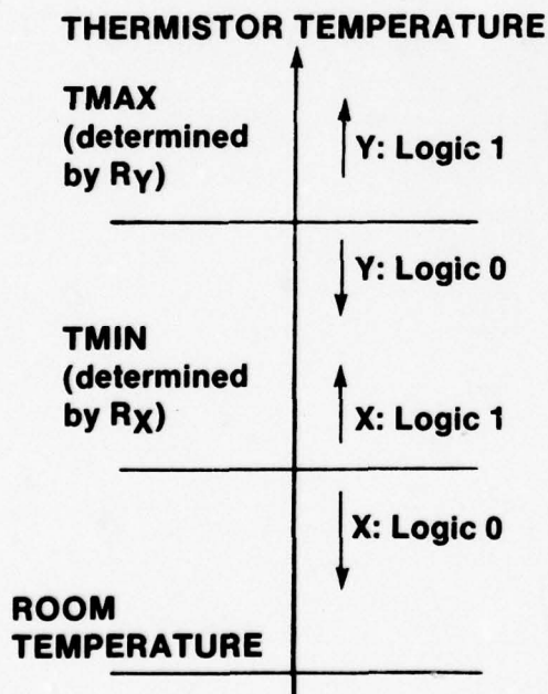
Figure C-2. Logic definition.
