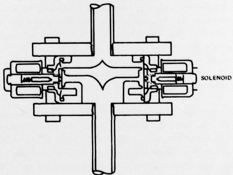
Figure 14. Digital valve
