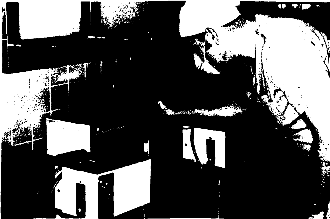
FIGURE 6. SIMULTANEOUS RECORDING OF HALOTHANE AND N 2 O LEVELS DURING SAMPLING.
