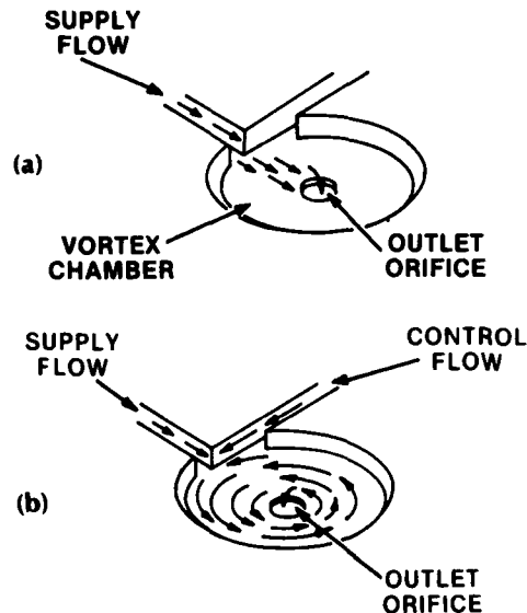
Figure 7. Vortex flow amplifier: (a) without control flow and (b) with control flow.
