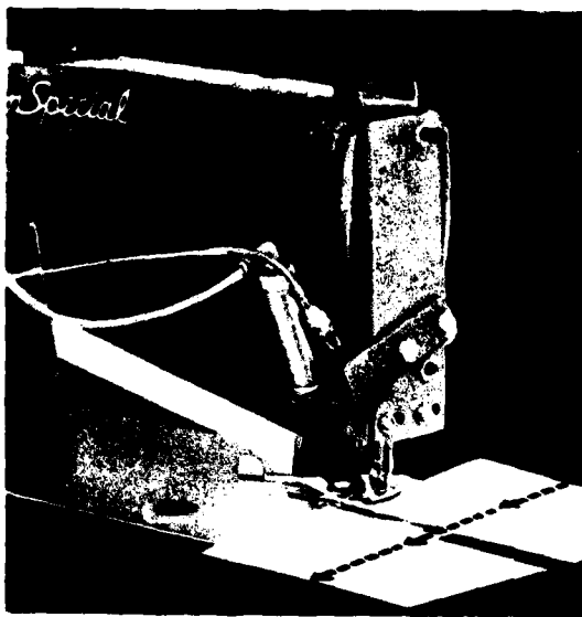
Figure 10. Fluidically controlled industrial sewing-machine attachment.
