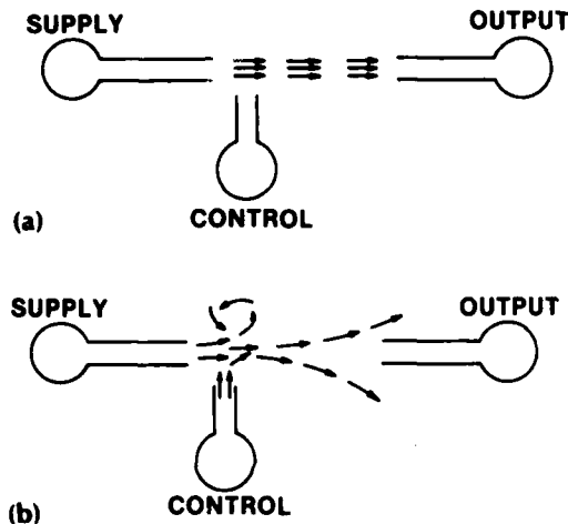
Figure 6. Flow mode control amplifier: (a) without control signal and (b) with control signal applied.
