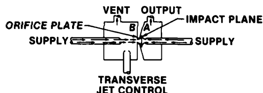
Figure 5. Transverse impact modulator.
