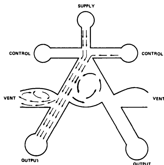
Figure 4. Wall-attachment fluidic bistable amplifier.
