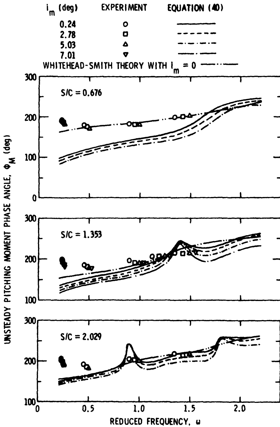
Figure 36. Comparison of Experimental and Theoretical Unsteady Pitching Moment Phase Angles with y_{max}^+ = 0 and \xi = 35^\circ .
