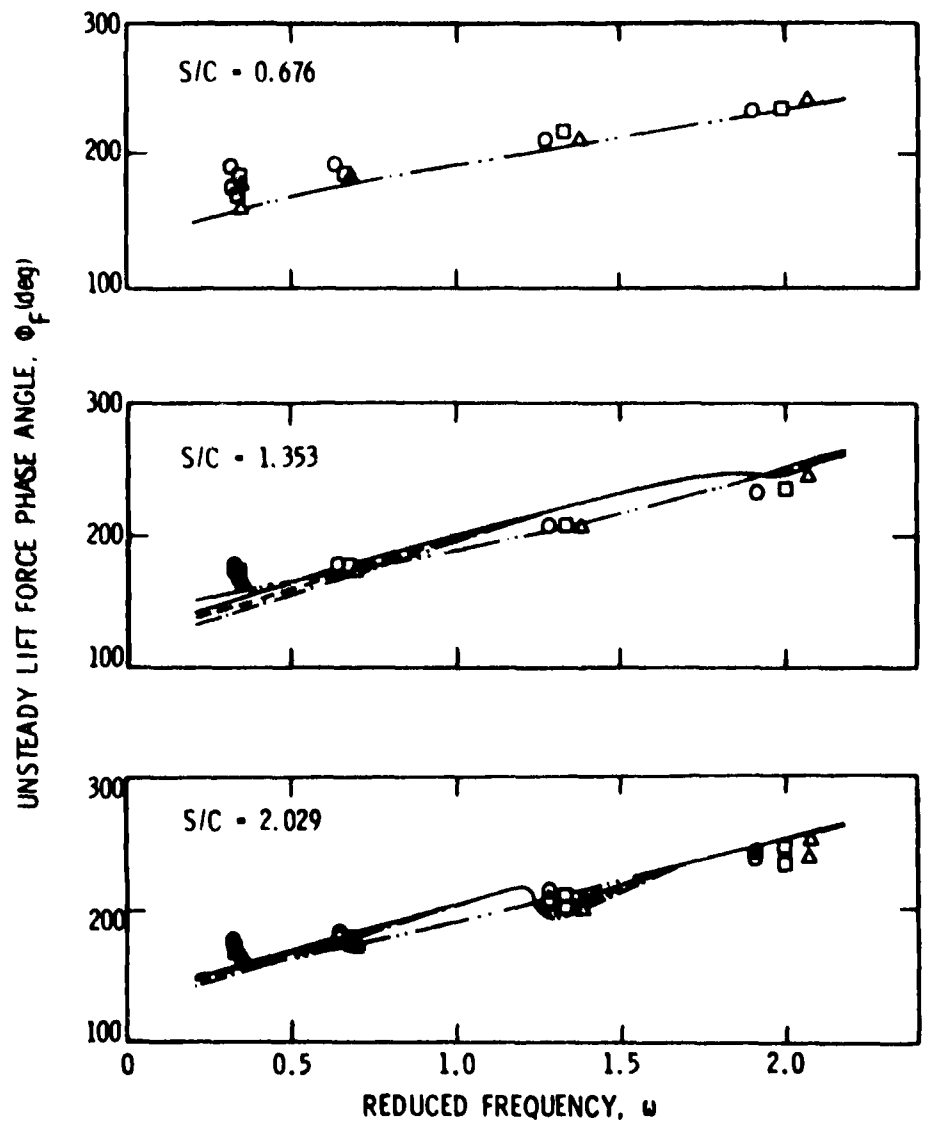
Figure 35. Comparison of Experimental and Theoretical Unsteady Lift Force Phase Angles with y_{max}^+ = 0 and \xi = 55^\circ .
