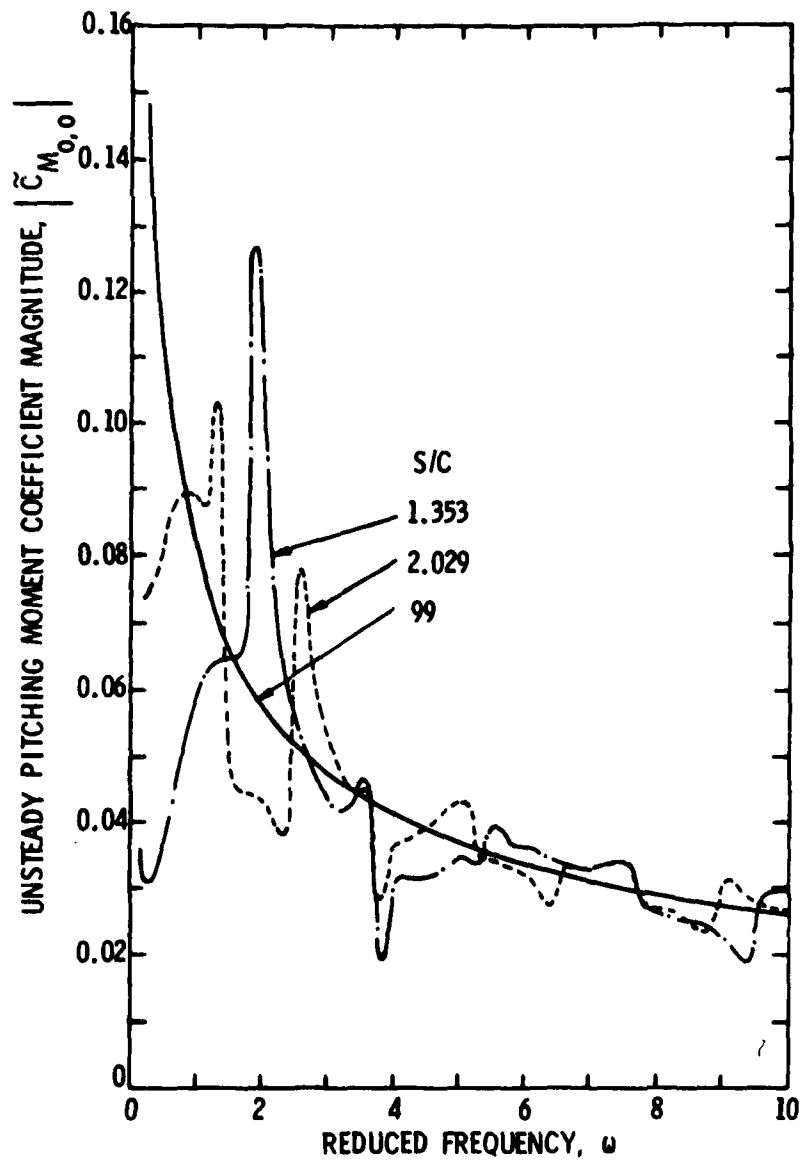
Figure 50. Unsteady Pitching Moment Coefficient with i_m = y_{\max}^+ = 0 and \xi = 55^\circ .
