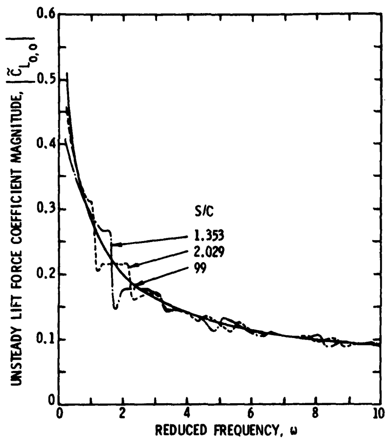
Figure 40. Unsteady Lift Force Coefficient with i_m = y_{max}^+ = 0 and \xi = 45^\circ .
