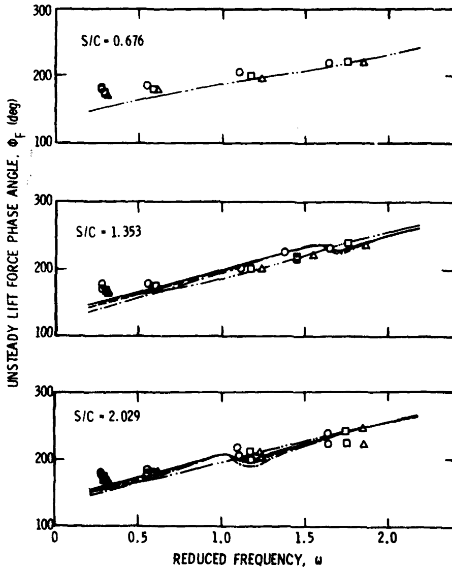
Figure 34. Comparison of Experimental and Theoretical Unsteady Lift Force Phase Angles with y_{max}^+ = 0 and \xi = 45^\circ .
