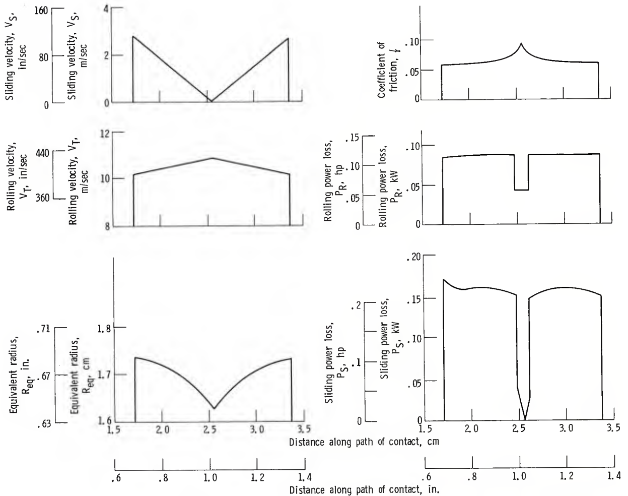
Figure 2. - Instantaneous values of rolling velocity, sliding velocity, coefficient of friction, rolling power loss, and sliding power loss across path of contact of 4.0-centimeter-(1.563-in.-) wide gear of reference 6. Pinion speed, 2000 rpm; pinion torque, 271 newton-meters (200 ft-lb).
