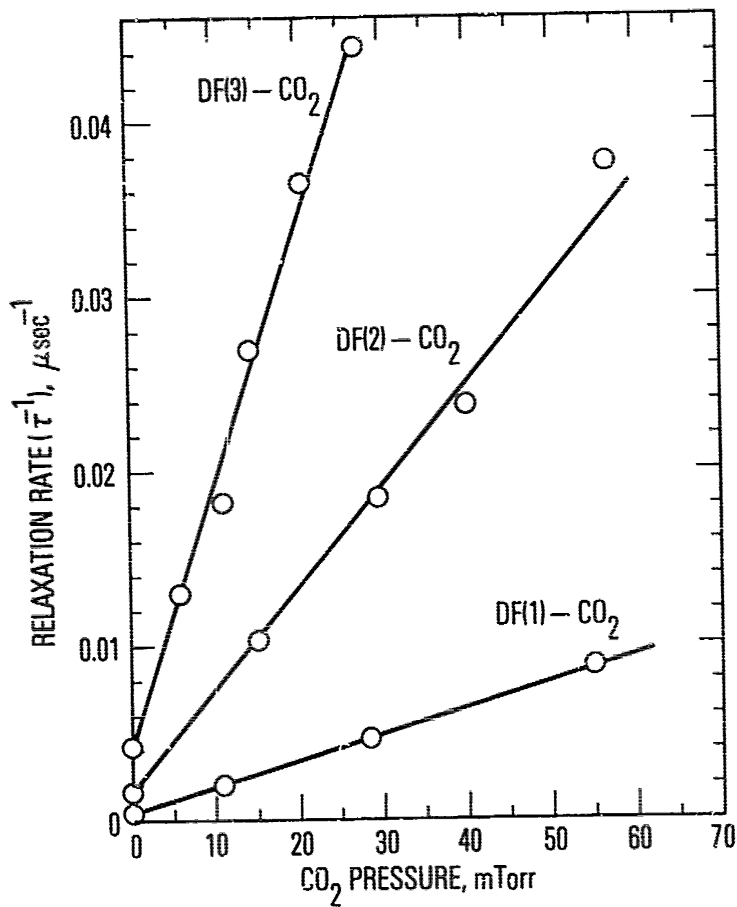
Fig. 6. Relaxation Rates of DF(v) in CO 2
