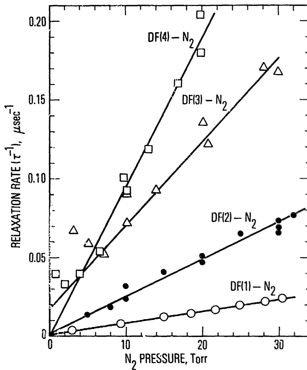
Fig. 5. Relaxation Rates of DF(v) in N 2
