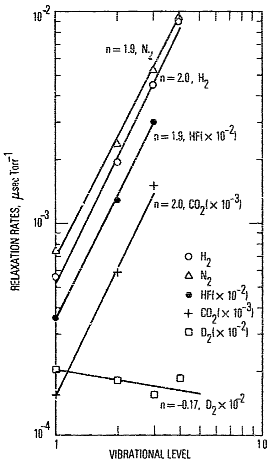
Fig. 8. Relaxation Rates of \text{DF}(v) in \text{N}_2 , \text{H}_2 , \text{HF} , \text{CO}_2 , \text{D}_2 vs Vibrational Level
