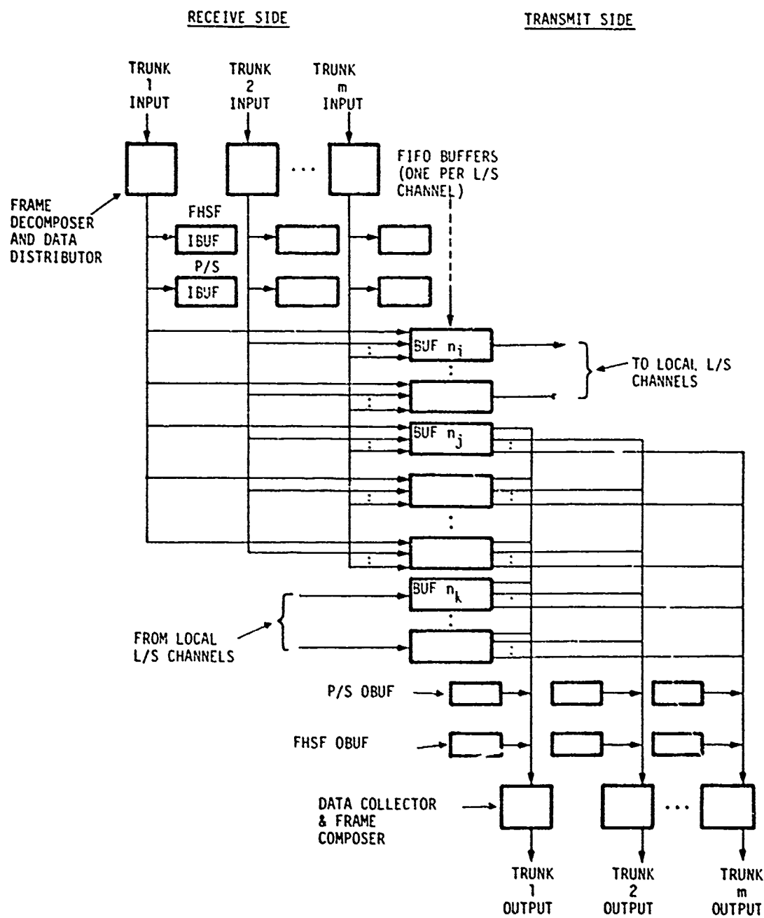
Fig. 7.7 Node data flow -- Decomposition, switching, composition.
