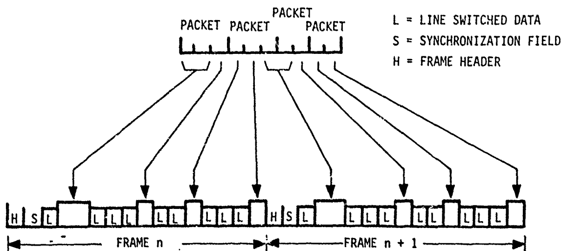
Fig. 7.4 Packet distribution.
