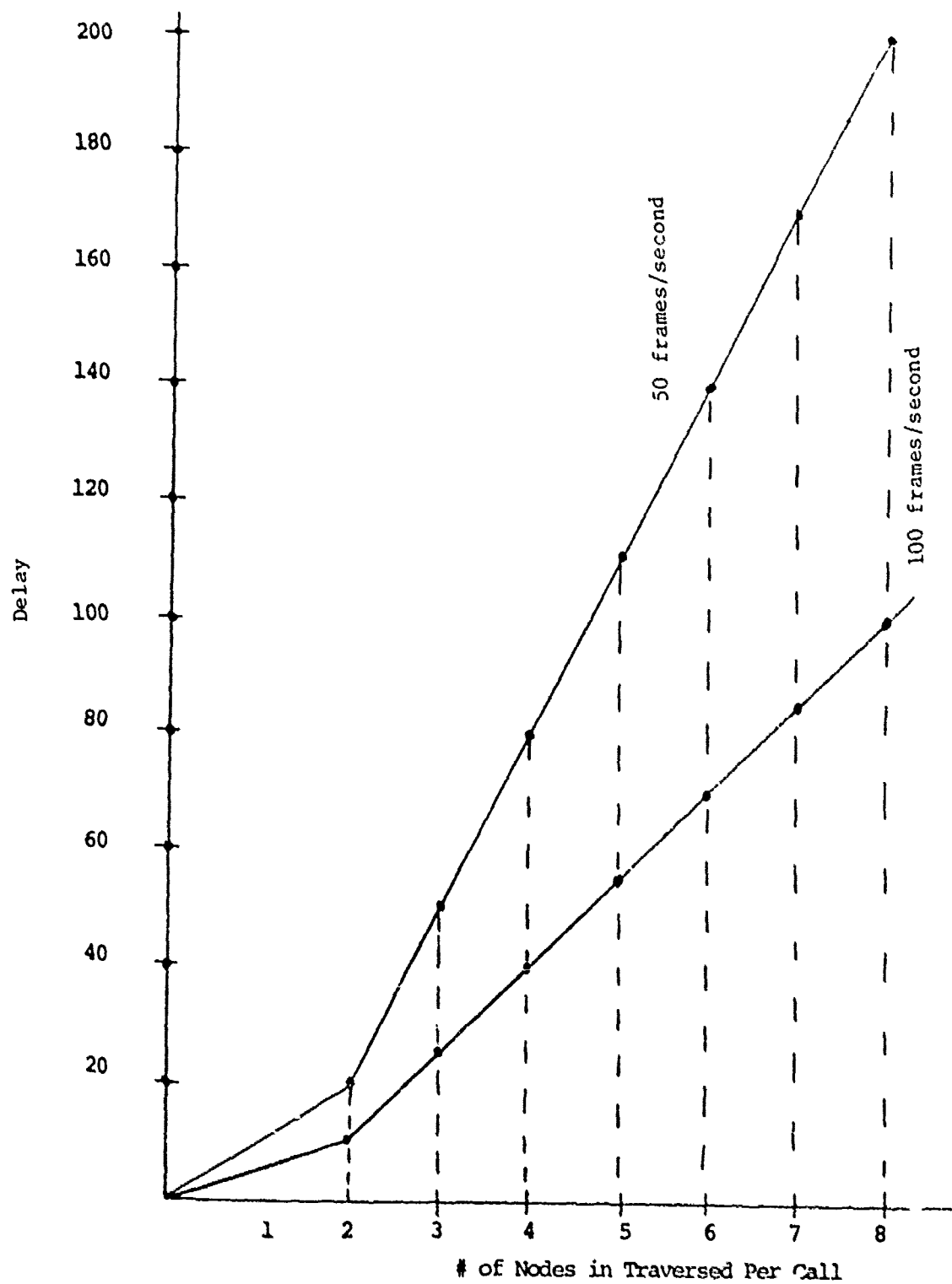
Fig. 8.2 End-to-end Class 1 traffic delays.
