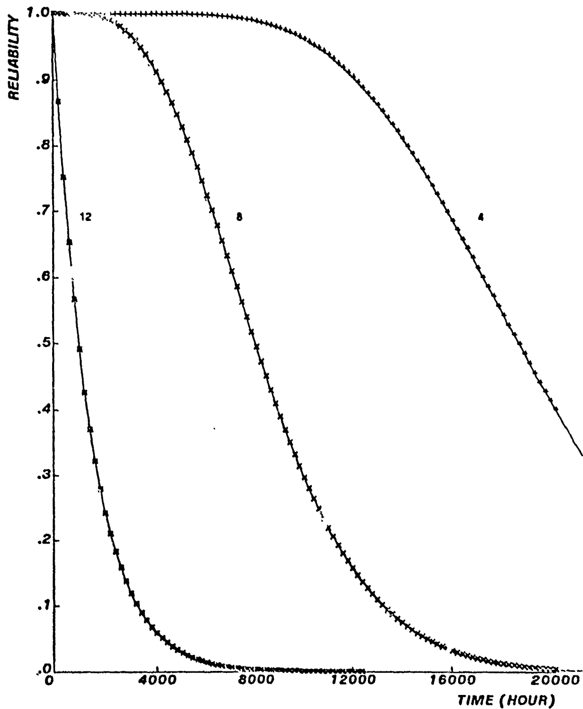
Fig. 3.16 Tandem with 12 processors, 32Kw/processor, 16Kw/processor required,
