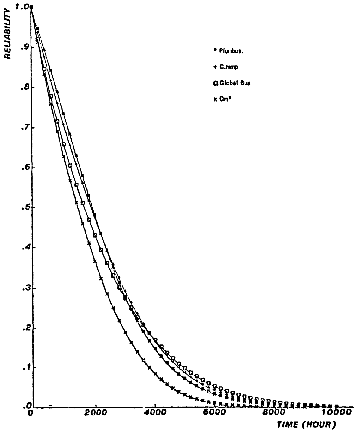
Fig. 3.19 Equivalent performance 62% voice, 28% of data, normal processor, 24% of T1 carrier in each line, three lines
