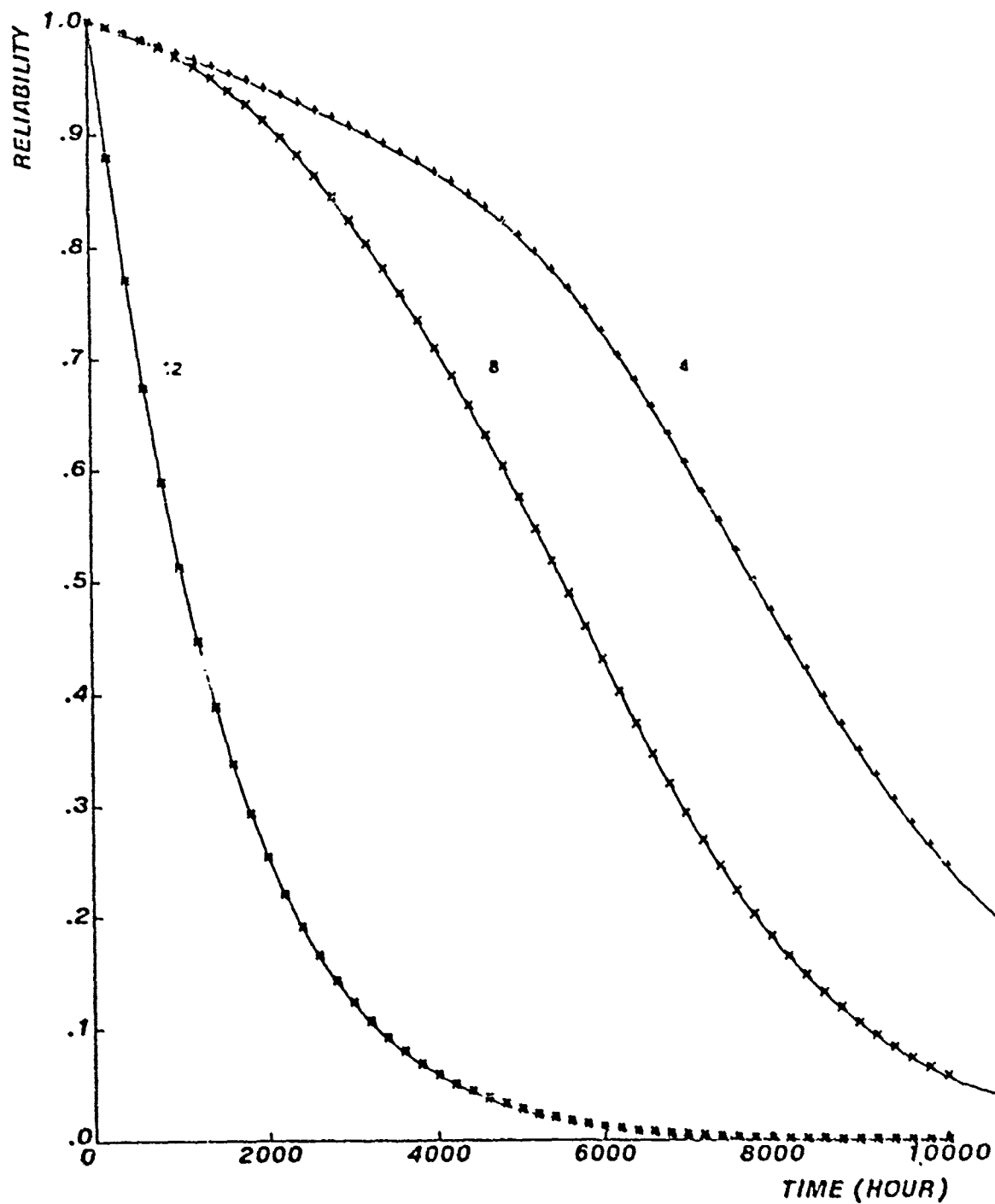
Fig. 3.10 Pluribus with 6 processor buses, 3 memory buses, 128Kw/memory bus, 216Kw required.
