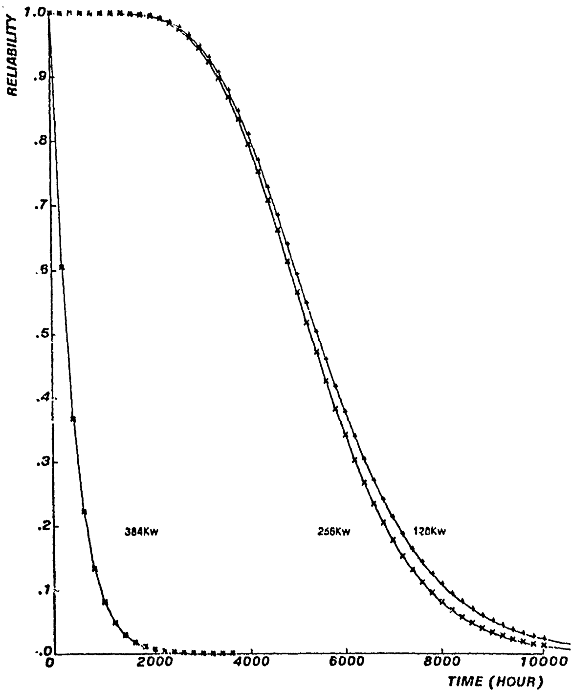
Fig. 3.15 Global bus with 12 processors, 32Kw/processor, 8 processors required
