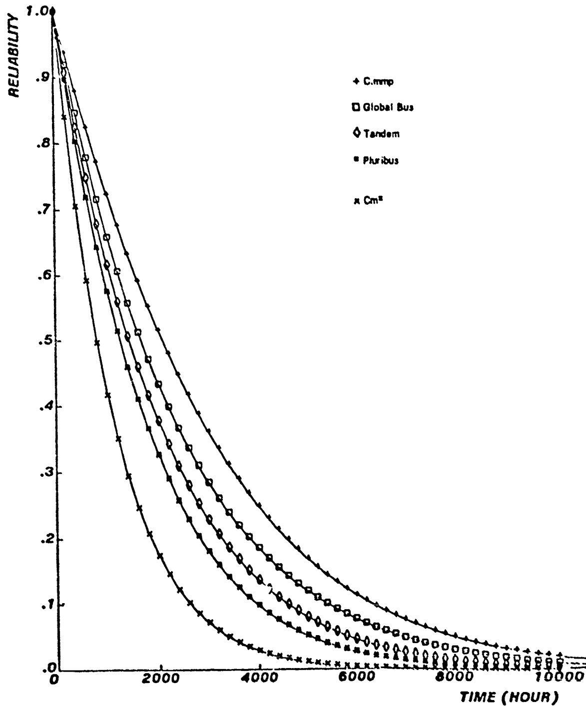
Fig. 3.21 Equivalent performance 62% voice, 24% data, ten times faster processor, 24% of T1 carrier in each line, three lines.
