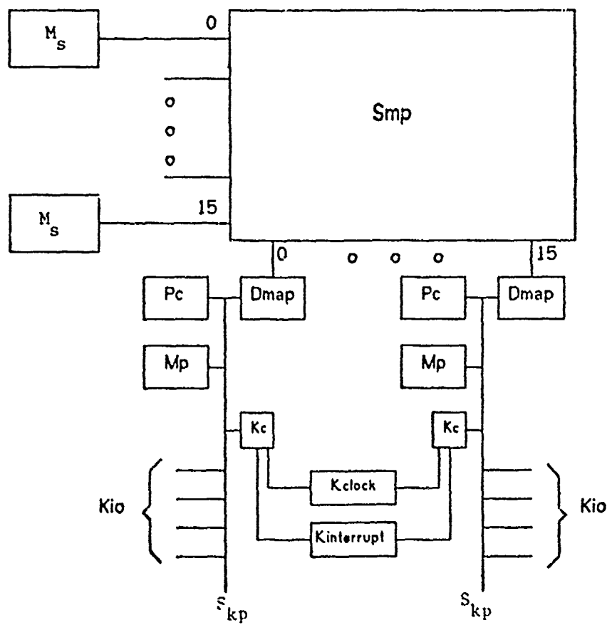
Fig. 6.1 C.mmp
