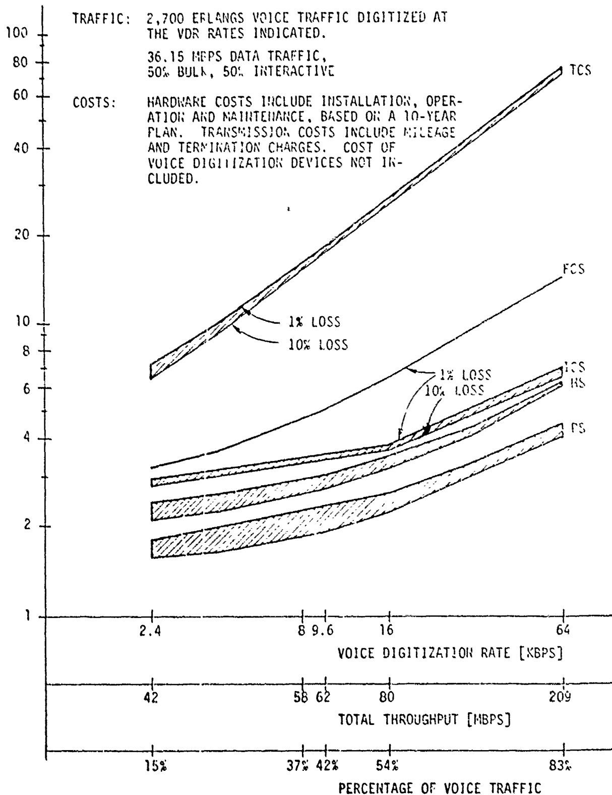
Fig. 2,3 Monthly backbone switching and transmission cost as a function of voice digitization rate (VDR) and switching technology (TCS - traditional circuit switching; FCS - fast circuit switching; ICS - ideal circuit switching; HS - hybrid switching; PS - packet switching). Cost ranges indicate alternative operation scenarios (HS and PS) or blocking probability range (TCS, ICS).
