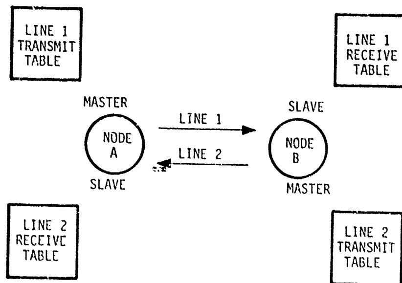
Fig. 7.5 Network Link.
