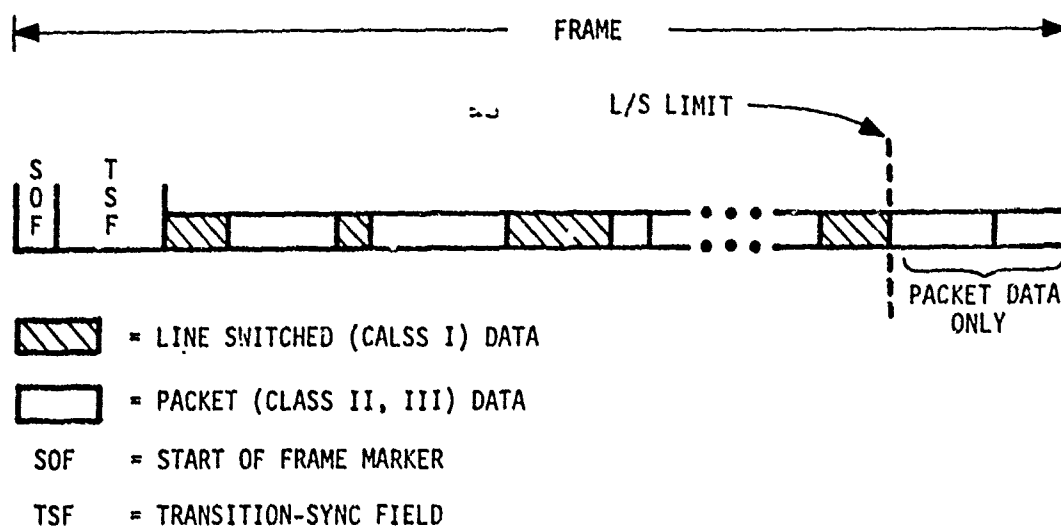
Fig. 7.3 Line switched/packet data integration.
