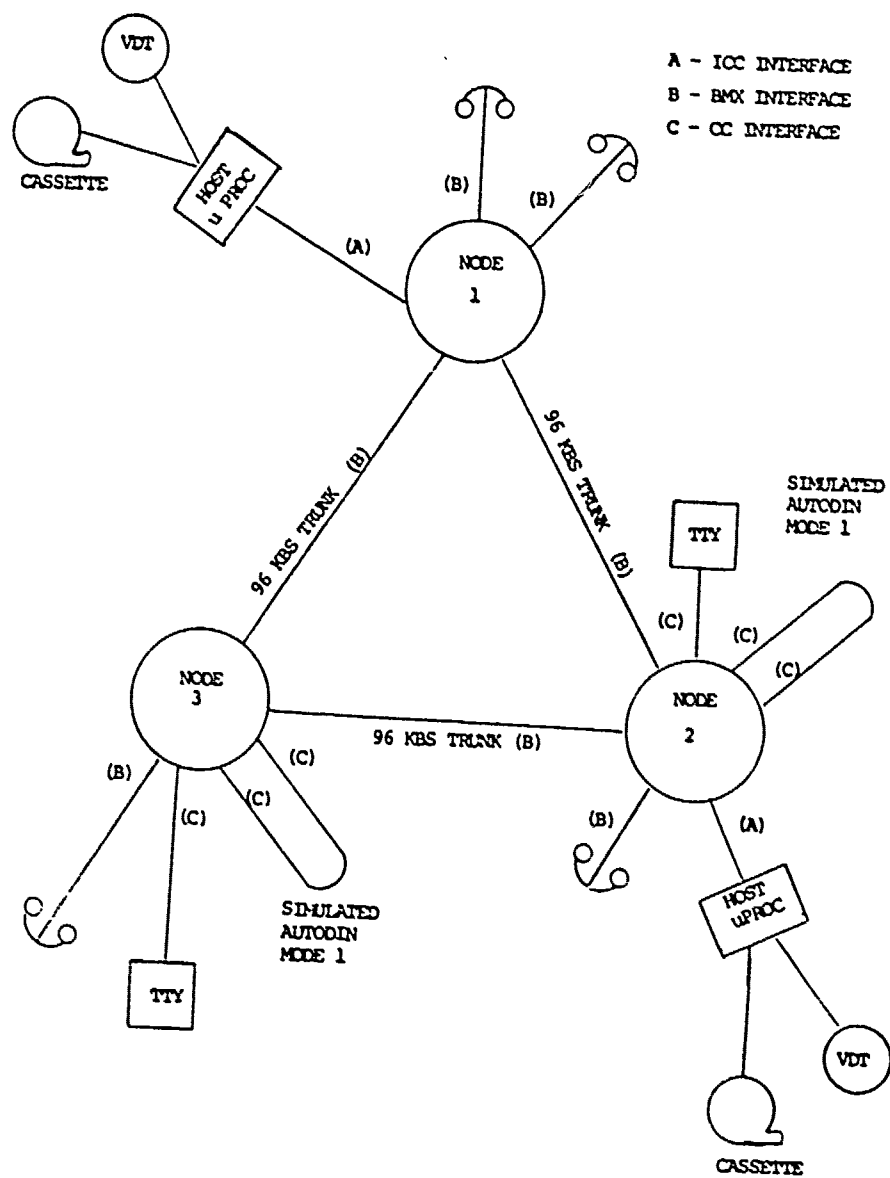
Fig. 8.6 Three node subnetwork function configuration.
