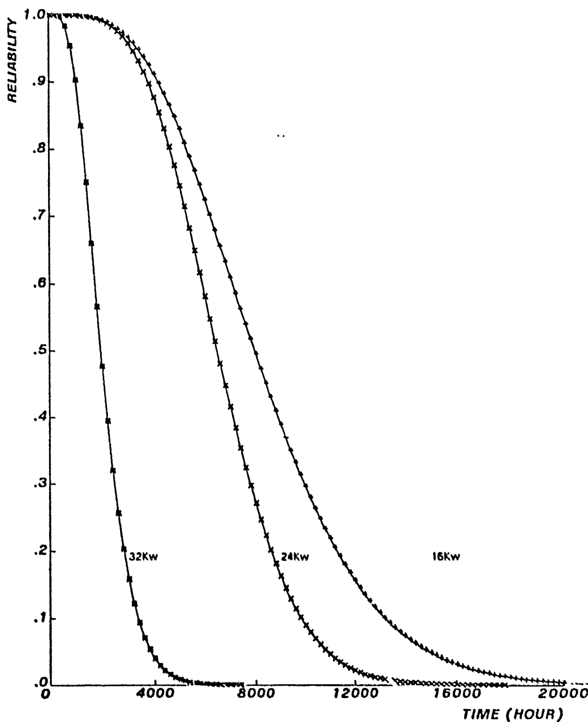
Fig. 3.17 Tandem with 12 processors, 32Kw/processor, 8 processors required
