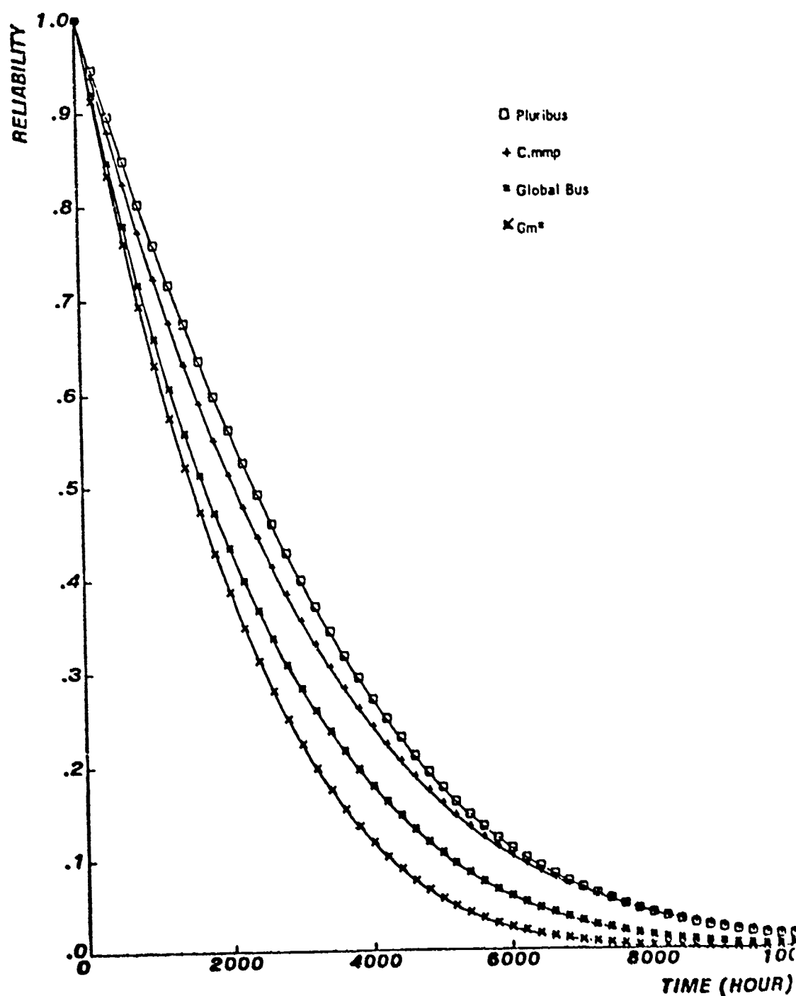
Fig. 3.20 Equivalent performance 62% voice, 28% data, ten times faster processor, 48% of T1 carrier in each line, three lines.
