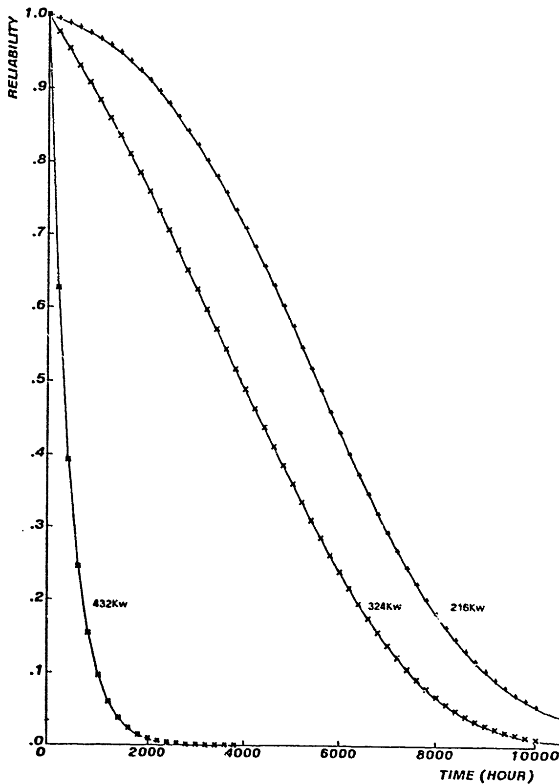
Fig. 3.11 Pluribus with 6 processor buses, 3 memory buses, 128Kw/memory bus, 8 processors required,
