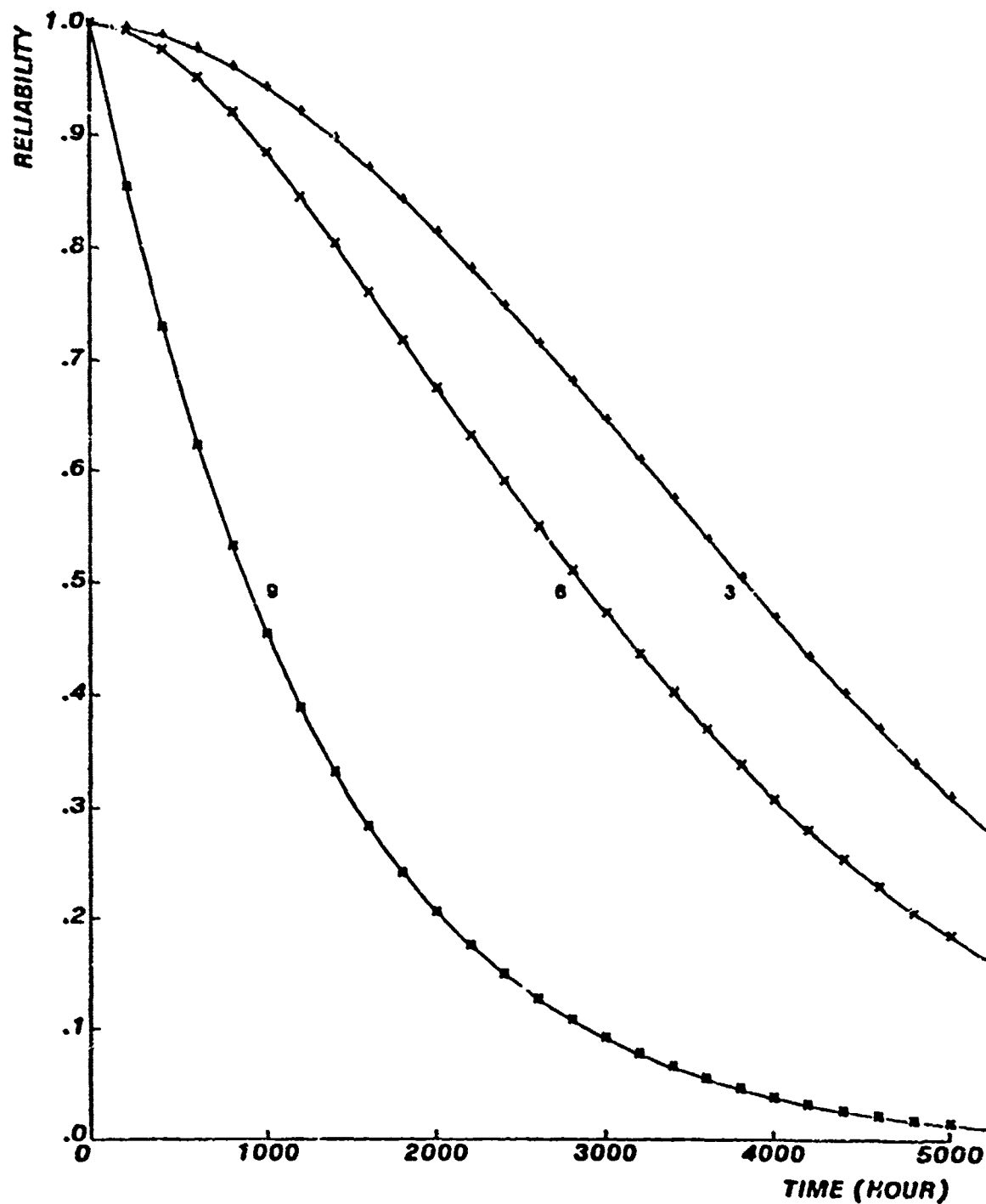
Fig. 3.12 3-Cluster Cm* with three processors/cluster, 32Kw/Cm, 144Kw required (parallel buses)
