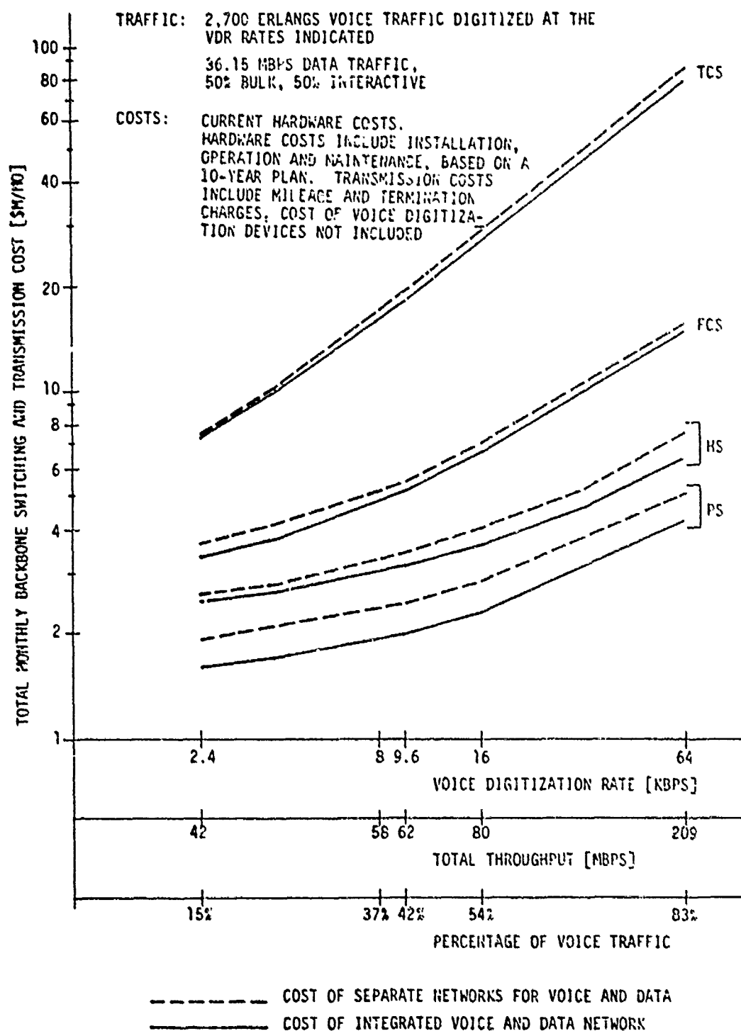
Fig. 2.2 Integrated versus segregated voice and data networks as a function of voice digitization rate (VDR) and switching technology (TCS - traditional circuit switching; FCS - fast circuit switching; HS - hybrid circuit switching; PS - packet switching).
