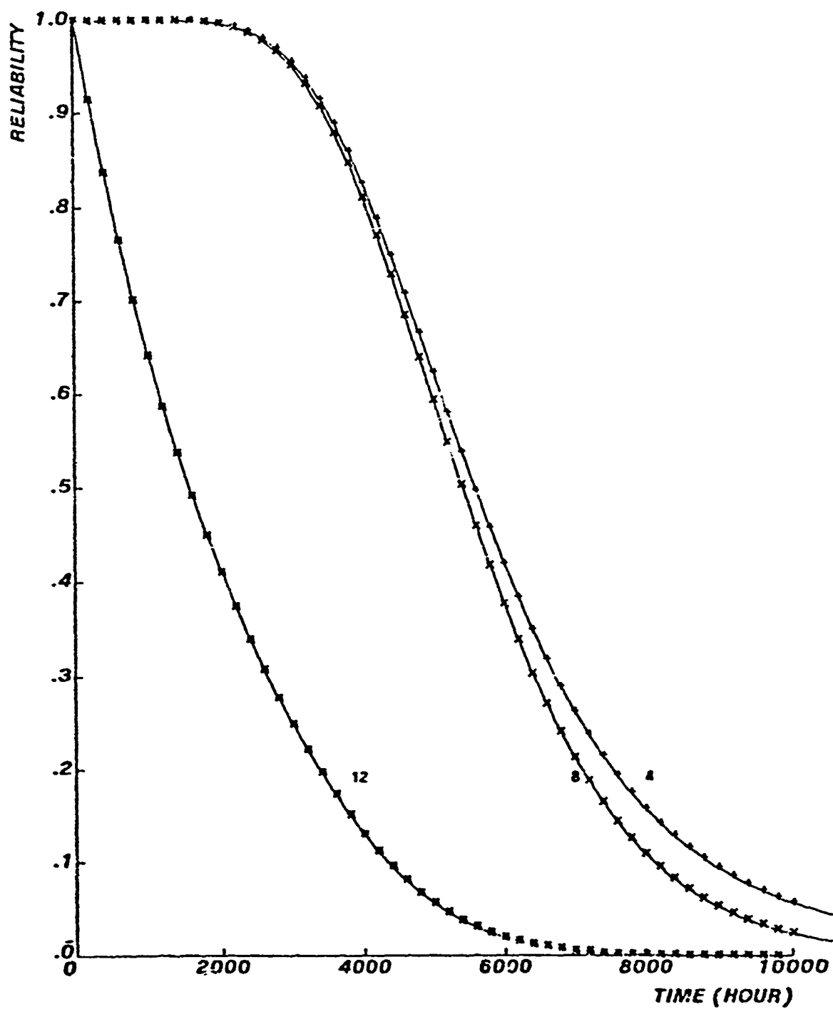
Fig. 3.14 Global bus with 12 processors, 32Kw/processor, 128Kw required
