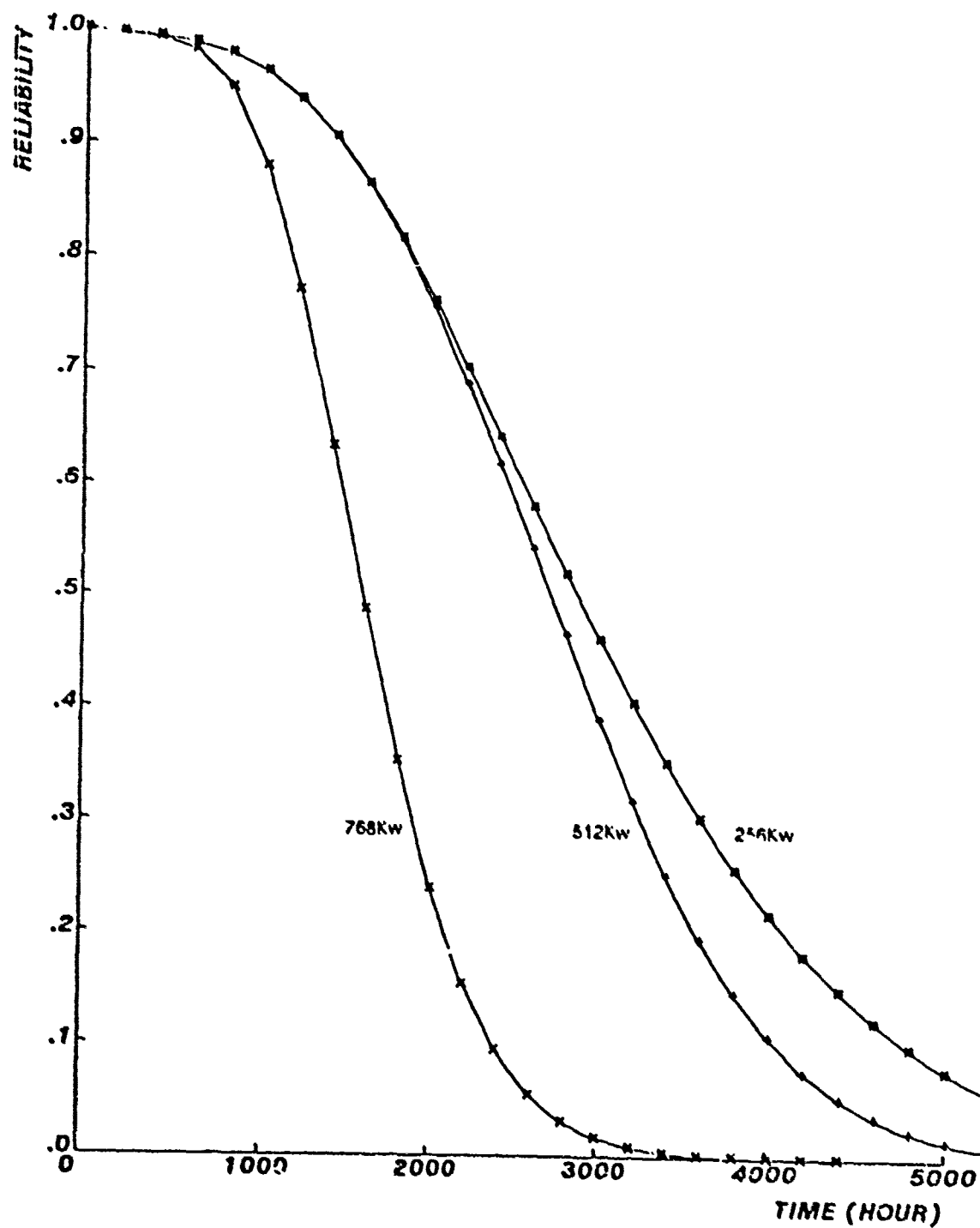
Fig. 3.9 C.mmp with 64Kw per port, 12 processors required (distributed switch)
