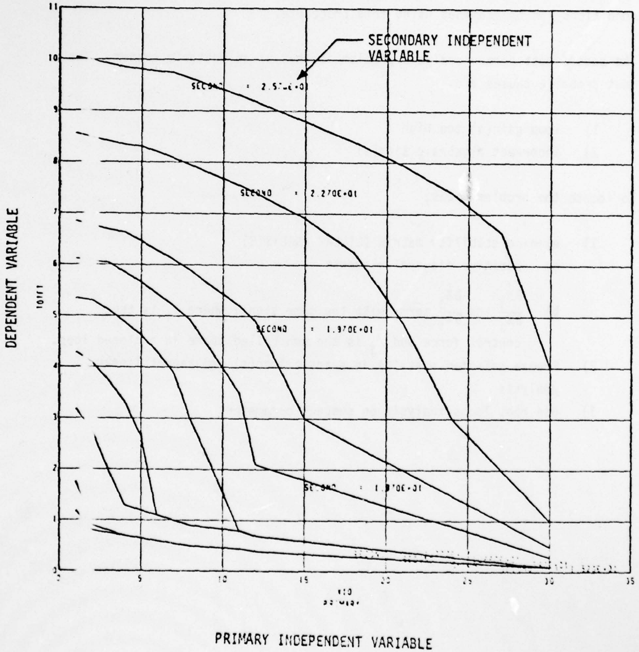
Figure 41 ACLS Fan Map as Plotted by EASY
