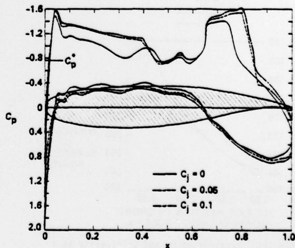
Fig. 9. Effect of Blowing Coefficient, ( C_j ), Variations on Chordwise Pressures for CAD USB Supercritical Airfoil, M_\infty=0.703 , \alpha=0^\circ , (Slot Location at 65% Chord).
