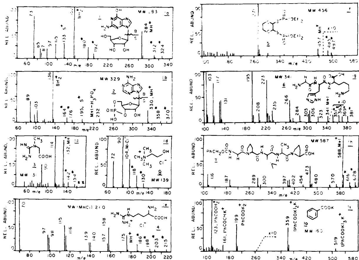
Figure 1. Activated-emitter, solids-probe, methane (0.5 Torr) CI spectra of: (a) guanosine (1) (32 mA); (b) cyclic adenosine monophosphate (2) (35 mA); (c) creatine (3) (32 mA); (d) choline chloride (8) (28 mA); (e) arginine hydrochloride (4) (26 mA); (f) dioxathion (5) (30 mA); (g) glycyl-histidyl-lysine (6) (32 mA); (h) CBz-glycyl-prolyl-leucyl-alanyl-proline (7) (36 mA); and (i) potassium benzoate (10) (40 mA). All spectra except 1h were recorded using procedure 1. Sample sizes were between 100 ng and 1 \mu g. Ions designated by an asterisk contain a methane reagent ion, C_2H_5^+ or C_3H_5^+ , plus the sample molecule or a neutral fragment derived from the sample molecule.
