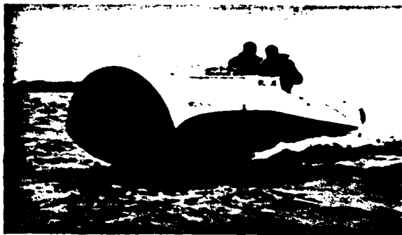
Figure 10. The "slicing" action of the supercritical hull is illustrated here as GAYLE Boat I cuts through a wave at 40 knots, instead of pounding over it, as would a conventional boat.
