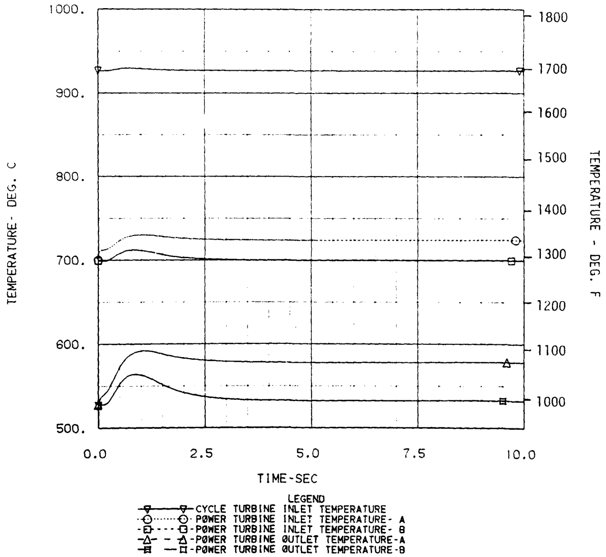
Figure 6-79. Turbine Helium Temperatures
