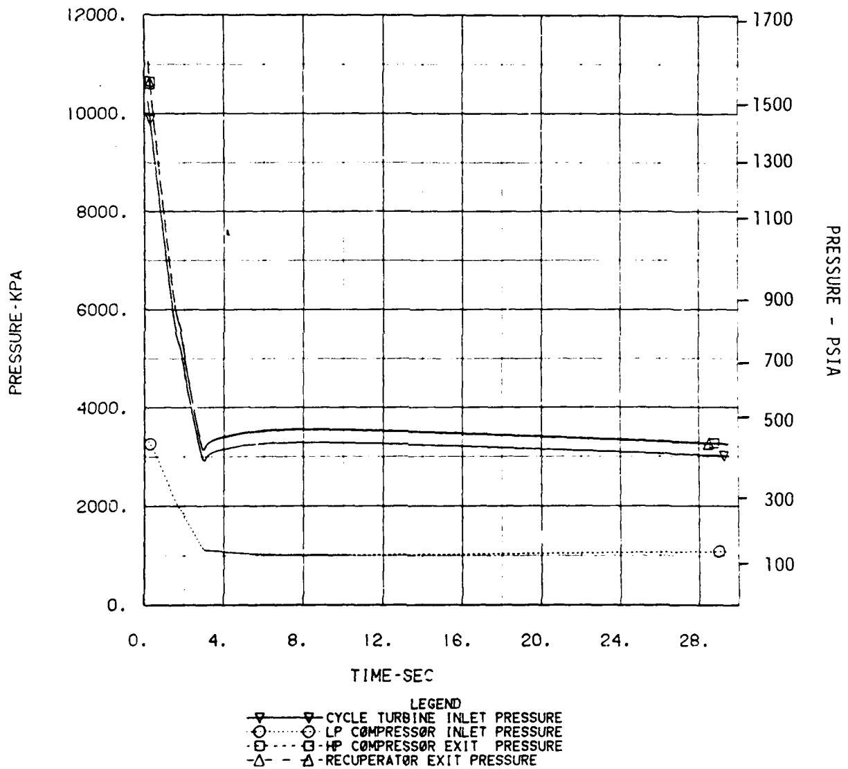
Figure 6-33. Turbomachinery Pressures
