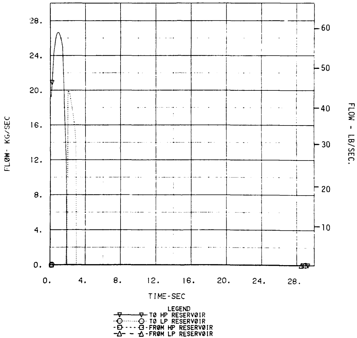
Figure 6-36. Inventory Flows
