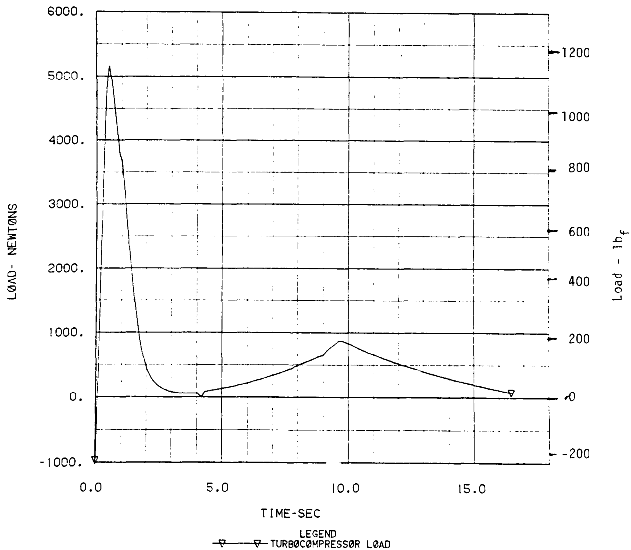
Figure 6-55. Turbocompressor Thrust Bearing Load
