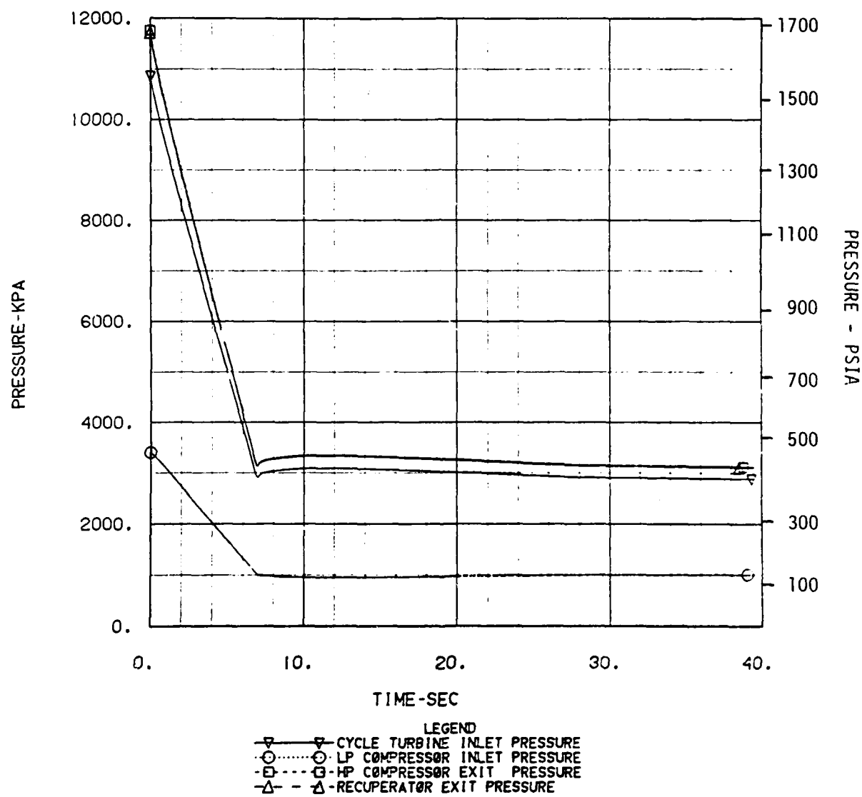
Figure 6-15. Turbomachinery Pressures
