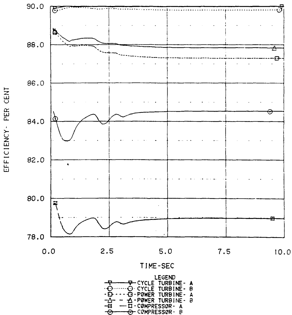
Figure 6-72. Turbomachinery Efficiencies
