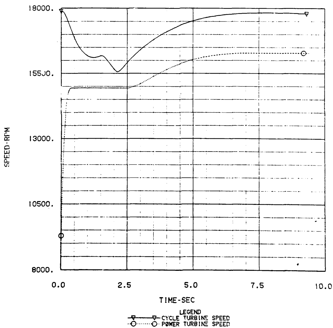
Figure 6-43. Turbomachinery Speeds
