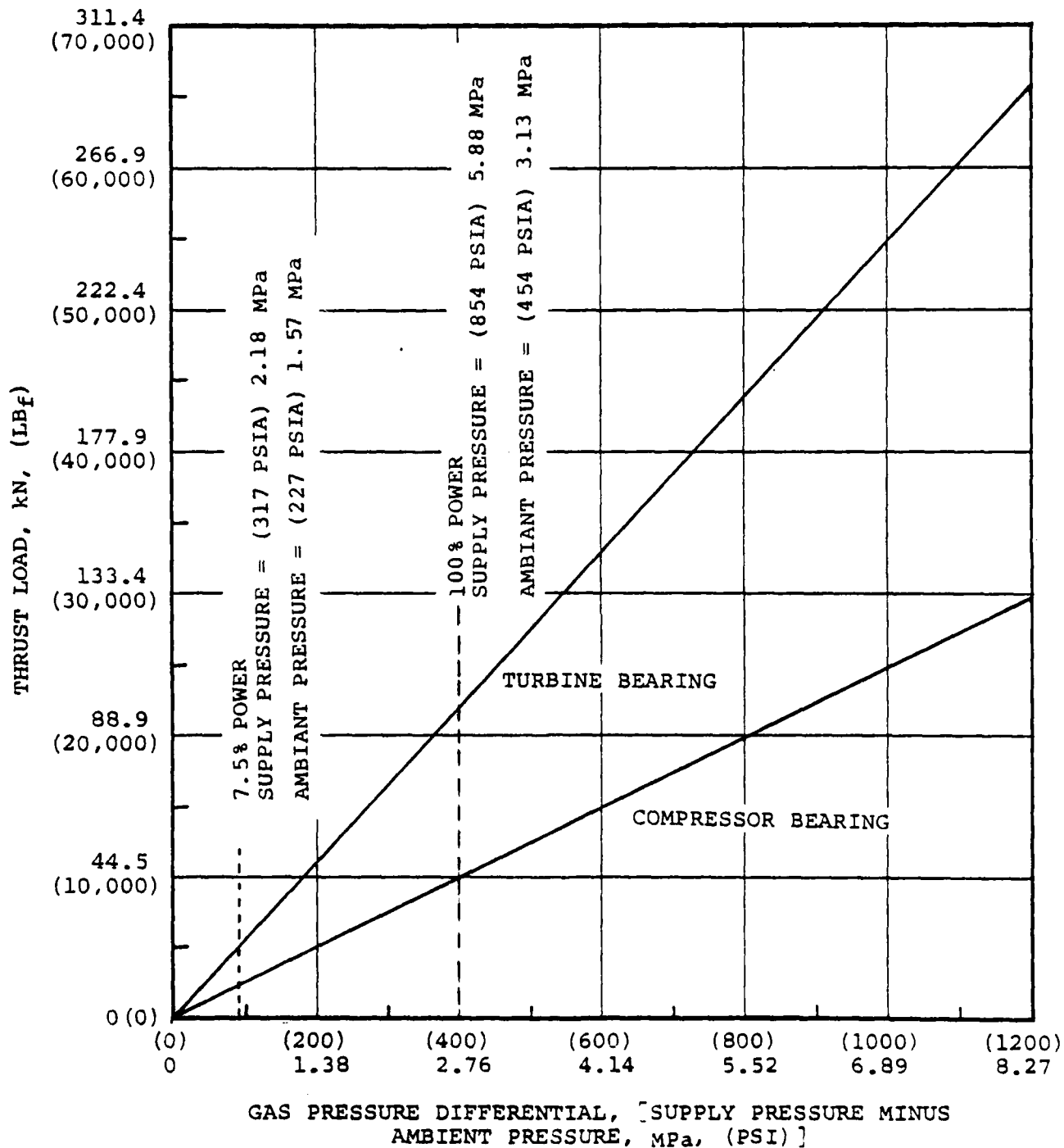
Figure 7-21. Effect of Power Level on Thrust Load Capacity Helium Lubricated Externally Pressurized Thrust Bearings
