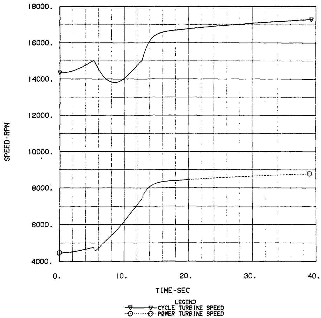
Figure 6-25. Turbomachinery Speeds
