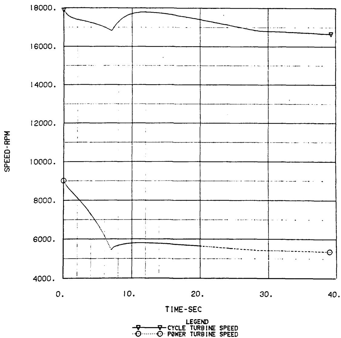
Figure 6-16. Turbomachinery Speeds
