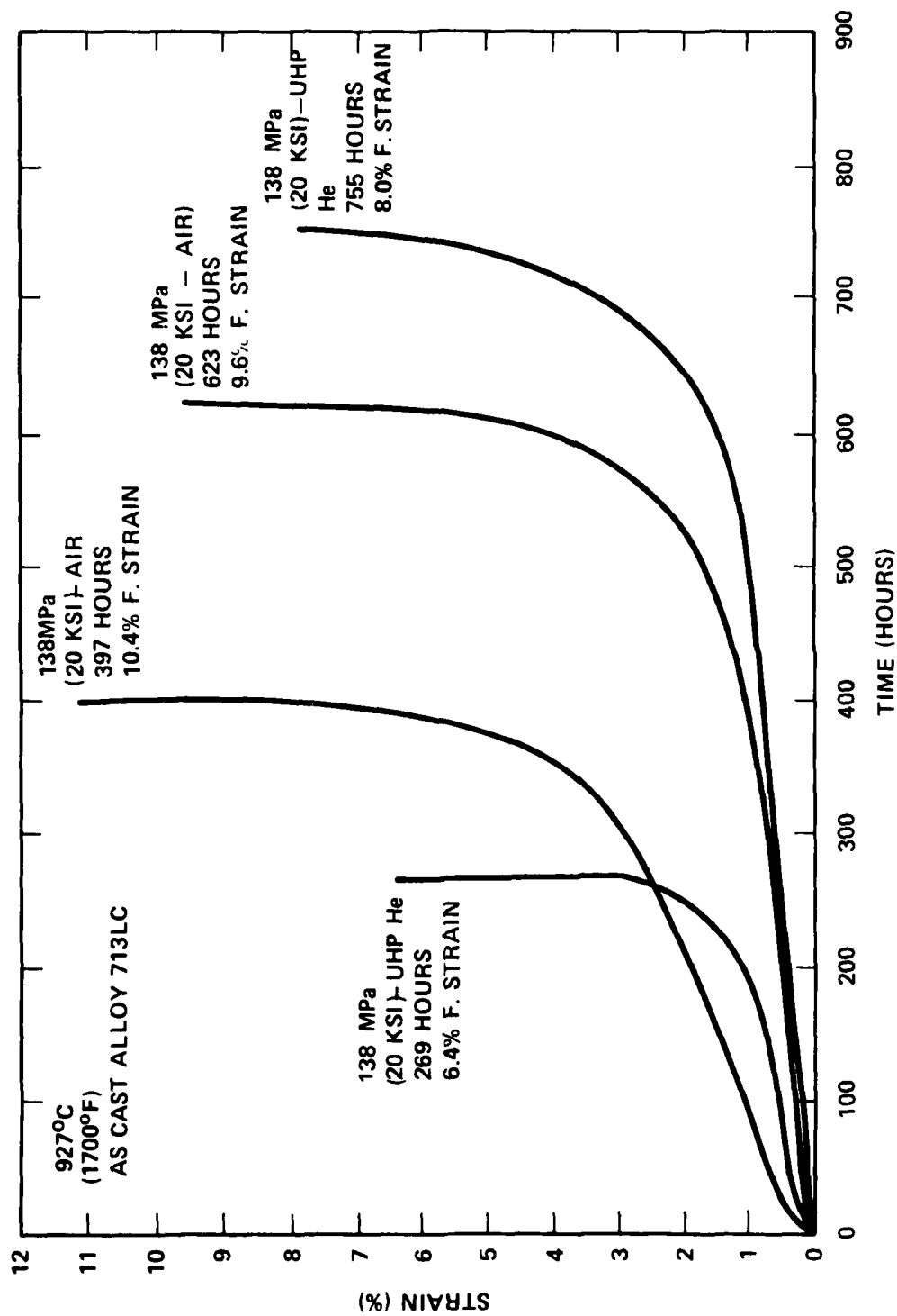
Figure 9-14. Creep-Rupture Curve for As-Cast Alloy 713LC
