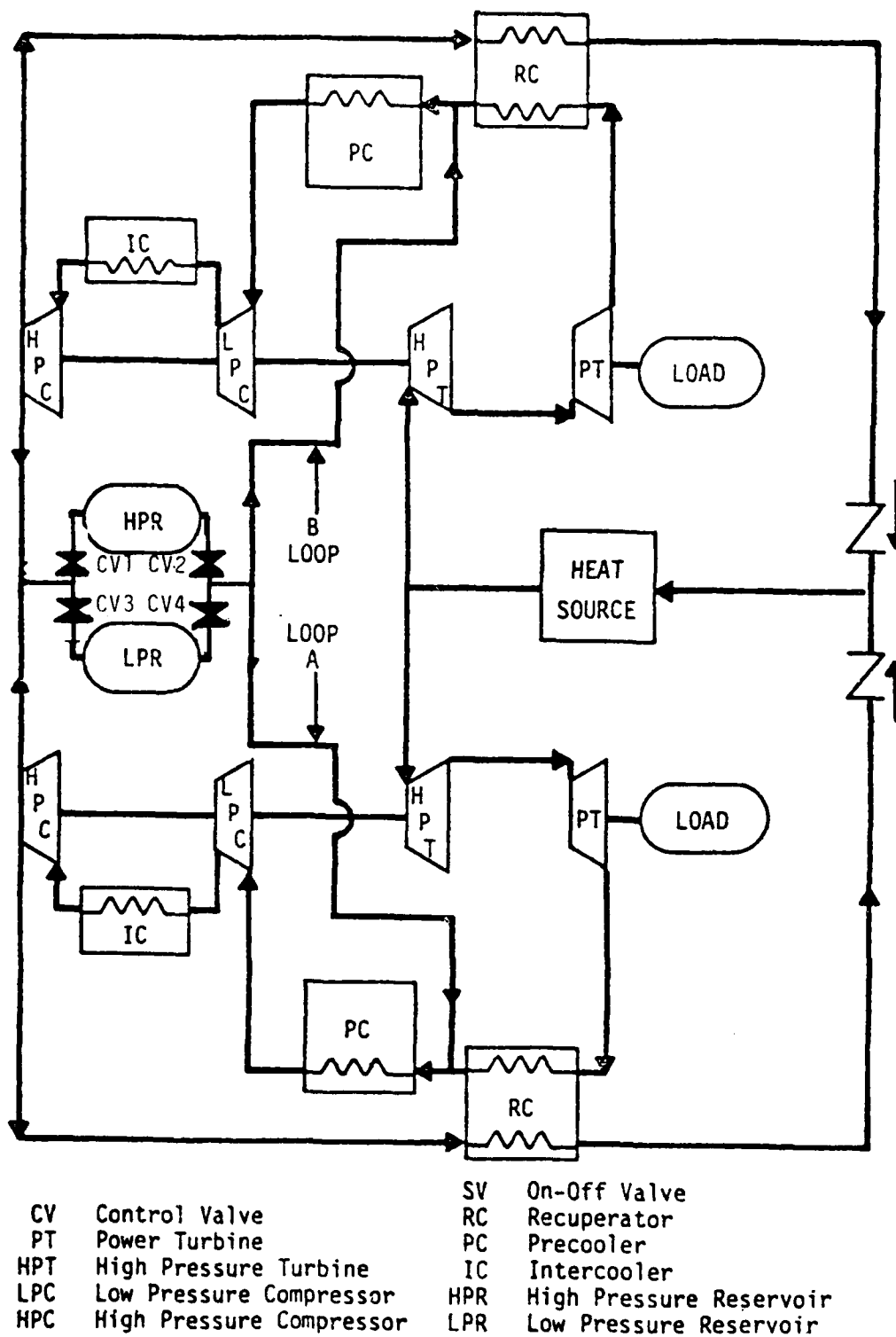
Figure 6-1. Helium Inventory Control Schematic
