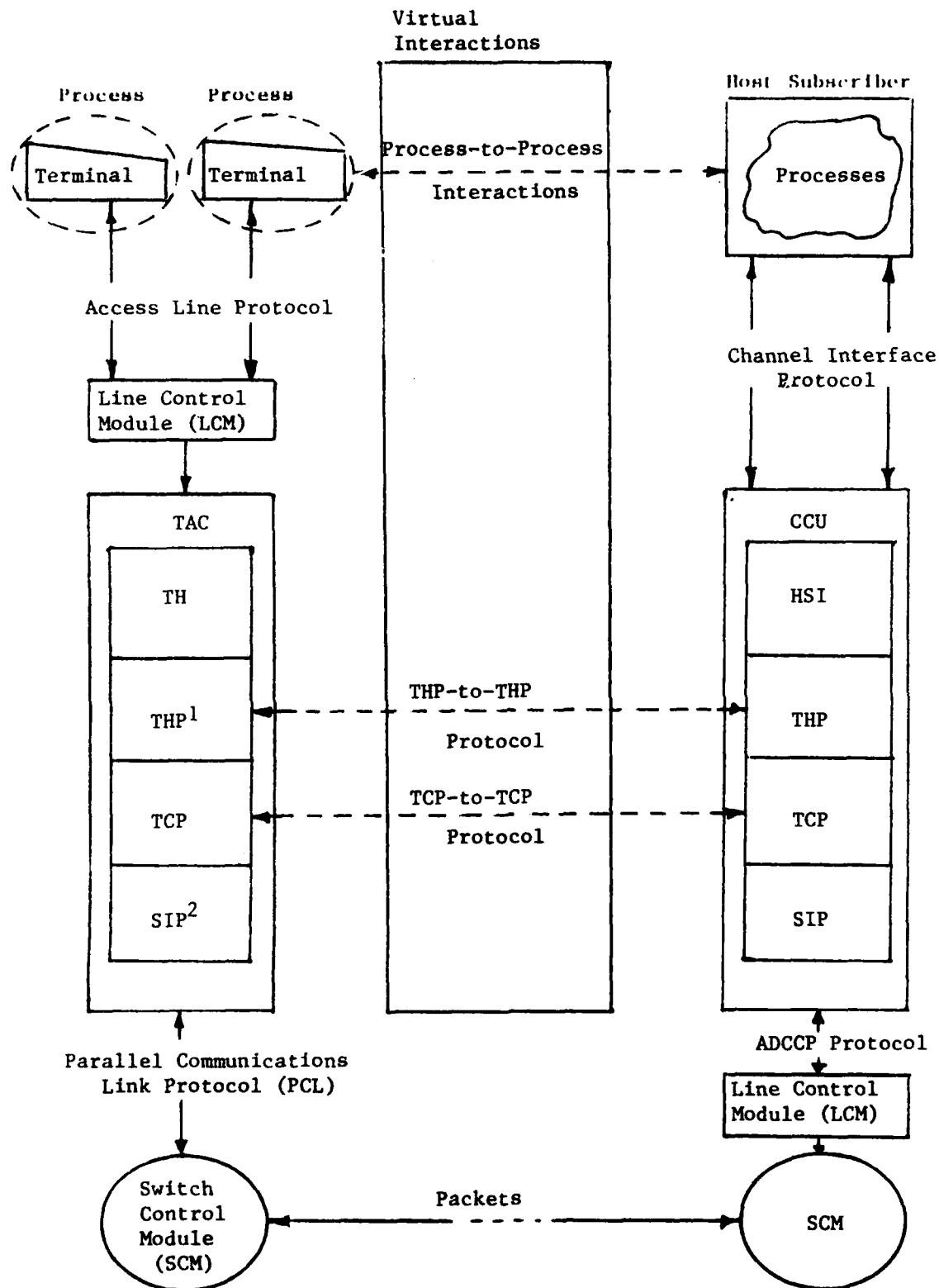
Figure 5. Levels of Protocol Interaction Source: AUTODIN II Design Plan Vol VI, Appendix D
