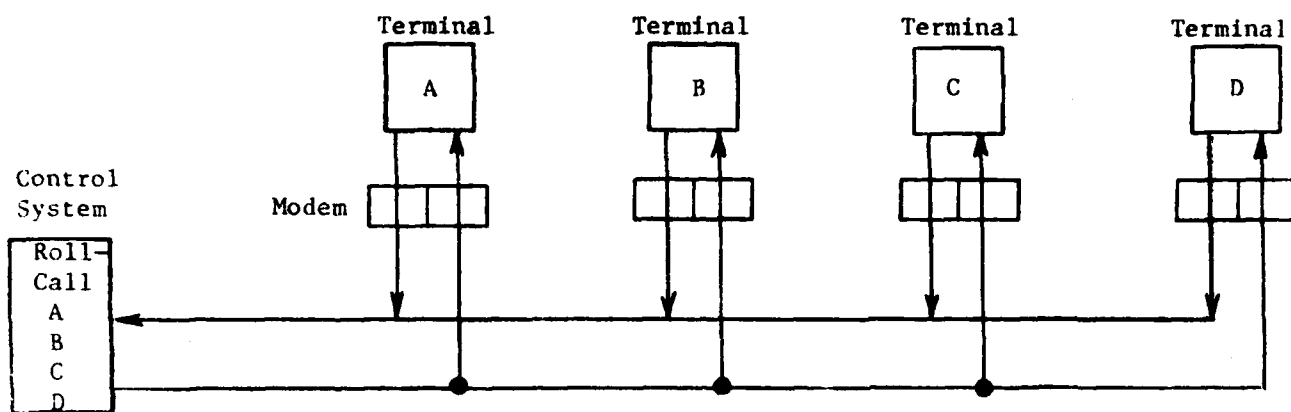
(a) Multidrop network
