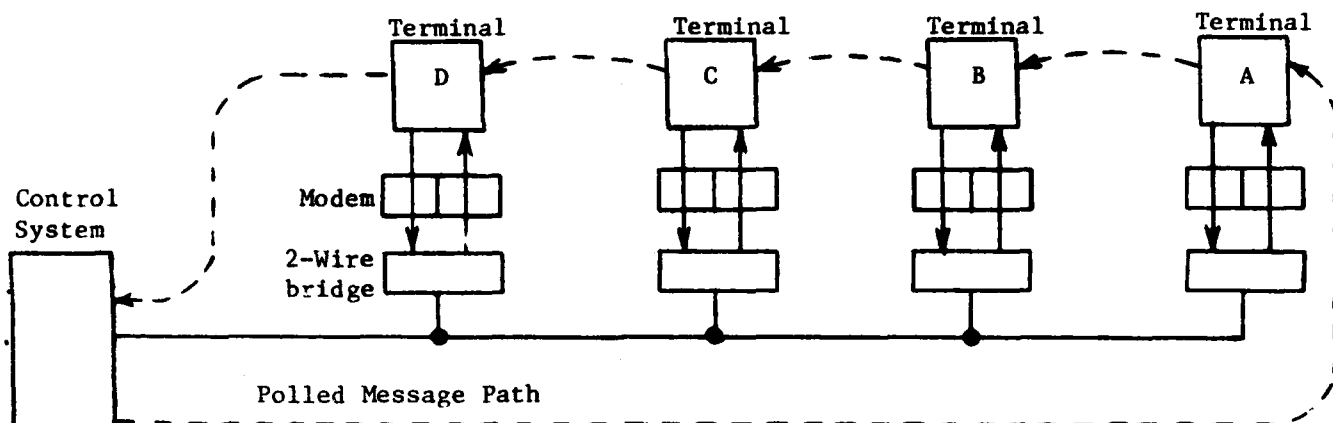
a) 2-wire network
