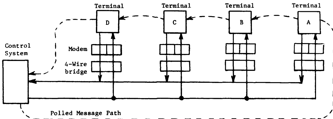
b) 4-wire network
