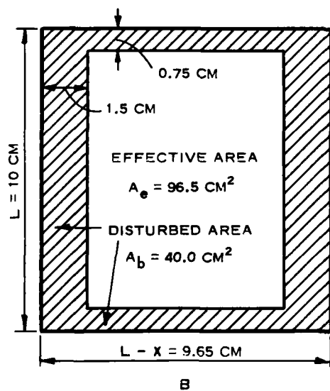
FIG. 14. INFLUENCE OF PROGRESSIVE FAILURE IN DIRECT SHEAR TESTS
