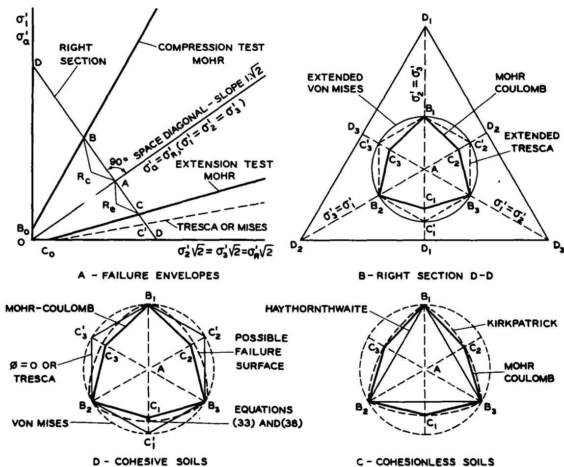
FIG. 40 - FAILURE SURFACES IN THE PRINCIPAL STRESS SPACE
