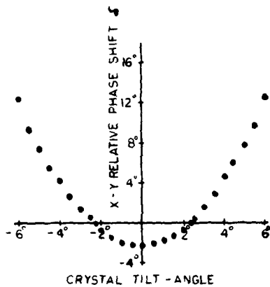
Fig. 1. Crystal tilt-angle versus X-Y phase anisotropy.
