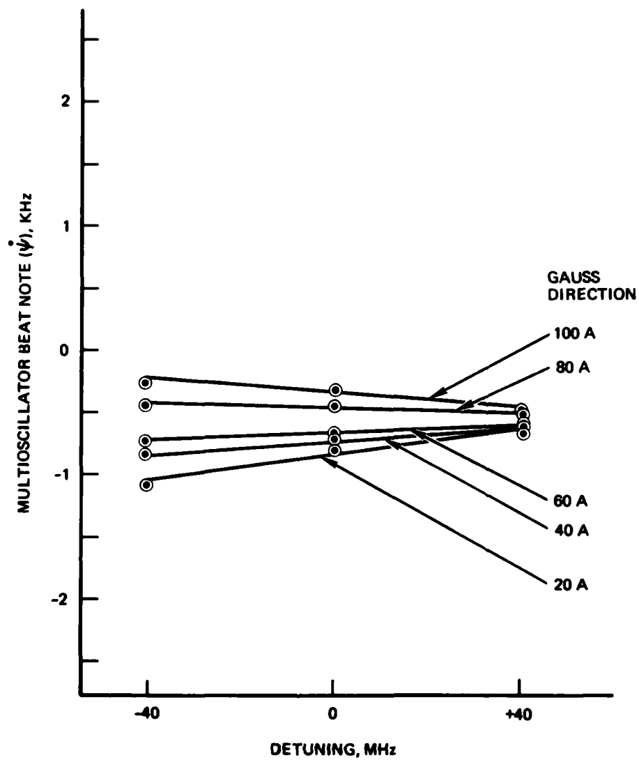
Figure 13b. \dot{\psi} versus Cavity Length Tuning in a Zeeman Multioscillator
