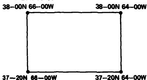
FIGURE 2-22 Corner Method
