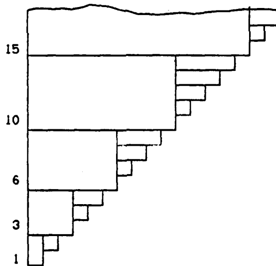
Figure 3.4. The triangular transform.
