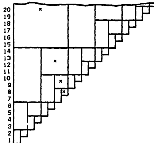
Figure 5.1. The online binary transform.
