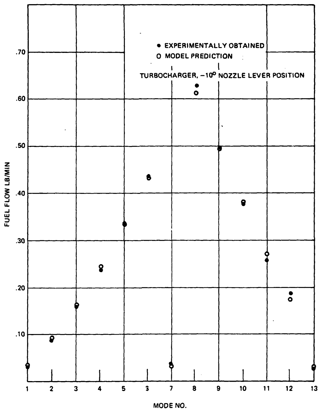
FIGURE 19 - COMPARISON OF MODEL PREDICTIONS WITH THOSE OF EXPERIMENTALLY OBTAINED FUEL FLOW RATES. JOHN DEERE, MODEL 4239T, WITH AERODYNE TURBOCHARGER, -10^{\circ} NOZZLE LEVER POSITION
