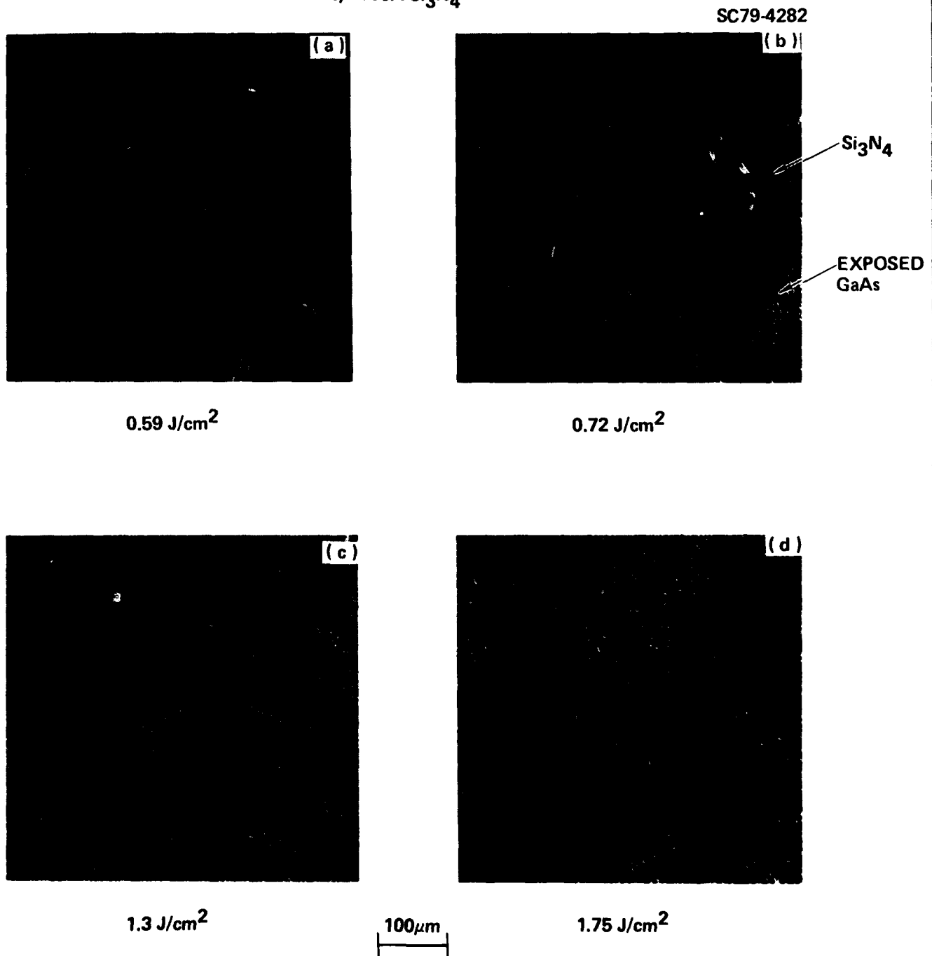
Fig. 4 Surface morphology of semi-insulating GaAs samples coated with ~1000Å \text{Si}_3\text{N}_4 film after irradiation with a ruby laser pulse of energy density: (a) 0.59 J/cm 2 , (b) 0.72 J/cm 2 , (c) 1.3 J/cm 2 , and (d) 1.75 J/cm 2 . All samples were implanted with 300 keV, 1 \times 10^{15} \text{ cm}^{-2} Si + ions at room temperature prior to \text{Si}_3\text{N}_4 coating and laser irradiation.
