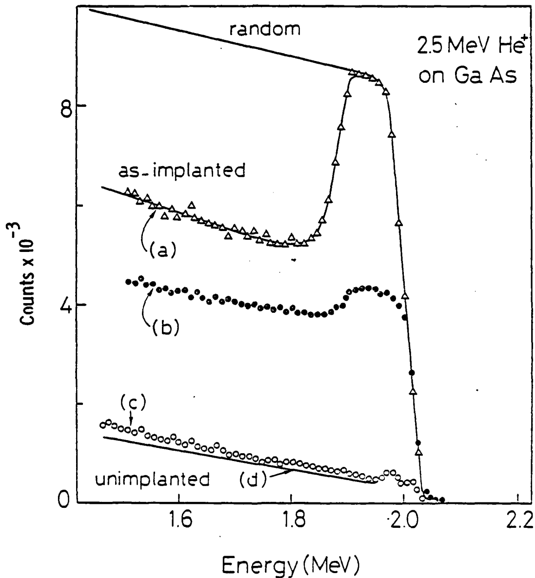
Fig. 5 Backscattering spectra of 2.5 MeV \text{He}^+ ions incident in a random direction and in \langle 100 \rangle direction of GaAs samples implanted with 400 keV Te ( 10^{15} \text{ cm}^{-2} ), after laser irradiation of energy (a) 0.2 to 0.8 \text{J/cm}^2 , (b) 0.9 \text{J/cm}^2 , (c) 1.0 to 1.4 \text{J/cm}^2 . The curve (d) is obtained from unimplanted \langle 100 \rangle GaAs sample.
