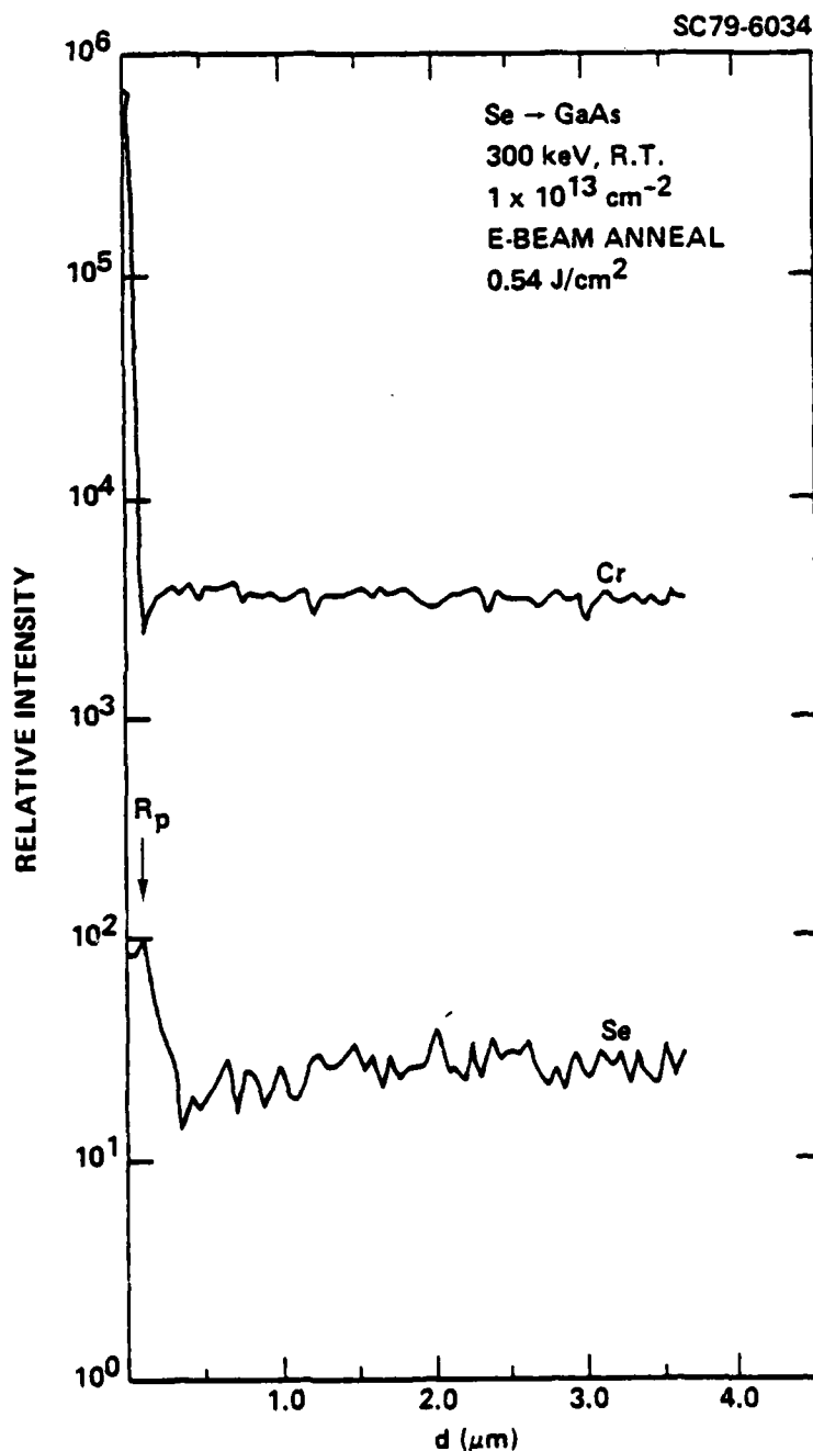
Fig. 16 Depth distributions of Se and Cr atomic concentrations measured by SIMS in a semi-insulating GaAs sample irradiated with an electron beam pulse of 0.54 \text{ J/cm}^2 . The sample was implanted at room temperature with 300 keV \text{Se}^+ ions to a dose of 10^{13} \text{ cm}^{-2} prior to electron beam irradiation.
