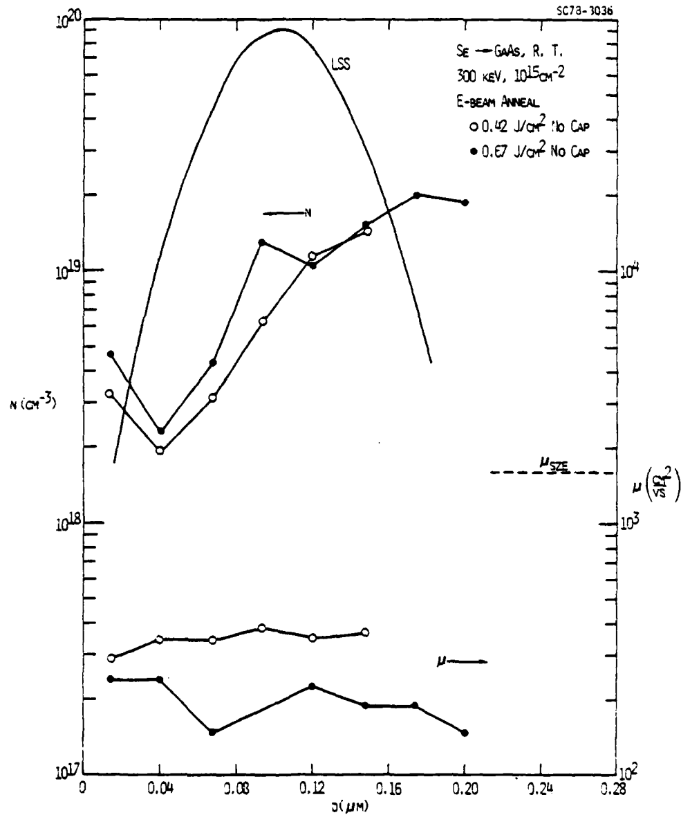
Fig. 14 Electron concentration ( n ) and mobility ( \mu ) vs depth ( d ) profiles of two electron beam annealed samples, one with a pulse of 0.42 \text{ J/cm}^2 (○) and the other with a pulse of 0.67 \text{ J/cm}^2 (●). Both samples were implanted with 300 keV, 1 \times 10^{15} \text{ Se}^+ ions/cm at room temperature prior to electron beam exposure. The dotted line ( \mu_{SE} ) represents the estimated value of mobility 10 for the peak electron concentration measured in the n -profile.
