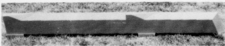
FIGURE 7* - Photograph of Simplified Sidewall With a Fairing at the Transom and at 50% Length Forward of the Transom
