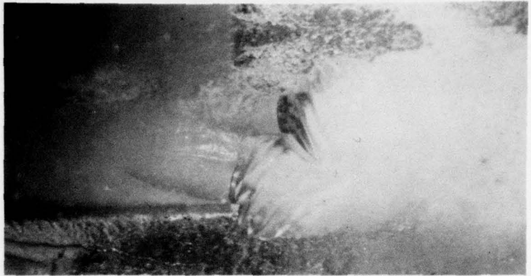
FIGURE 15 - Photograph of Propellers 4407 and 4704 Operating Near Hump (Viewed From Beneath)
