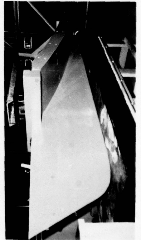
FIGURE 13 - Fitting Room Photographs for Model 5353 Fitted With Propellers 4703 and 4704 and With Curved Planing Surface to Simulate the Aft Seal of a Surface Effects Ship
