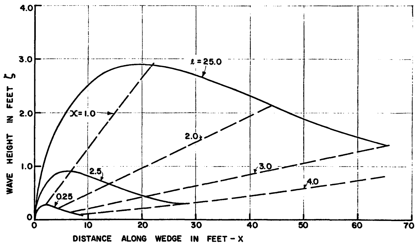
Figure III.5. Spray Sheet Surface Elevation from Equation III.12.
