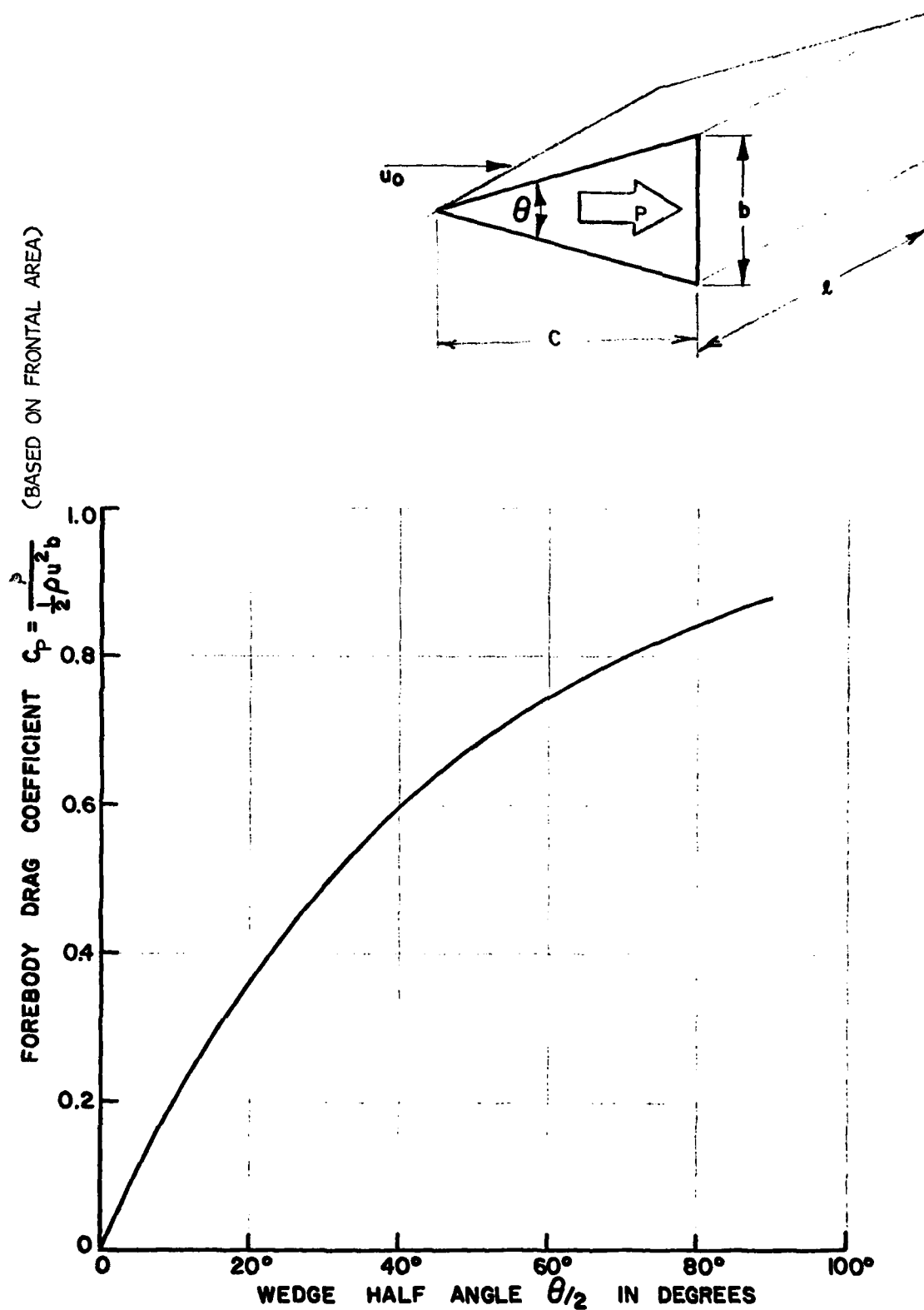
Figure III.1. The Drag Force Acting on the Forward Faces of a Wedge in Two Dimensional Inviscid Flow.
