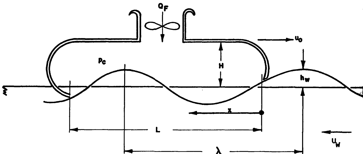
Figure 2. Basic Geometry.
