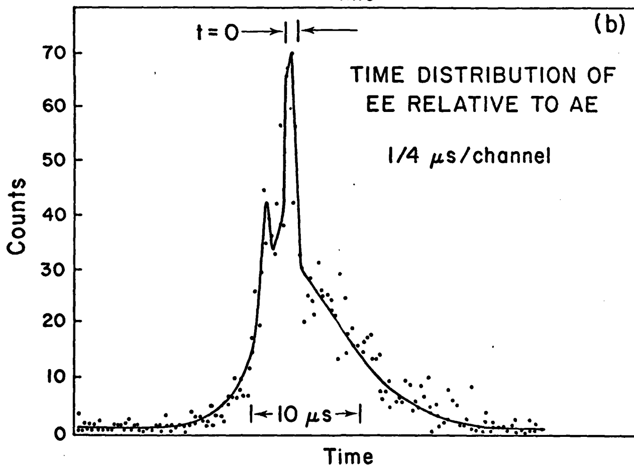
Fig. 9. a. Distribution of EE in time relative to AE at 1 \mu\text{s}/\text{channel} . The t = 0 point is shown to be uncertain by \pm 0.5 \mu\text{s} . b. Data similar to Fig. 9a taken at 1/4 \mu\text{s}/\text{channel} .
