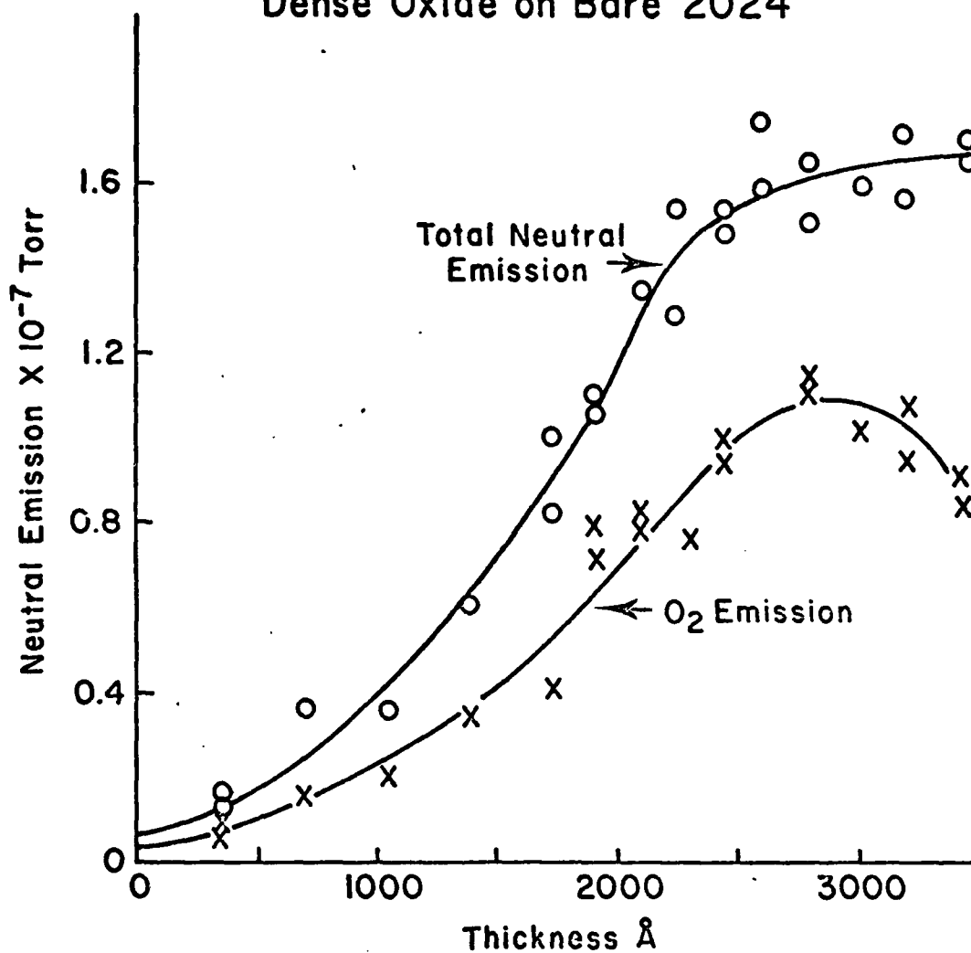
Fig. 4. Neutral emission intensity versus thickness for a dense oxide on bare Al 2024. xxx: peak heights of \text{O}_2 emission, ooo: peak heights of the total emission curves.
