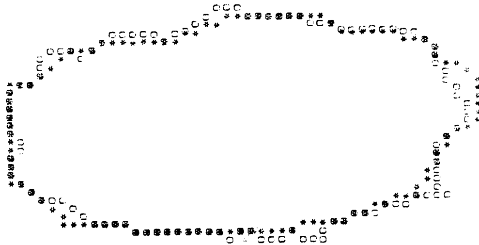
Figure 12b - True (O) and estimated (*) boundaries for distorted ellipse using Kalman filter algorithm and incorrect model parameters.
