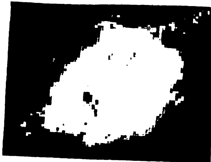
Figure 10e - Satellite Image of a Cloud.
