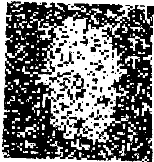
Figure 10b - Distorted Ellipse, \Delta/\sigma=1 .
