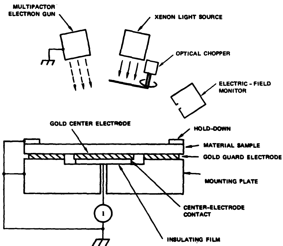
FIGURE 1 SETUP FOR MATERIALS CHARGING TESTS
