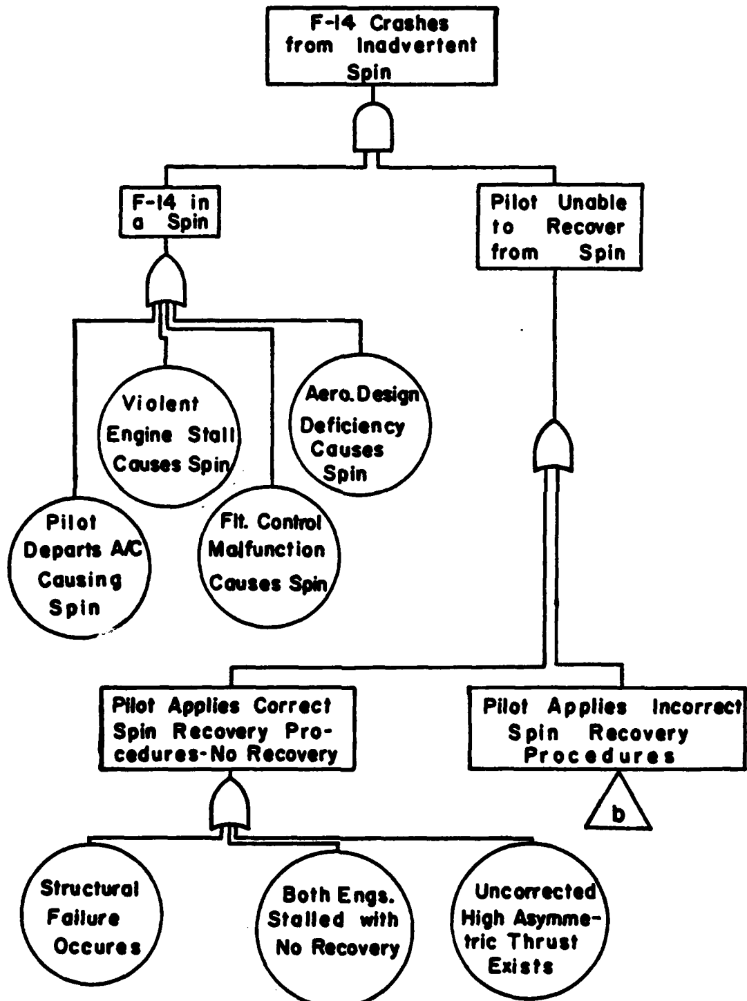
FIGURE I. FAULT TREE ANALYSIS CHART
