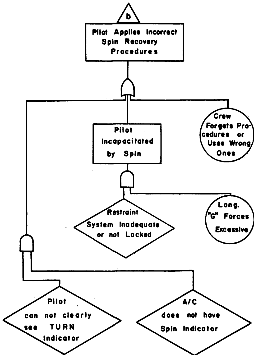
FIGURE 1. FAULT TREE ANALYSIS CHART
