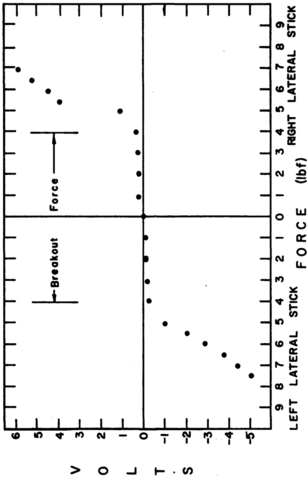
FIGURE 12. OUTPUT VOLTAGE VS. LATERAL STICK FORCE
