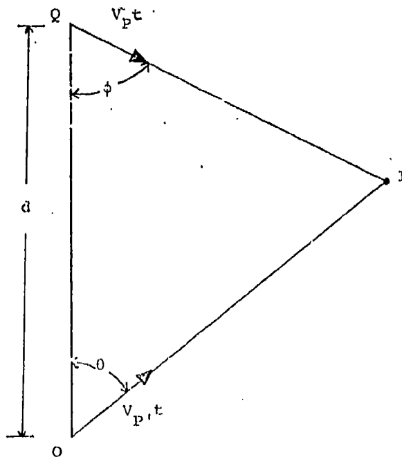
Geometry For Constant Bearing Intercept
