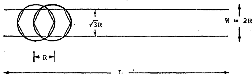
Sprint-Drift Search
