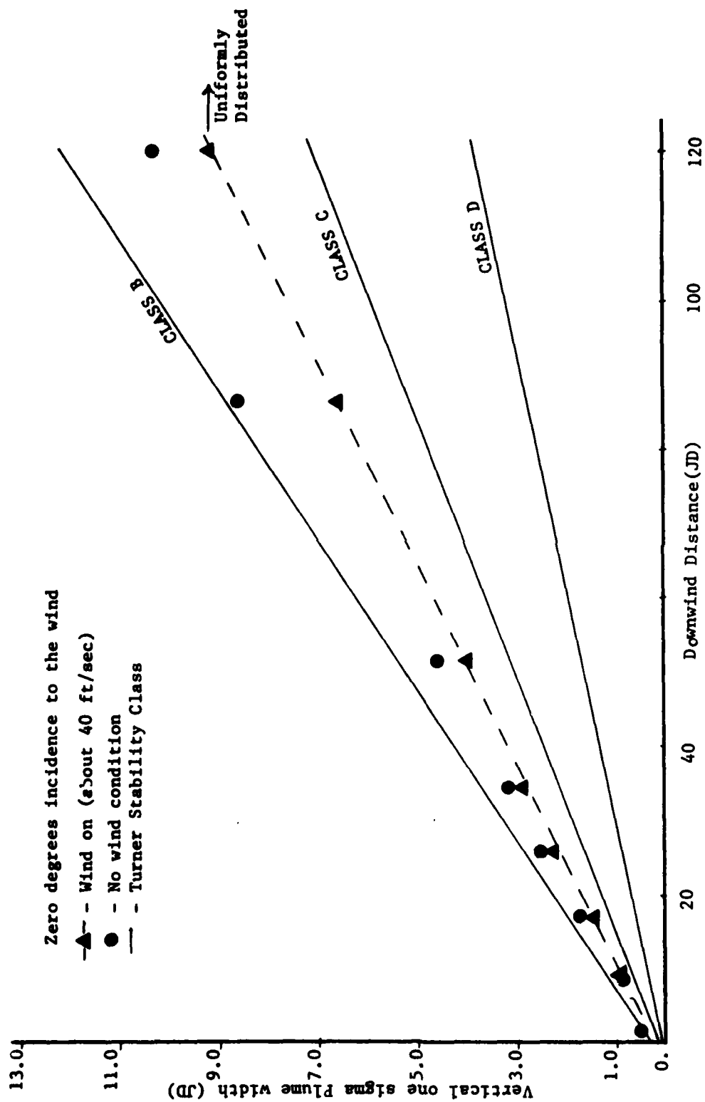
Figure 36 Vertical Plume Width vs. Downwind Distance
