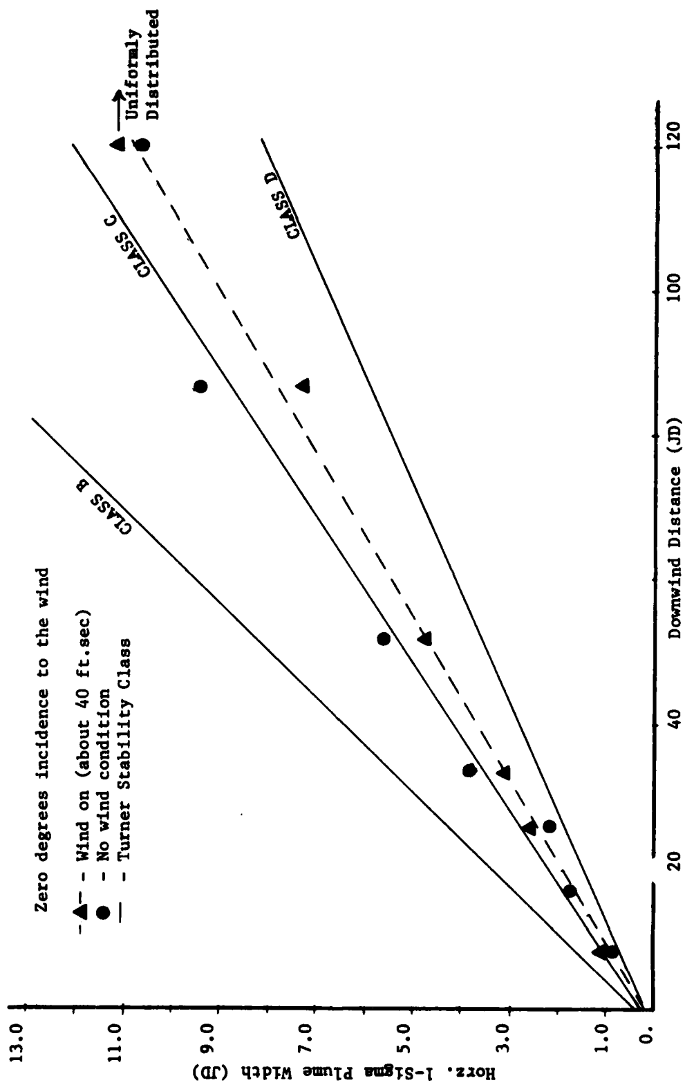
Figure 35 Horizontal Plume Width vs. Downwind Distance
