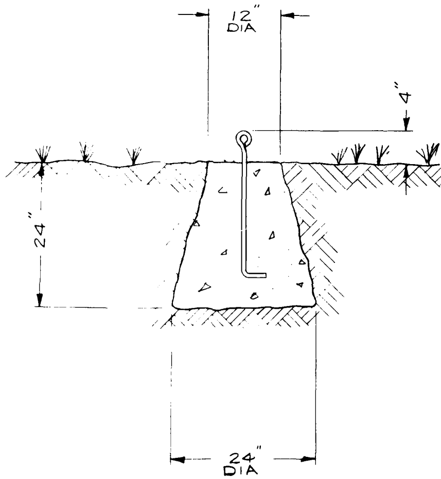
TYPICAL ANCHOR ROD INSTALLATION
