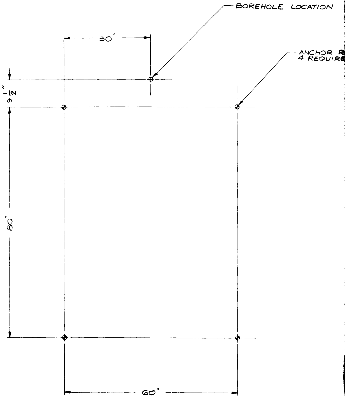
ANCHOR ROD PLACEMENT FOR DRILL RIG TIE DOWNS
