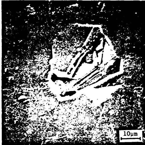
a) Transgranular Microfracture, T = 23°C
