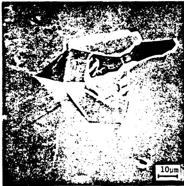
b) Intergranular Microfracture, T = 1000°C
