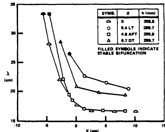
Fig. 16 Location of bifurcation point, M = 1.43 , Re_L = 9 \times 10^6 .
