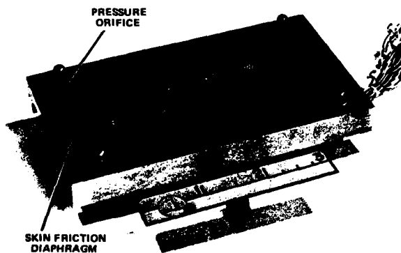
Fig. 4 Skin friction survey plate.
