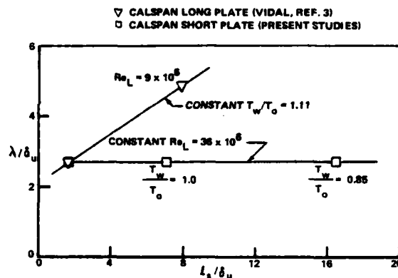
Fig. 20 Re_L and T_w/T_0 effects on interaction lengths, M \sim 1.43 .
