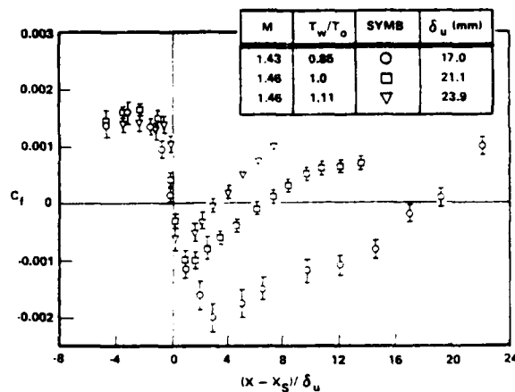
Fig. 11 Heat transfer effect on skin friction distribution, Re_L = 36 \times 10^6 .
