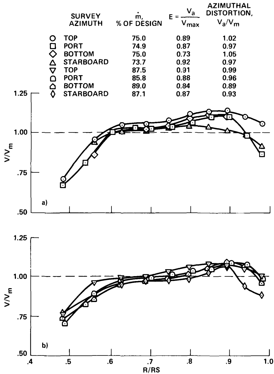
(a) \dot{m} \approx 75\% (b) \dot{m} \approx 85\%
