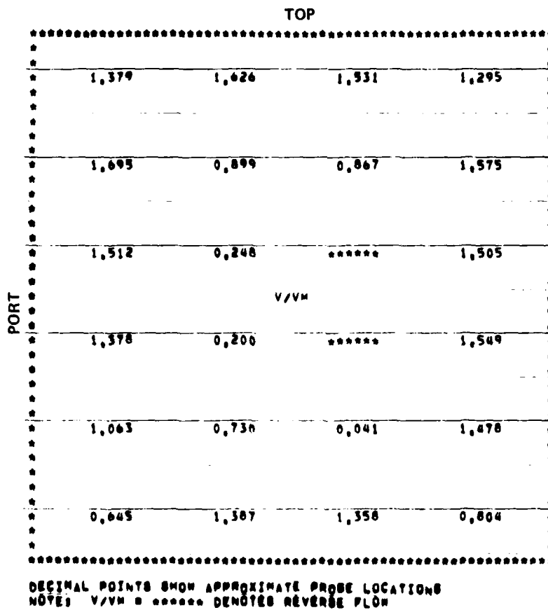
(a) Type A distortion at \dot{m} \approx 90\% .
