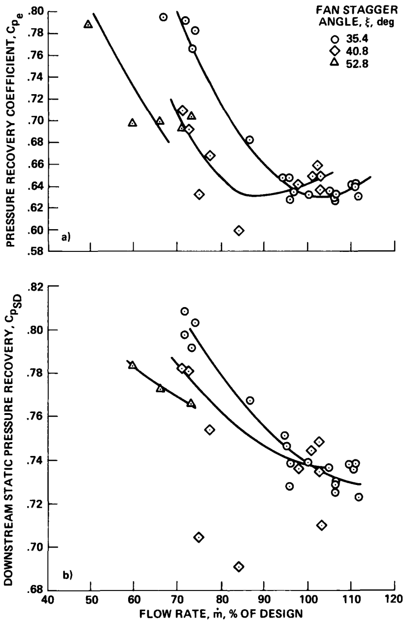
(a) Static pressure recovery coefficient near exit plane. (b) Static pressure recovery in settling duct.
