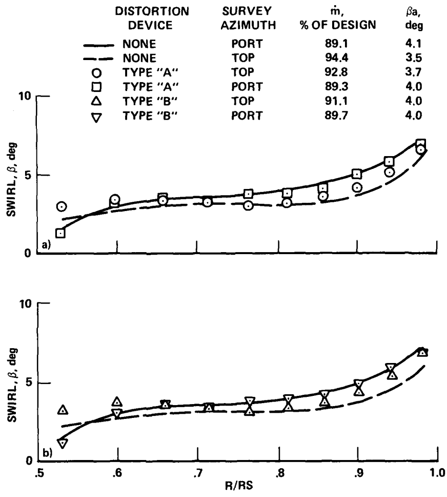
(a) Type A distortion. (b) Type B distortion.
