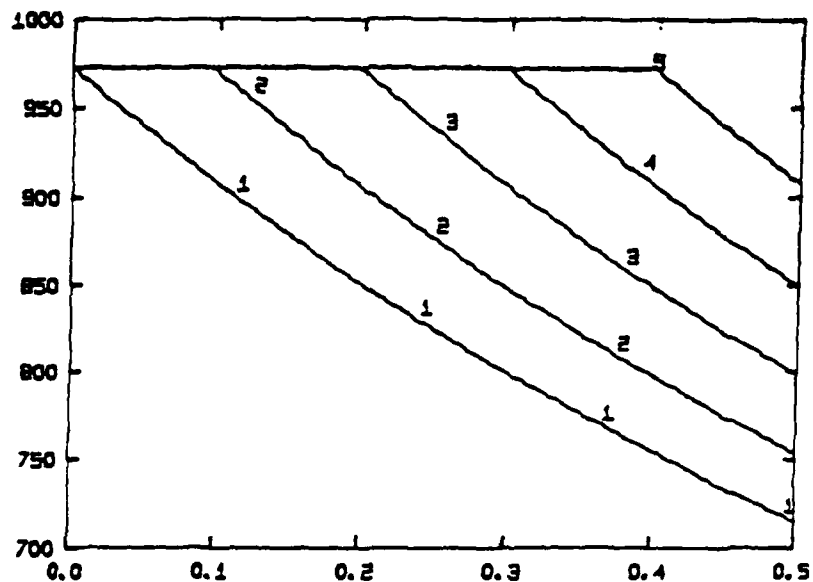
Figure 16. The temperature profile within 0.2 atm \text{SiH}_4 at various times after exposure to the laser beam. The times are: (1) 41 msec, (2) 43.2 msec, (3) 45.7 msec, (4) 48.1 msec, (5) 50.6 msec, after the laser beam is switched on. The beam intensity is 8 \text{ w/cm}^2 and the product q_p is assumed to be constant and equal to 0.6 \text{ cm}^{-1} .
