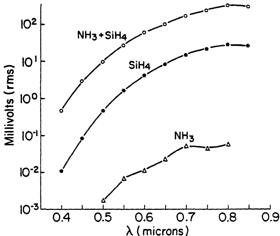
Figure 20. Emission spectra from reaction flame measured with a 1/4 meter Jarrell-Ash monochrometer. Cell pressure was 0.2 atm and gas flow rates for \text{SiH}_4 were 11 \text{cm}^3/\text{min} and \text{NH}_3 were 110 \text{cm}^3/\text{min} . Measurements were made only at the discrete wavelengths indicated in the figure. Millivolt output from PM tube amplifier was corrected for sensitivity of PM tube at a particular wavelength. Thus values are proportional to intensity.
