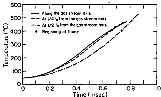
Figure 25. The calculated temperatures of volume elements of reactant gas after they enter the laser beam at time = 0. All volume elements lie in plane m of Figure 24 and r_o is the radius of the gas stream. The times corresponding to the points designated as the beginning of the flame were calculated from the measured distance to the flame as given in Figure 19 and the calculated velocity of the particular elements in the reactant gas stream. Reference flow conditions are assumed.
