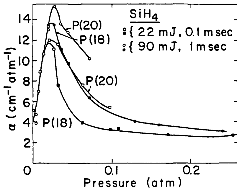
Figure 6. The absorption coefficients of SiH 4 as a function of pressure for the P(18) and P(20) CO 2 laser lines.
