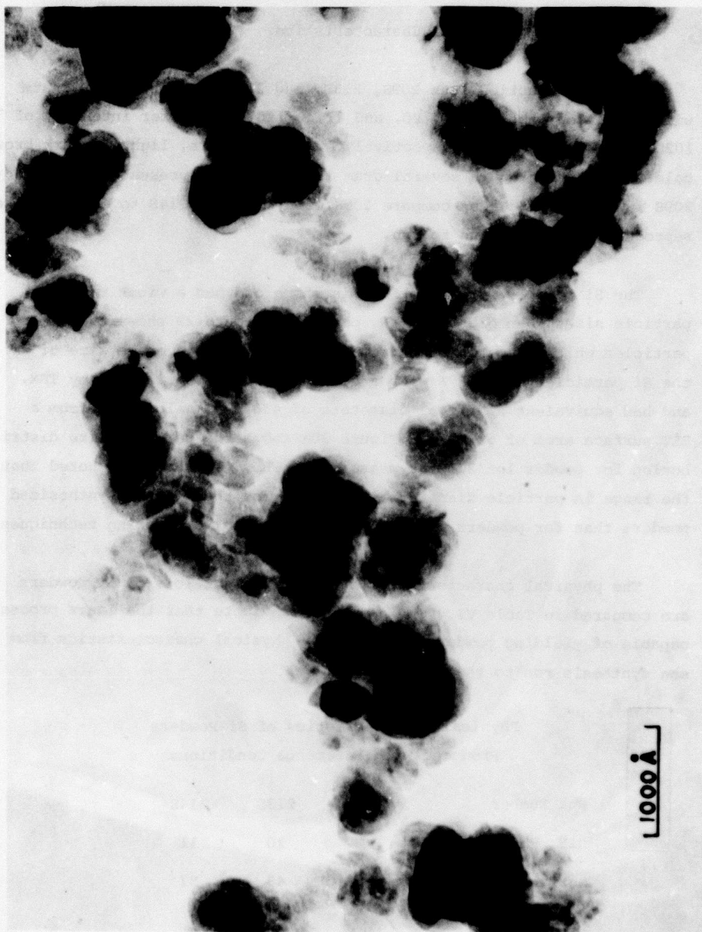
Figure 29. TEM photograph of Si powders from lot 209S.
