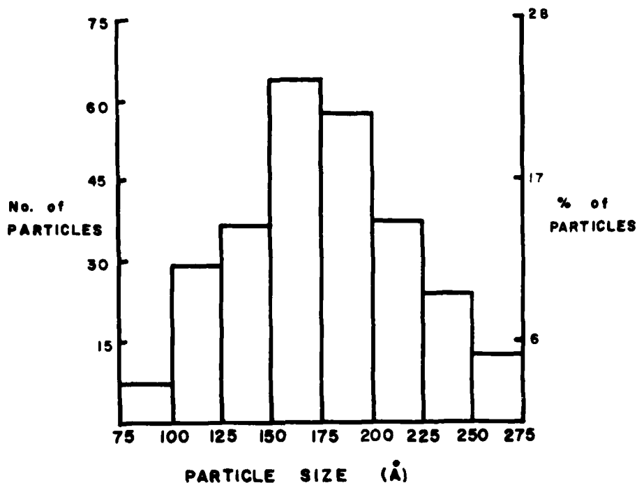
Figure 33. Particle Size Distribution Of 603SN Si 3 N 4 Powder.
