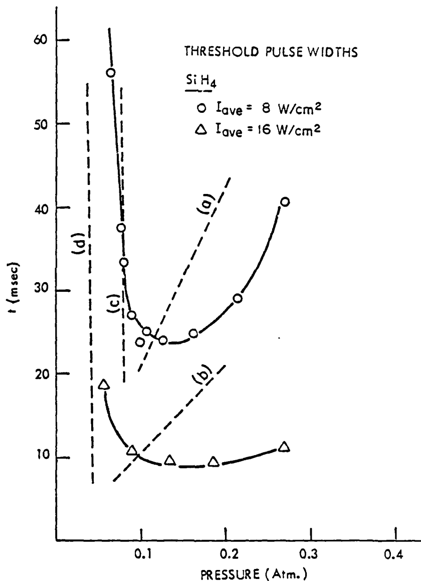
Figure 13. Threshold pulse-lengths which result in the formation of Si powder from \text{SiH}_4 as a function of pressure. Dotted lines a, b, c, and d are calculated thresholds equating the absorbed power to the sensible heat (a,c) and to the conductive losses (b,d). Lines a and c correspond to 8 \text{ W/cm}^2 and b and d correspond to 16 \text{ W/cm}^2 .
