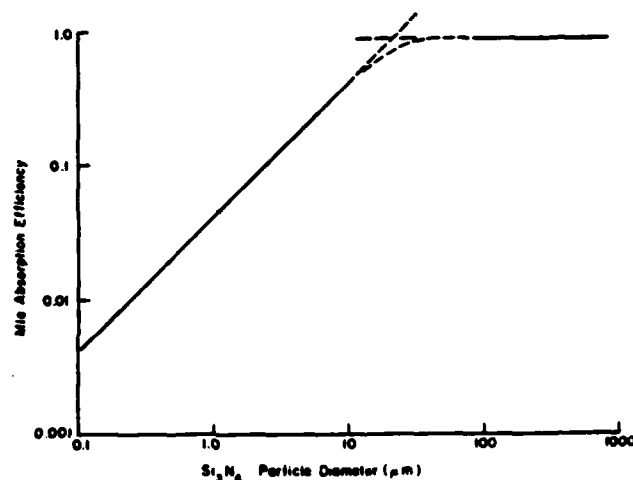
Figure 1. Mie absorption efficiency of Si_3N_4 particles to 10.6 \mu m light as a function of particle size.
