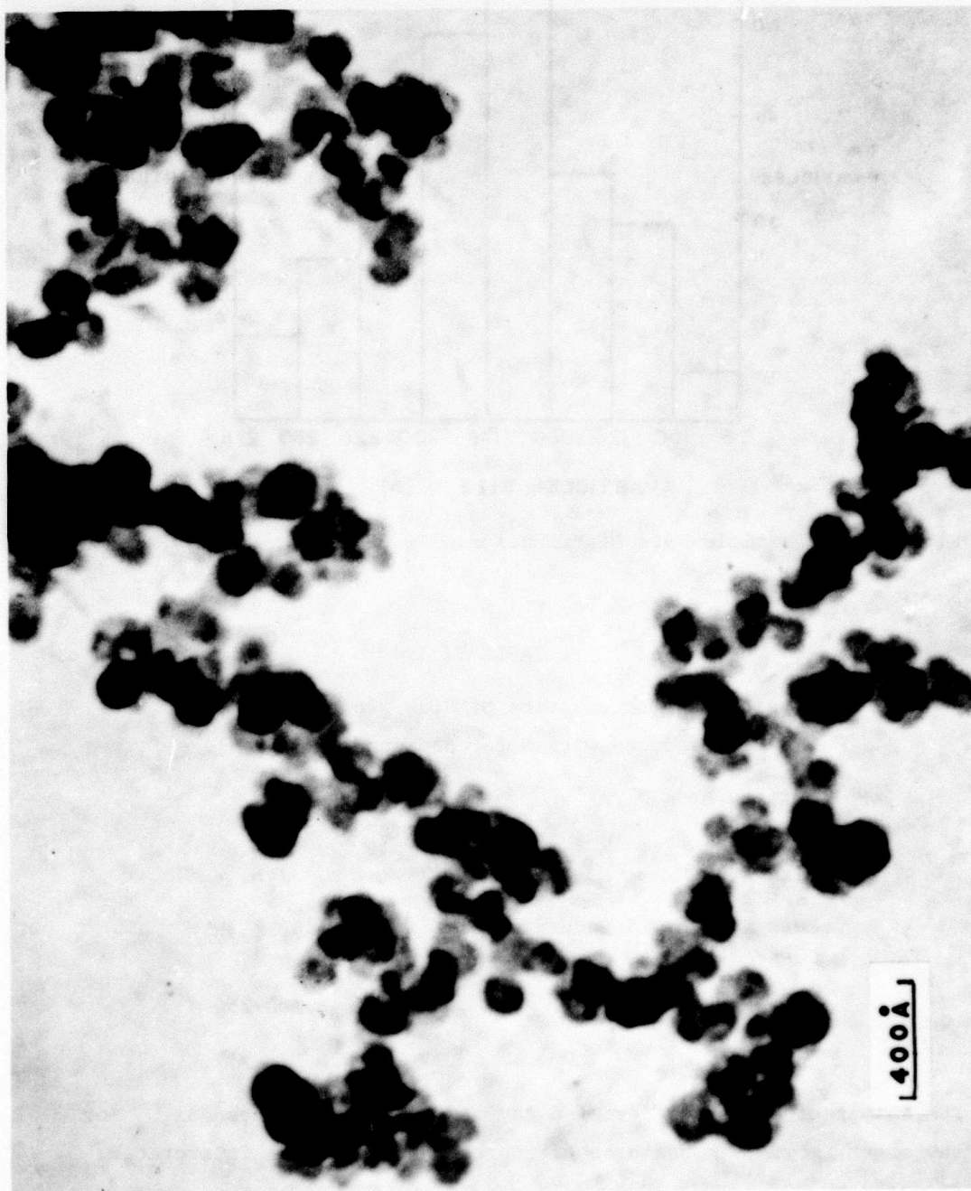
Figure 32. TEM photomicrograph of \text{Si}_3\text{N}_4 powders from lot 603SN.
