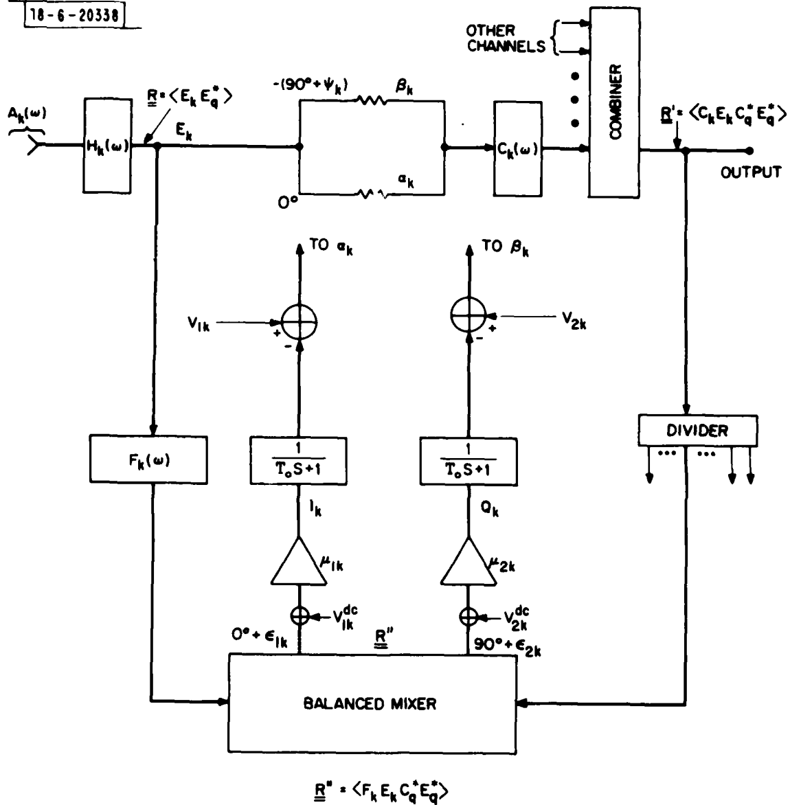
Fig. 11. Model of a wideband, analog feedback nulling processor including the effects of various component imperfections.
