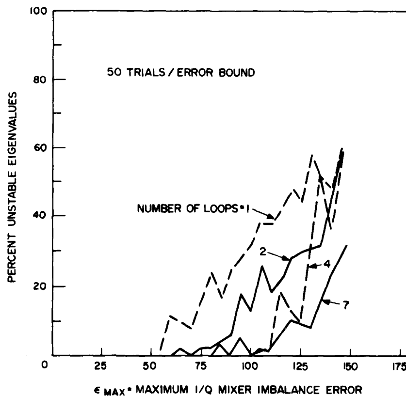
Fig. 15. Stability dependence as a function of I/Q mixer imbalance errors for 1, 2, 4 and 7 control loops. Antenna geometry used was 7-element hexagonal array having D/\lambda = 6.6 with a single interference source positioned at \theta = 4^\circ , \phi = 0^\circ . FBW = 0.
