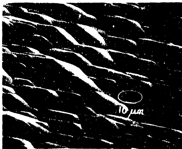
Figure 7 - Deeply Etched SC-cut Plate ( \text{NH}_4\text{F.HF} )
