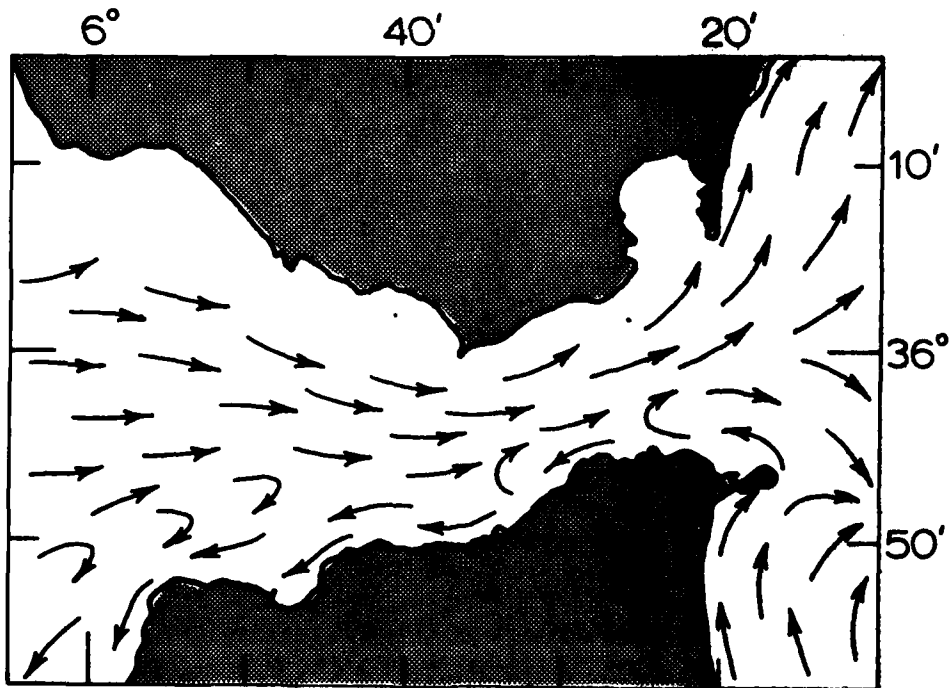
FIGURE 8. TIDAL CURRENTS IN STRAIT OF GIBRALTAR THREE HOURS AFTER HIGH WATER AT GIBRALTAR (SUBJECTIVE SUMMARY, N00 PUBL. 700).
