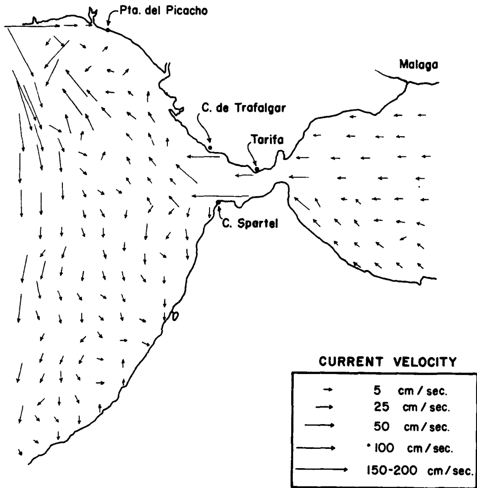
Figure 10 Currents (tidal and wind) in Bay of Gadiz at low water at Tarifa, computed with HN model (wind 6\text{m, sec}^{-1} from E).
