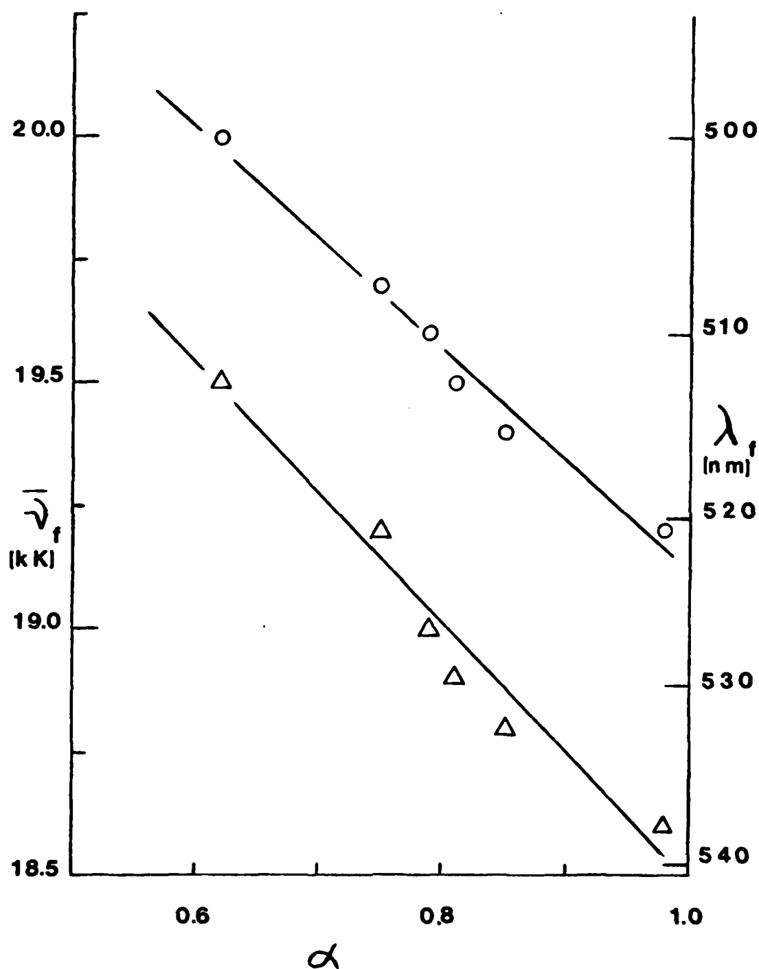
Figure 4. Correlation of fluorescence emission frequencies for C6F ( \Delta ) and C8F ( \circ ) with the solvent hydrogen bonding parameter, \alpha .
