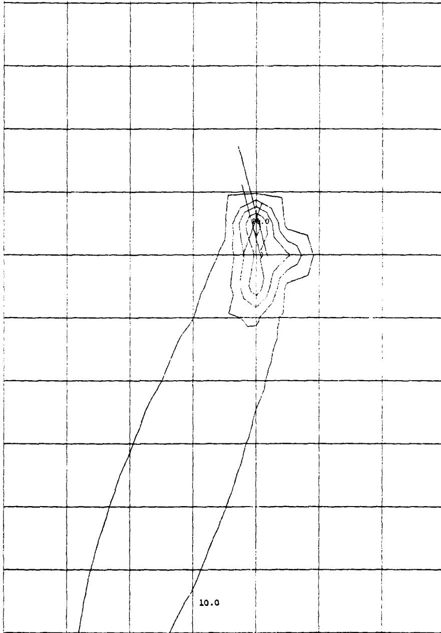
AIRCRAFT CO CONCENTRATION PROFILE (RUN NO. 1) (Scale = 20 \mu\text{g}/\text{m}^3 per contour)
