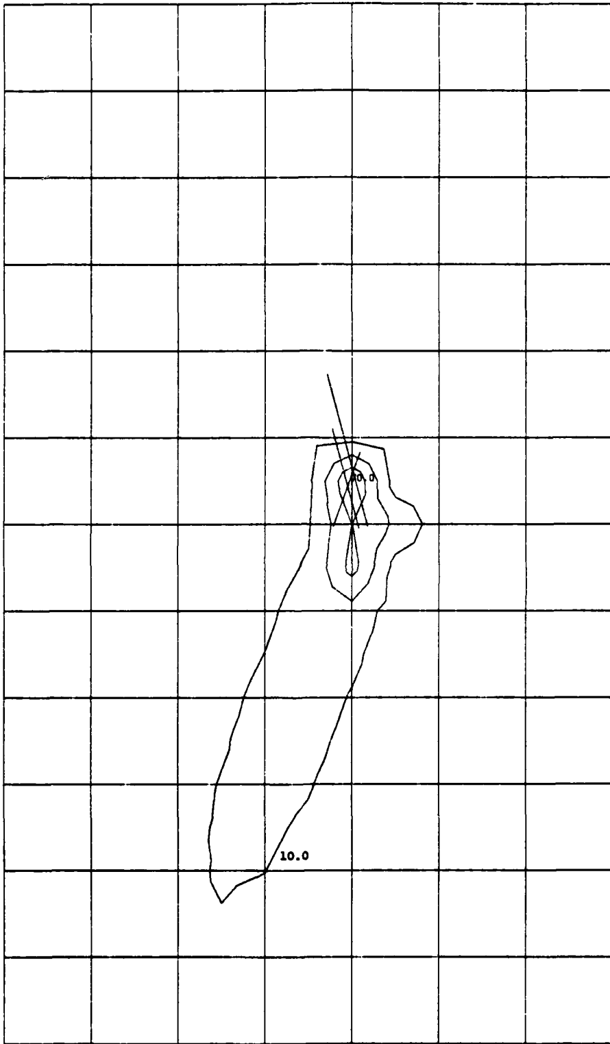
AIRCRAFT CO CONCENTRATION PROFILE (RUN NO. 7)
