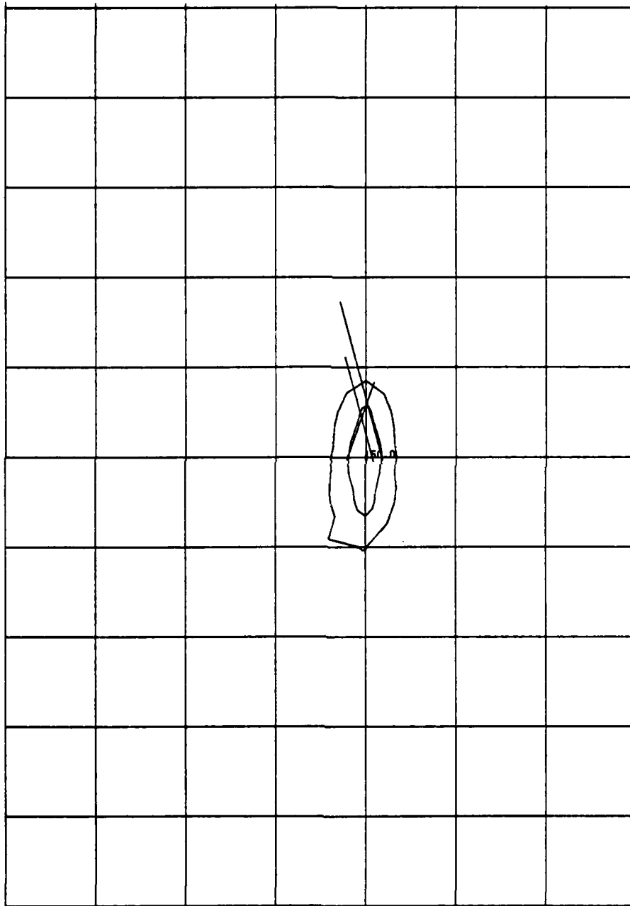
AIRCRAFT CO CONCENTRATION PROFILE (1 AUG 1300-1400) INCREMENTED FROM 50.0 (Scale = 50 \mu\text{gm}/\text{m}^3 per contour)
