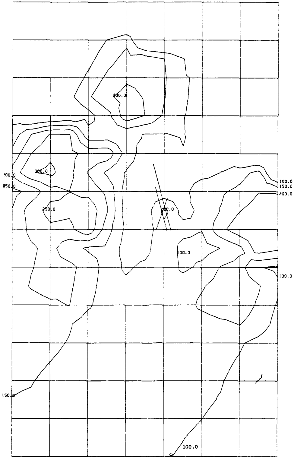
TOTAL CO CONCENTRATION PROFILE (RUN NO. 1) (Scale = 50 \mu\text{g}/\text{m}^3 per contour)
