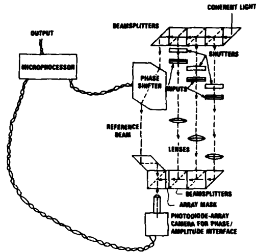
Figure 3. Multi-beam antenna controller.
