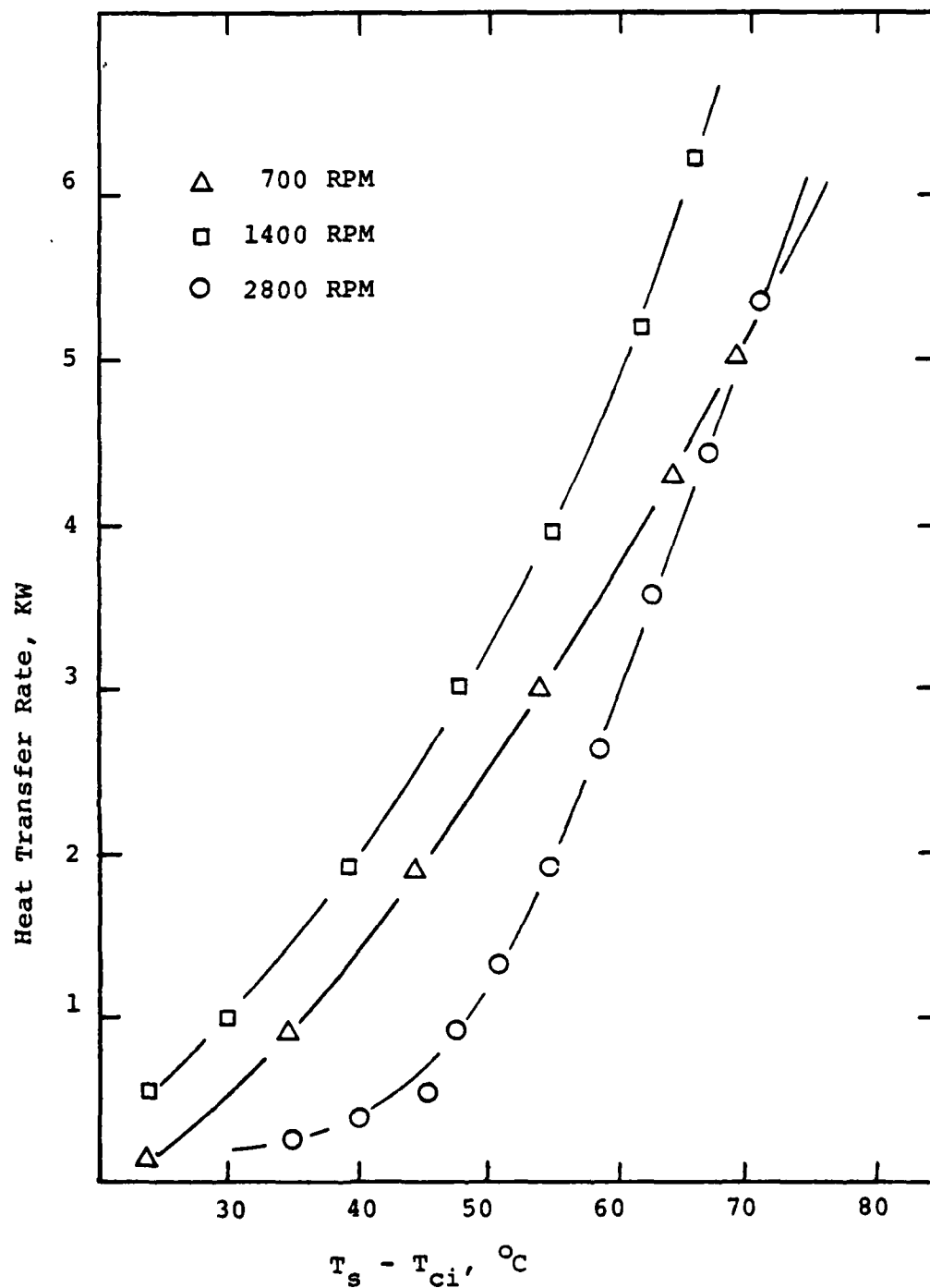
Figure 22. Heat Transfer Rate Versus Saturation Temperature Minus Water Inlet Temperature for Turbotec Tube and Distilled Water.
