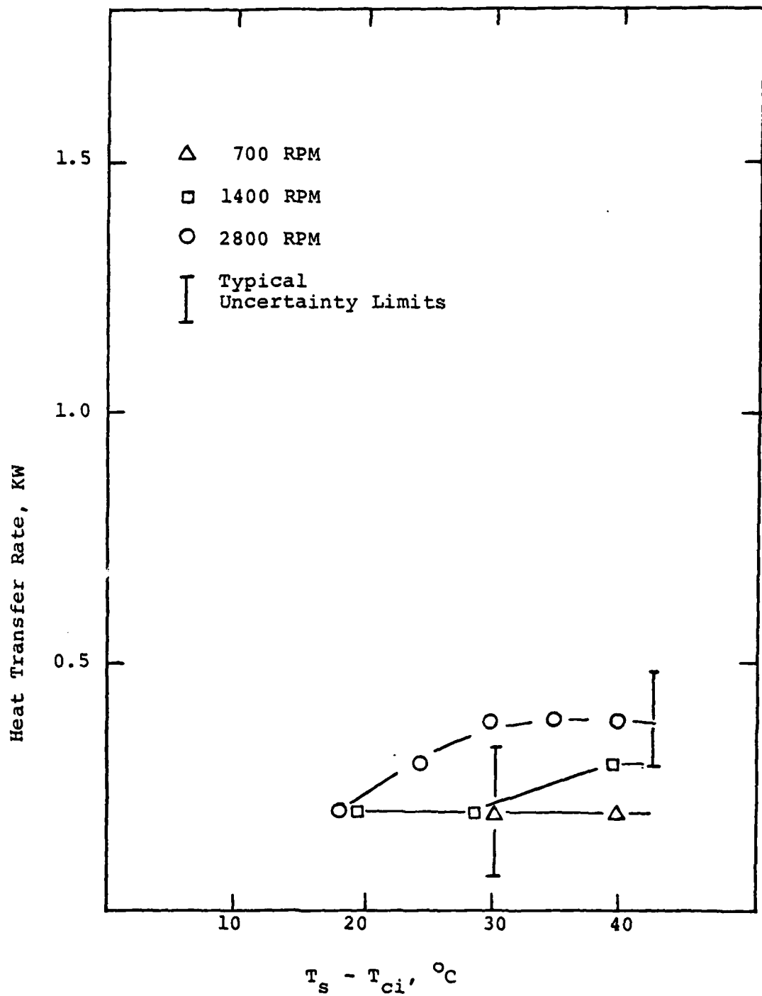
Figure 12. Heat Transfer Rate Versus Saturation Temperature Minus Water Inlet Temperature For Smooth Wall Cylinder and Freon 113.
