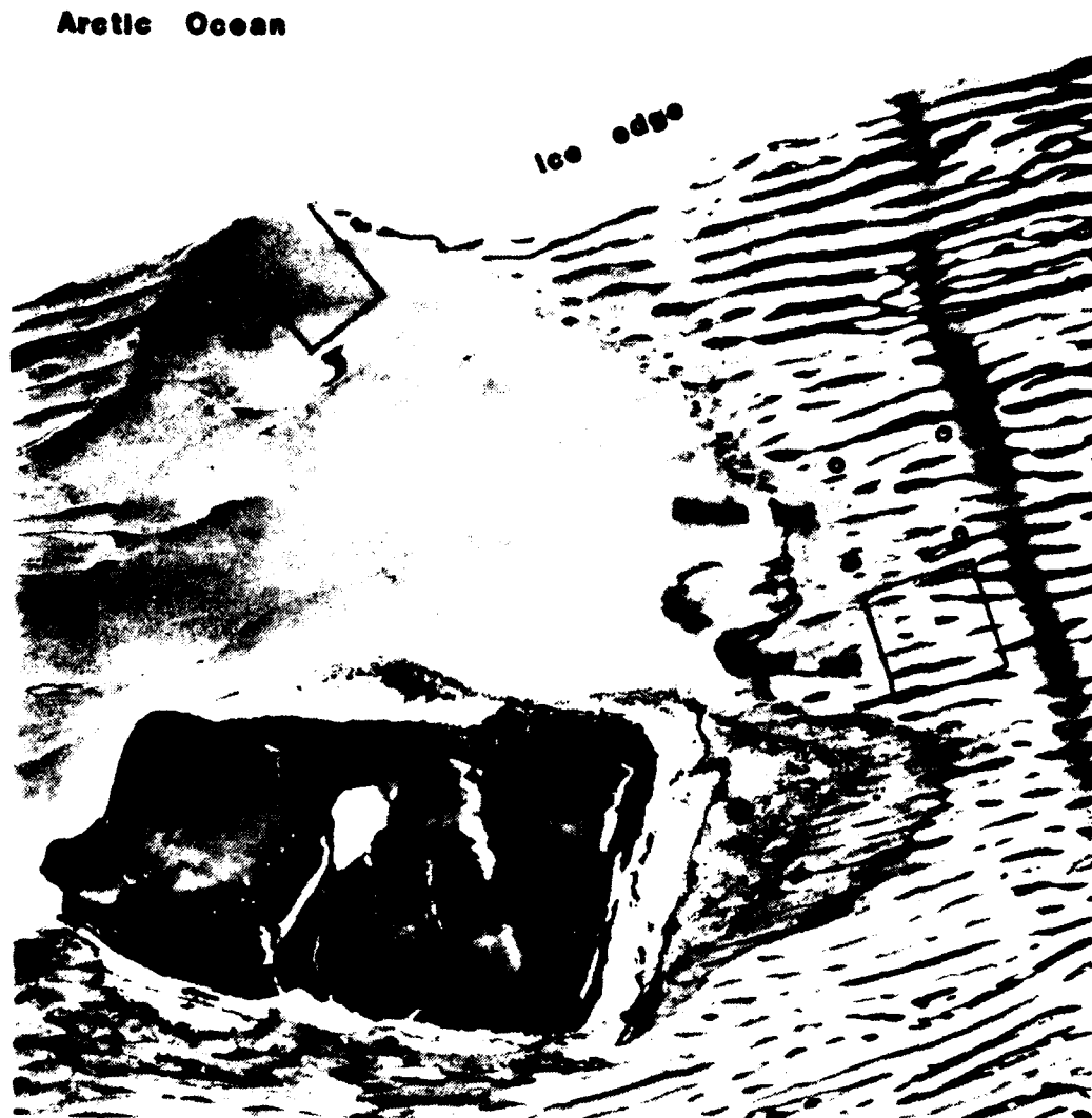
Ward Hunt Ice Shelf and ice rise showing ridge and trough structure relative to the location of the ablation nets
