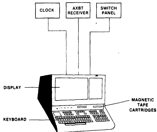
FIG. 2 FUNCTIONAL BLOCK DIAGRAM OF TERMINAL AXBT SYSTEM
