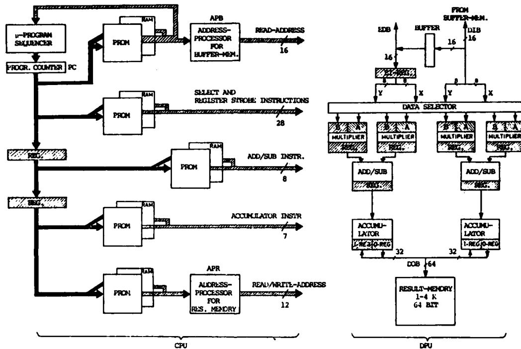
FIG. 1 CORRELATOR ARCHITECTURE
