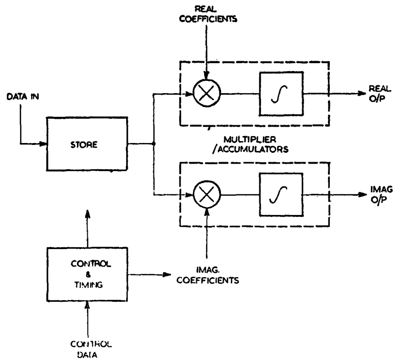
FIG. 6 PROCESSOR SCHEMATIC
