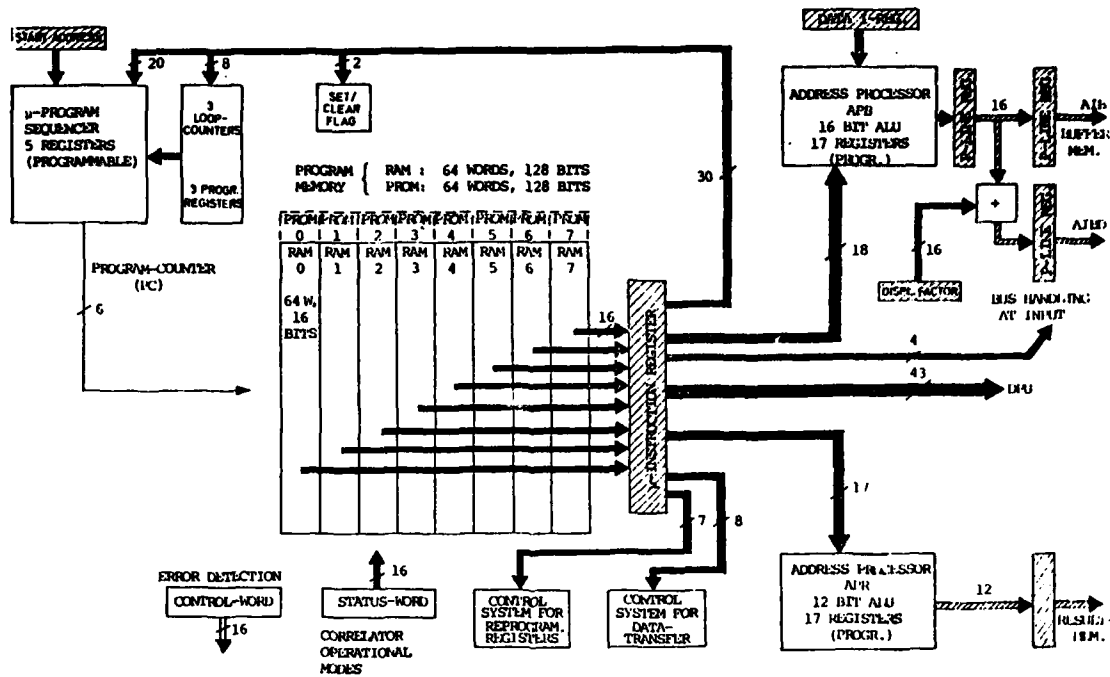
FIG. 3 BLOCK DIAGRAM OF CPU HARDWARE
