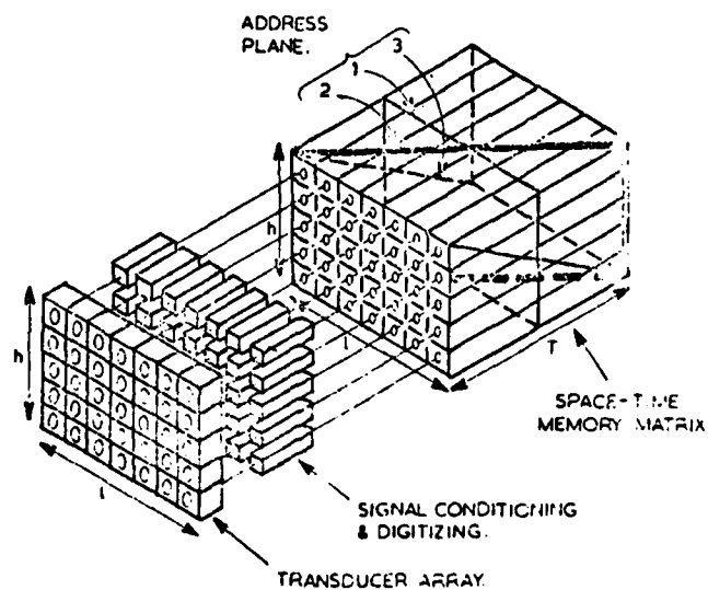
FIG. 3 SPACE TIME MATRIX BEAMFORMER
