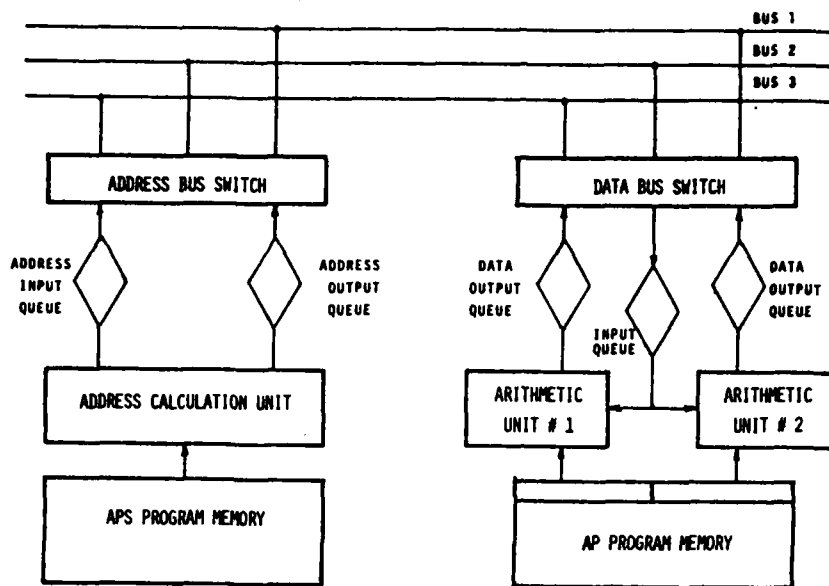
SIMPLIFIED DIAGRAM OF MAP300 ARITHMETIC UNIT
