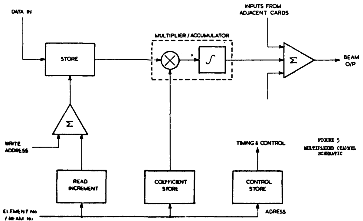
FIG. 5 MULTIPLEXED CHANNEL SCHEMATIC
