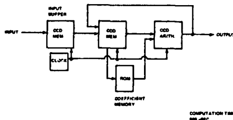
256 POINT FFT USING THREE CCD CHIPS PLUS A READ ONLY MEMORY (ROM) AND CLOCK
