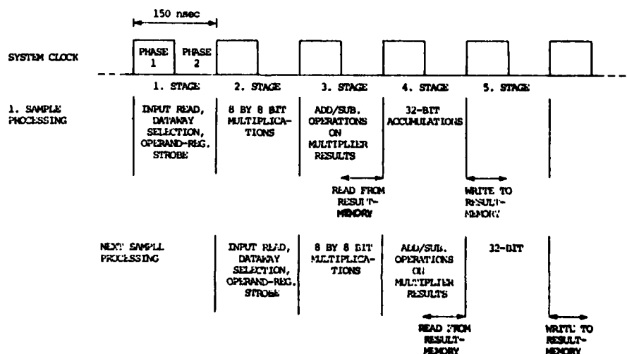
FIG. 2 TIME-SEQUENCED OPERATIONS OF THE DPU
