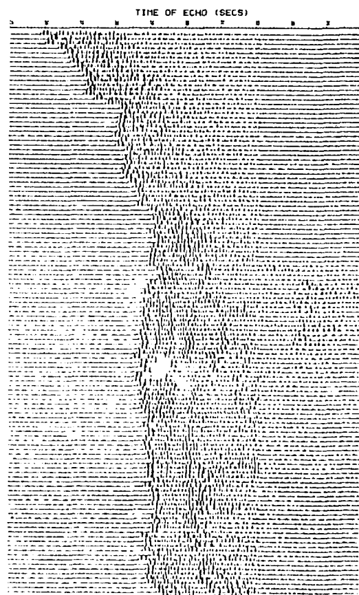
FIG. 4 TYPICAL "FILLED WIGGLE" DISPLAY FROM SUB-BOTTOM PROFILER
