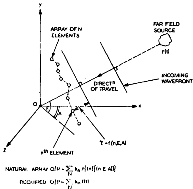
FIG. 1 THE BEAMFORMING PROBLEM
