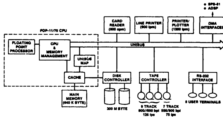
FIG. 5 HOST COMPUTER SUBSYSTEM
