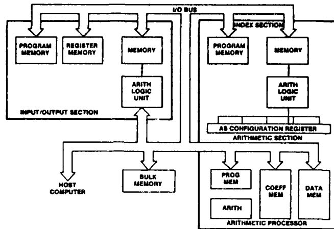
FIG. 4 SPS-81 ARCHITECTURE
