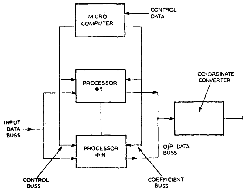
FIG. 7 SYSTEM ARCHITECTURE
