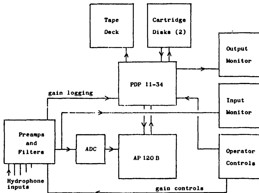
FIG. 1 BLOCK DIAGRAM OF SHIPBORNE PROCESSING SYSTEM
