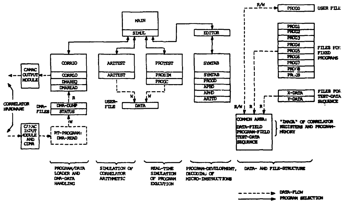
FIG. 4 CORRISIN STRUCTURE
