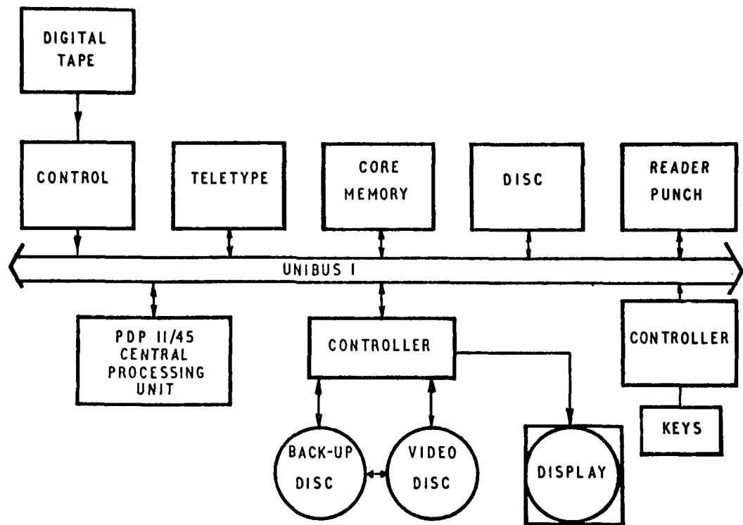
FIG. 5 DISC BASED DISPLAY SYSTEM
