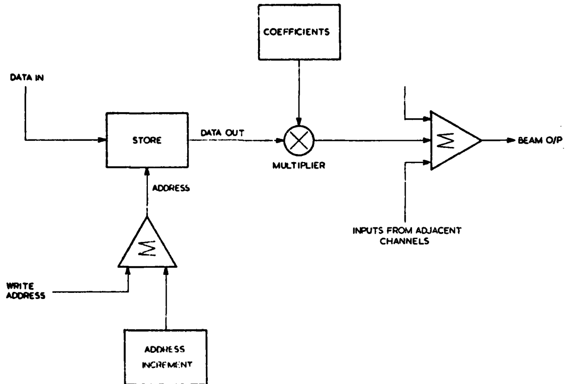
FIG. 4 BEAMFORMER CHANNEL SCHEMATIC
