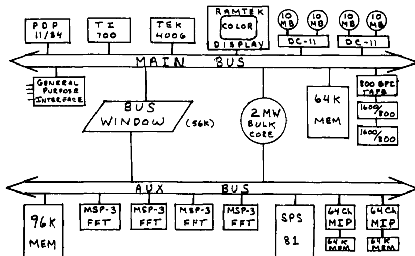
FIG. 4 SYSTEM CONFIGURATION FOR JUNE 1979
