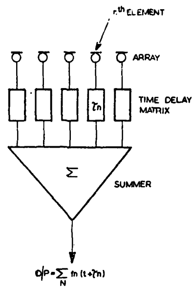
FIG. 2 BLOCK SCHEMATIC OF CONVENTIONAL TIME DELAY BEAMFORMER
