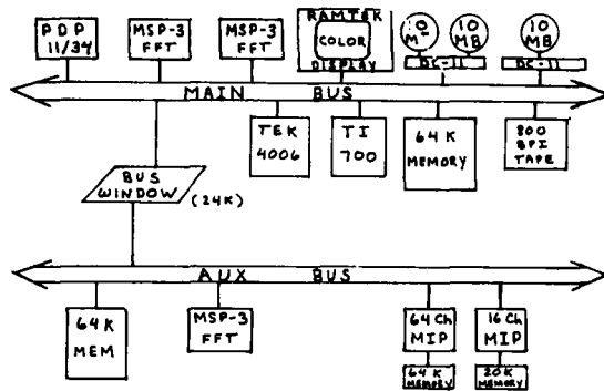
FIG. 2 SYSTEM CONFIGURATION FOR FEBRUARY 1979
