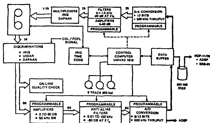
FIG. 2 ANALOG PREPROCESSOR SUBSYSTEM
