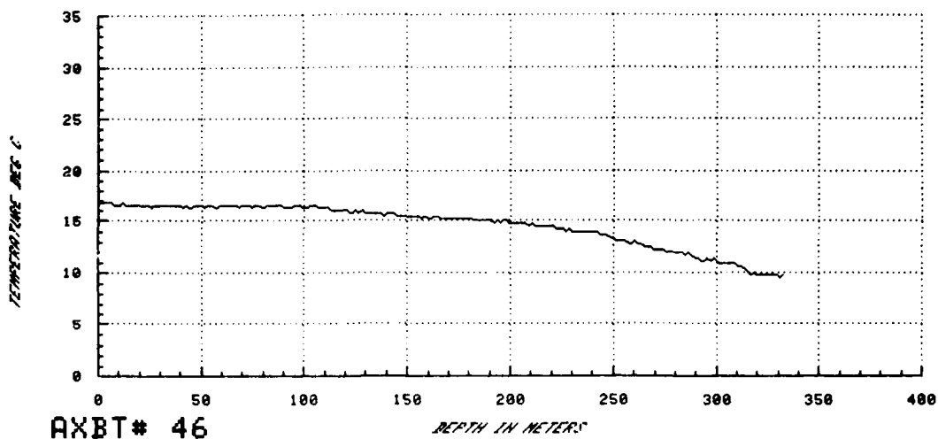
FIG. 3 AXBT PLOT PRODUCED ABOARD NRL AIRCRAFT
