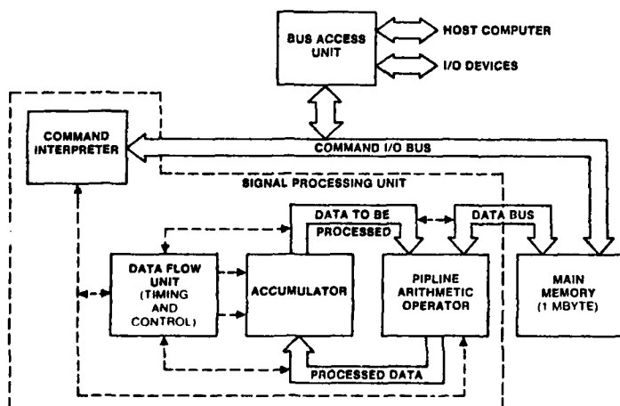
FIG. 3 RAYTHEON ADSP ARCHITECTURE
