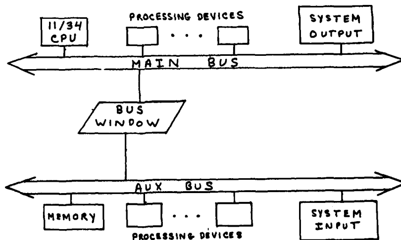
FIG. 1 BASIC SYSTEM ARCHITECTURE
