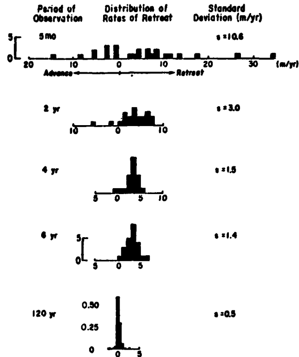
Figure 14. Distributions of measured retreat rates. Note the spread in the rates of shoreline change decrease as the period of observation lengthens. The histogram of 120-year rates is not strictly comparable to the others as it is based on a larger number of observations and includes effects of variations encountered around the entire perimeter of the lake (Powers, 1958); however, it still illustrates a continued reduction in the spread of retreat rates as the time interval lengthens.
