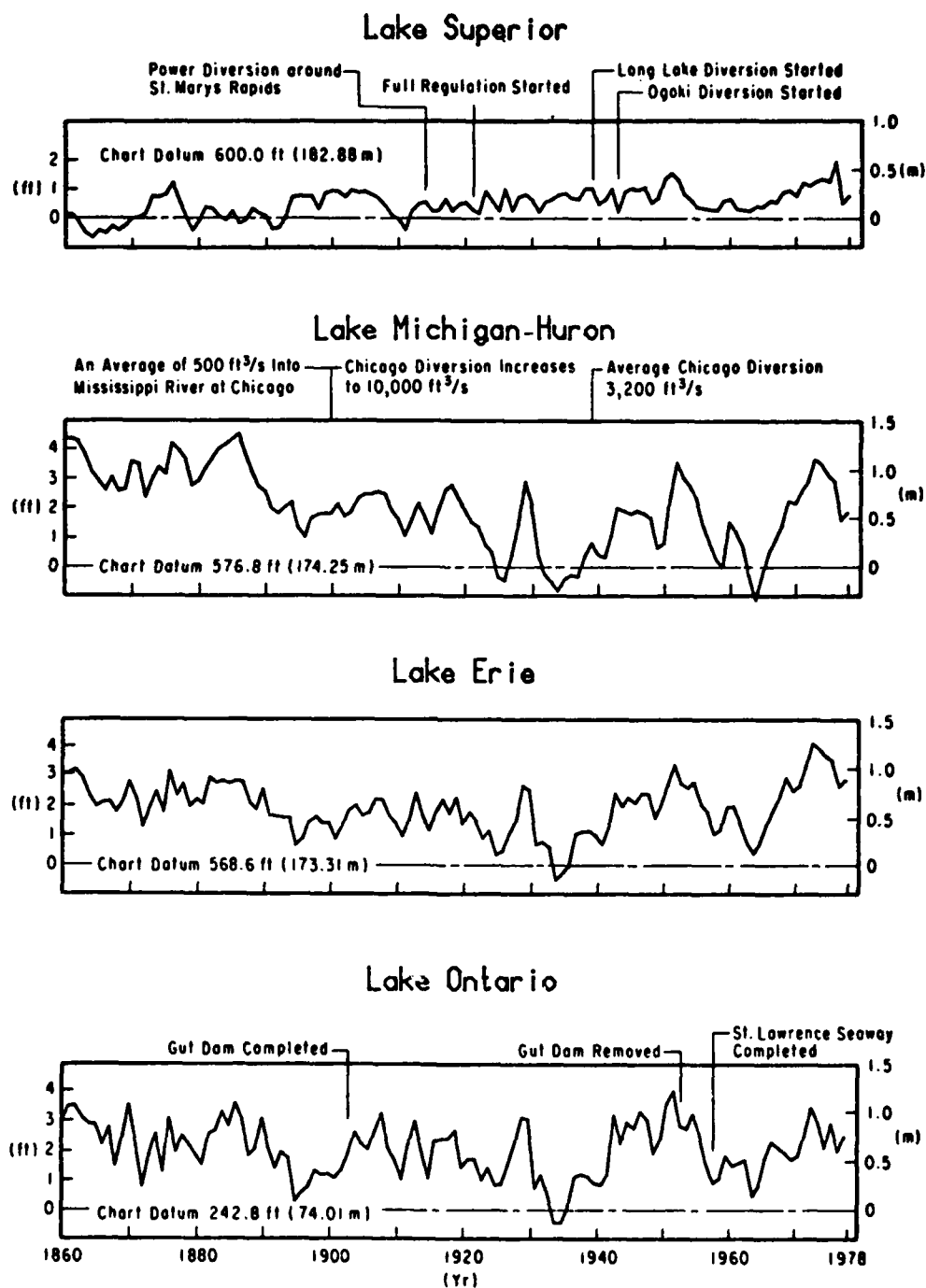
Figure 2. Historic changes in annual mean water levels on the Great Lakes, 1860 to 1978.
