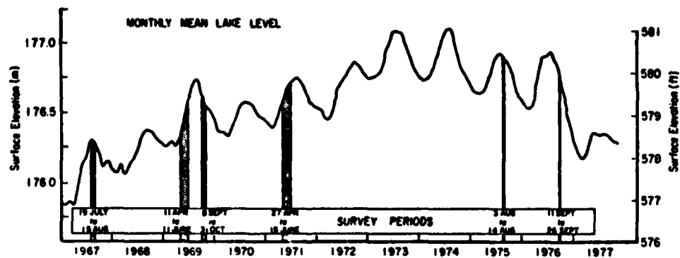
Figure 15. Lake Michigan hydrograph showing changes in lake level between survey periods.
