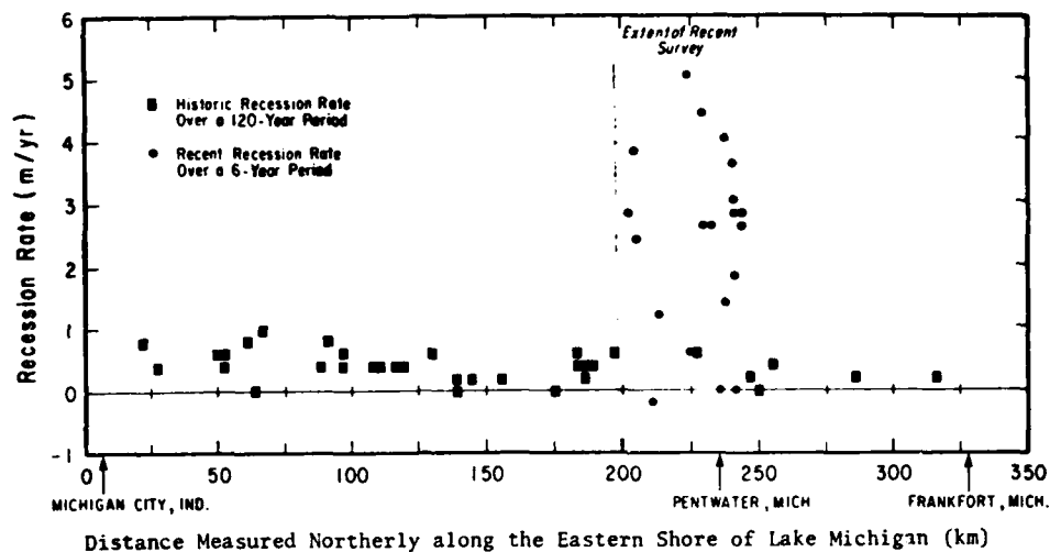
Figure 18. Comparison between rates of historic (1830's to 1959's) and recent (1969-75) recession. Positions of survey stations on the eastern shore of Lake Michigan are referenced to the Porter-La Porte County boundary in Indiana.
