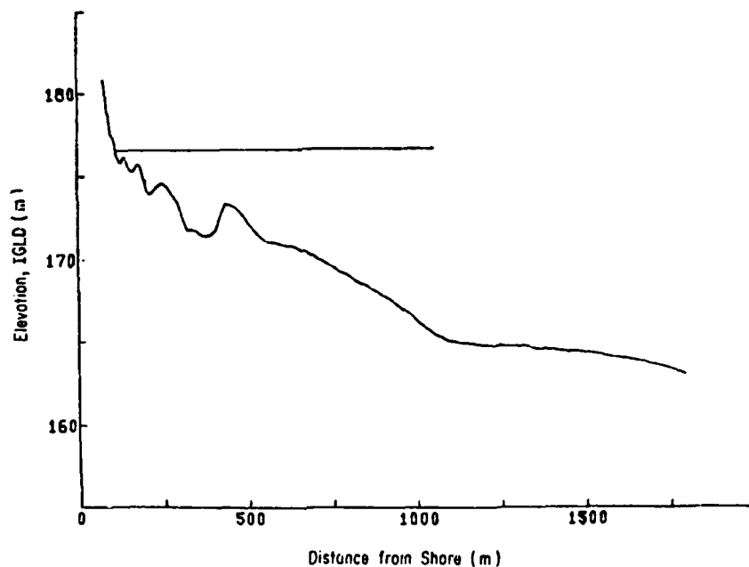
Figure A-5. A typical example of the nearshore bathymetry in the study area.
