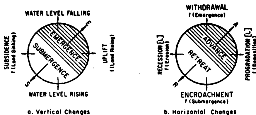
Figure 6. Terminology of vertical and horizontal shoreline changes.
