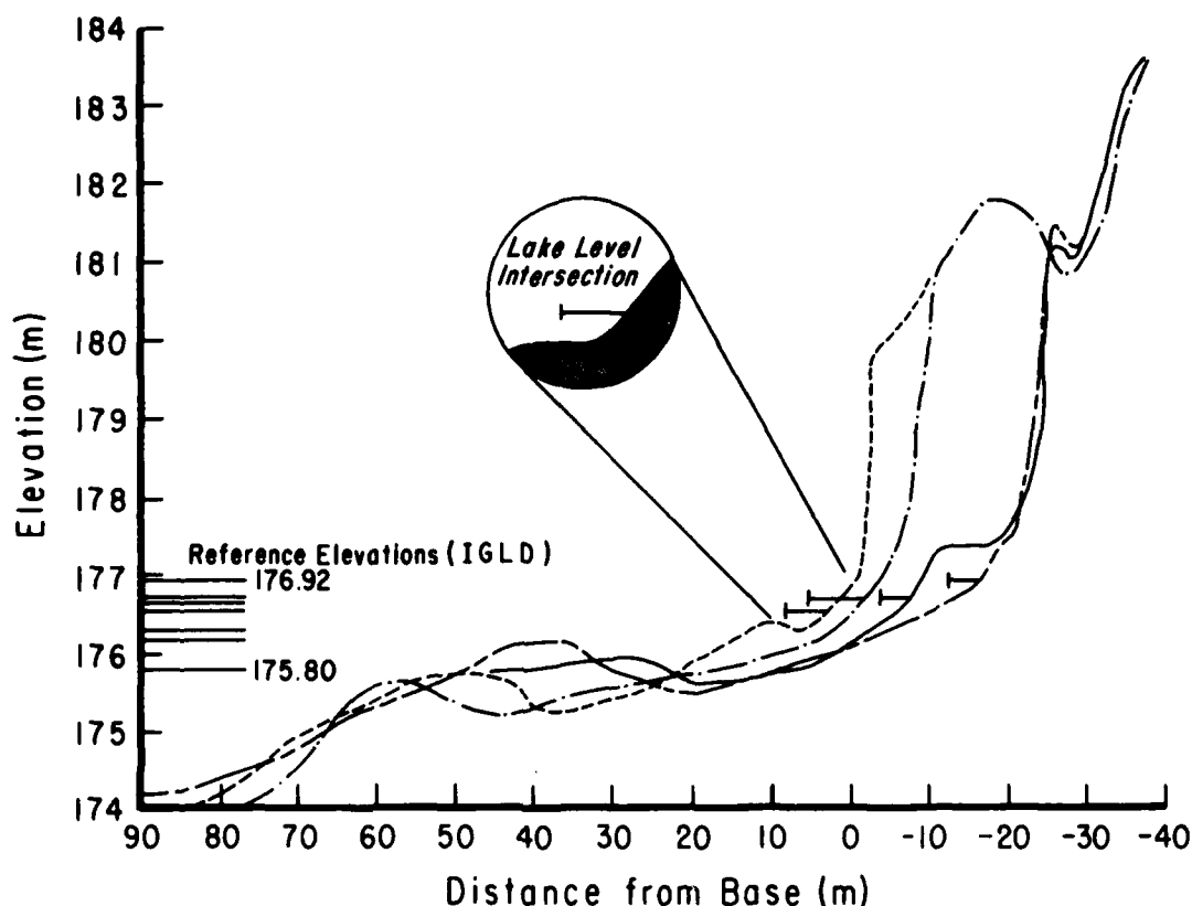
Figure 10. A fairly typical inner profile. Note the various reference elevations (International Great Lakes Datum - IGLD) at which contour migration was measured to determine rates of beach face recession plotted in Figure 9.
