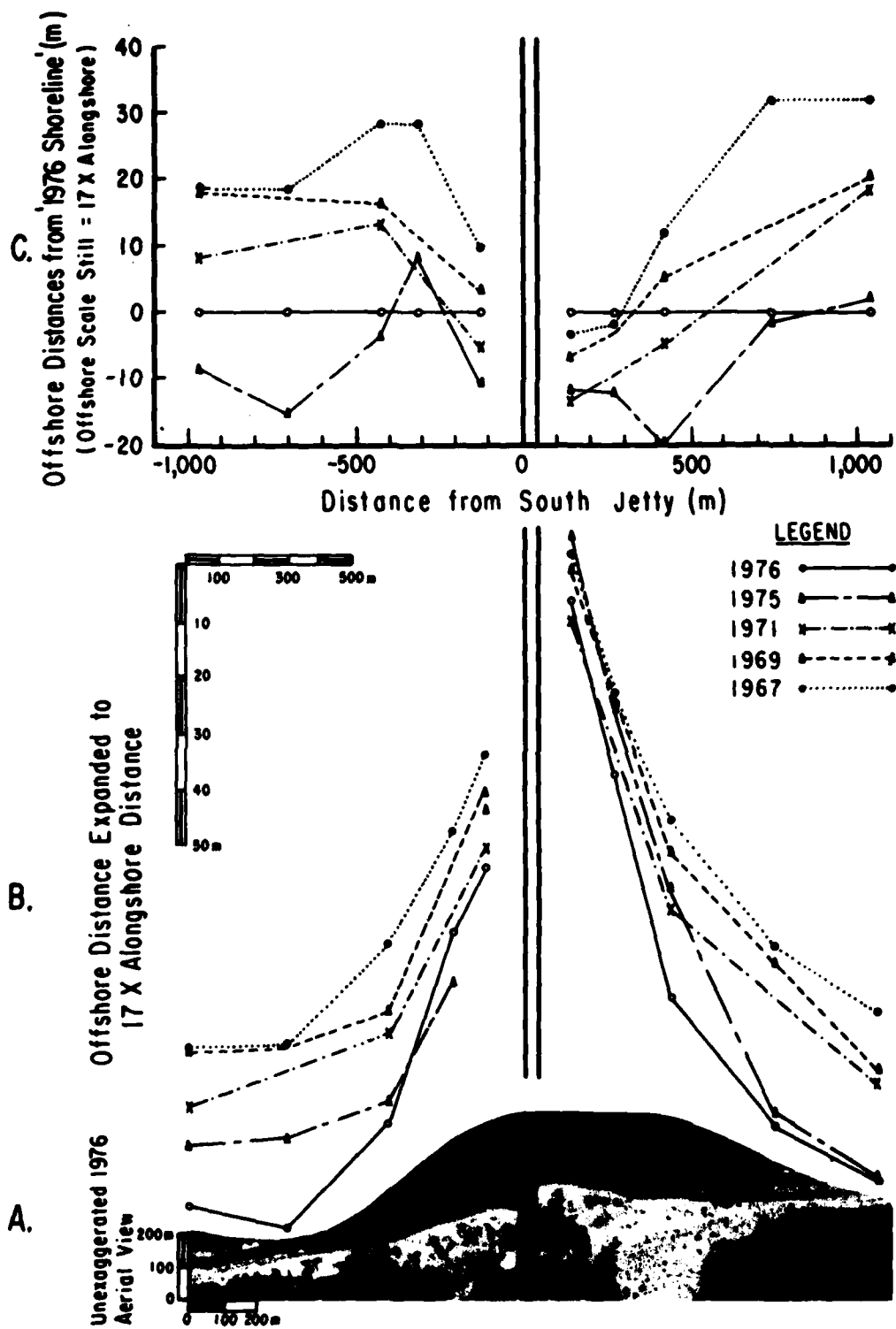
Figure 7. Different formats depicting changes in the shoreline adjacent to the Pentwater jetties. The top format (also used in Figures 8 and 9) was obtained from the unexaggerated aerial view by a two-step transformation (A to B, then B to C).
