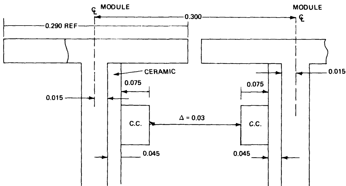
Figure 30 Pitch ISEM-2A Module
