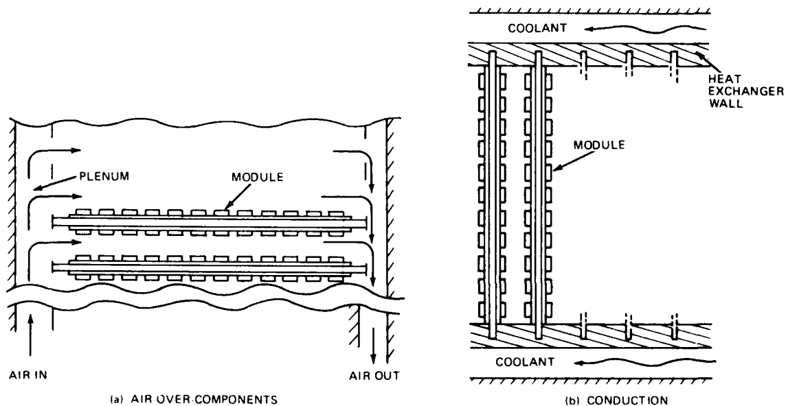
Figure 47 Typical Module Installation
