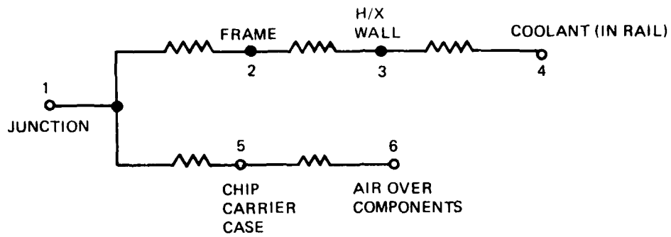
Figure 49 Resistance Network
