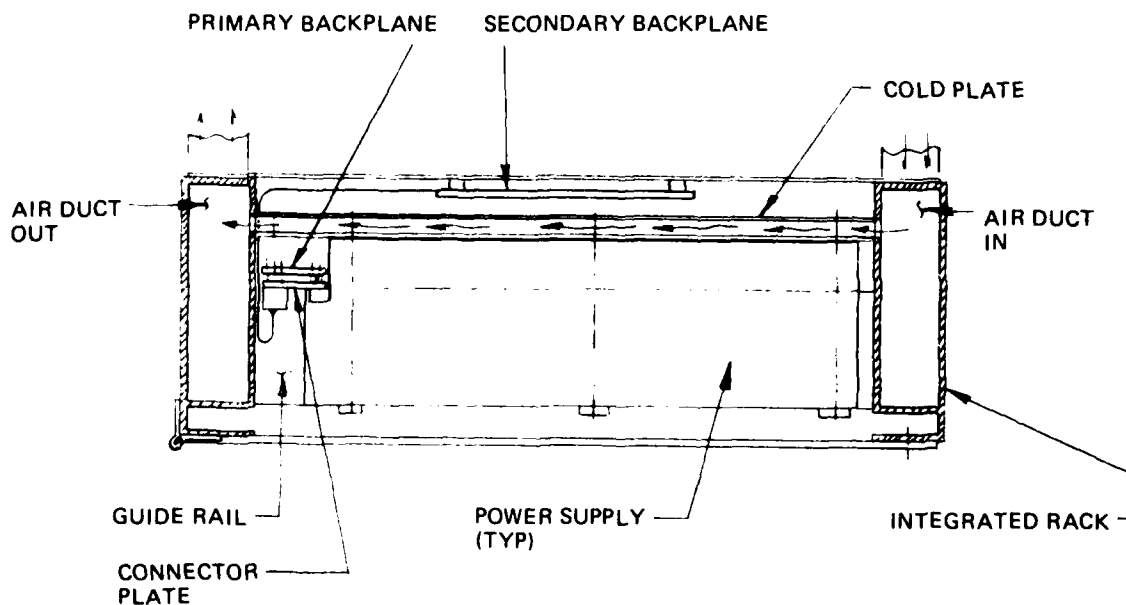
Figure 36 Power Supply Mounting (Typical)
