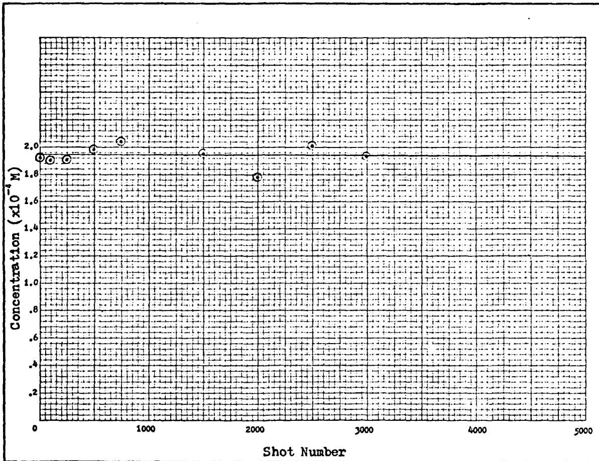
Fig. 20. Dye Concentration Versus Shot Number for Trial 4
