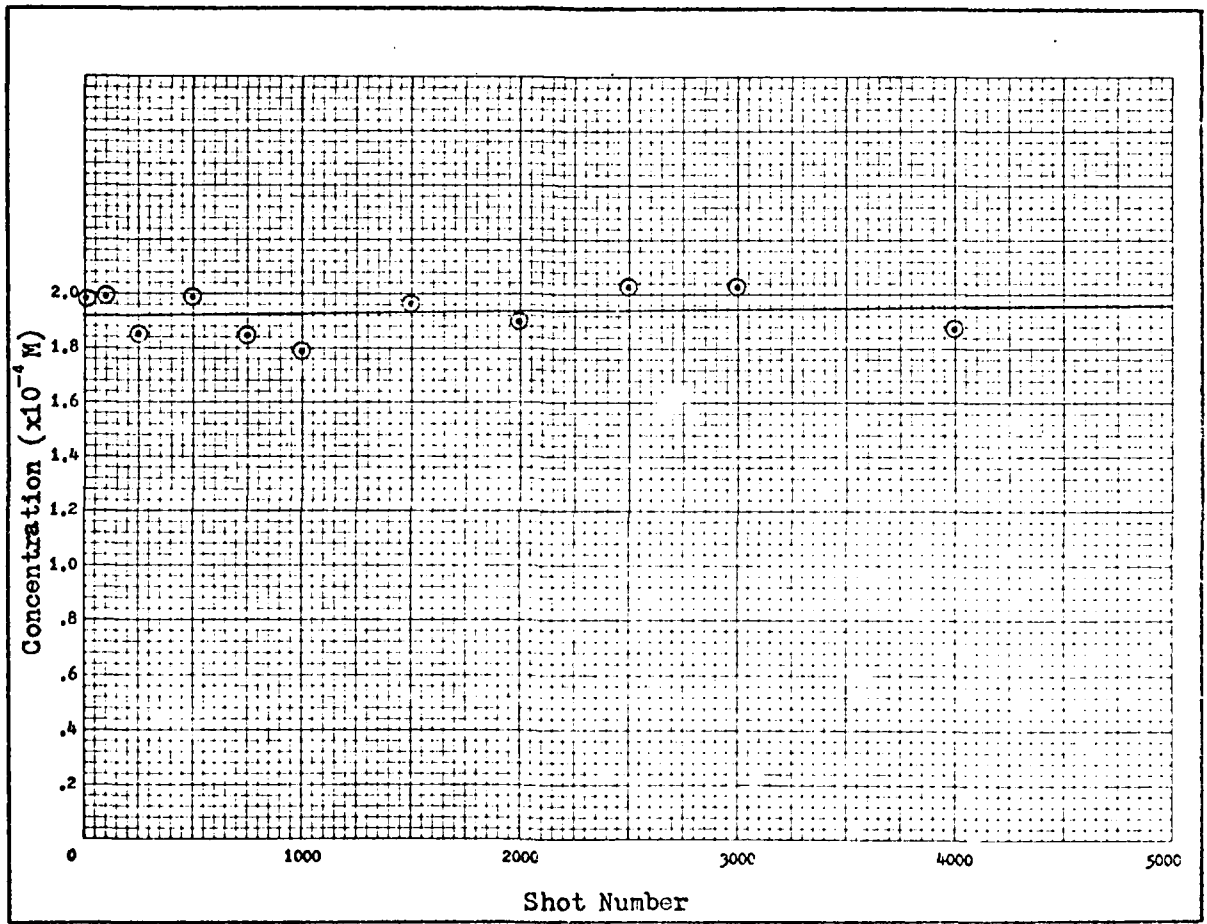
Fig. 24. Dye Concentration Versus Shot Number for Trial 6
