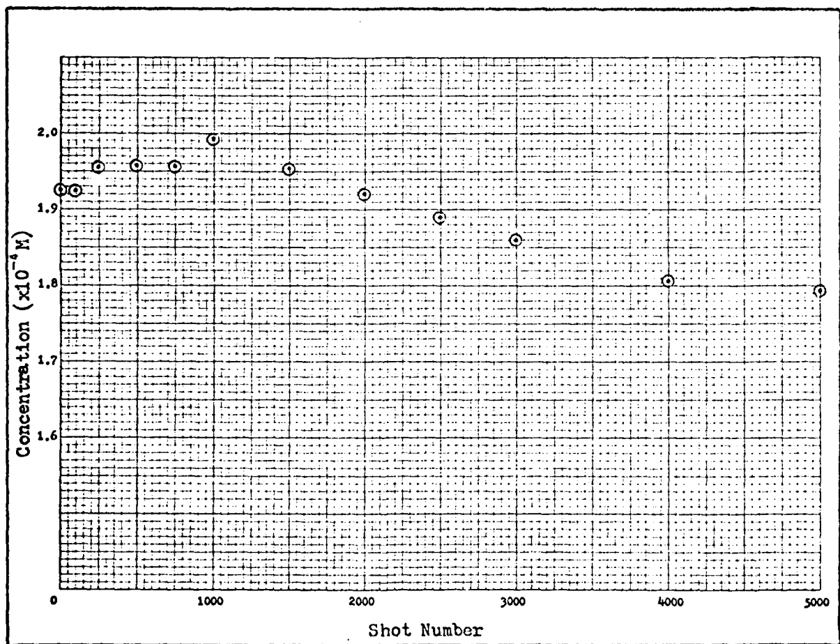
Fig. 25. UV-Determined Concentration Versus Shot Number for Trial 2
